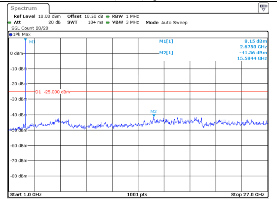
1000.0MHz-27000.0MHz Band 41 20MHz/2675.0/High 16QAM 100@0 Band 41 5MHz/2686.7/High 16QAM 25@0
