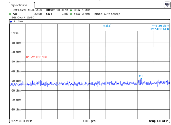
30.0MHz-1000.0MHz Band 41 20MHz/2675.0/High 16QAM 100@0 Band 41 5MHz/2686.7/High 16QAM 25@0
