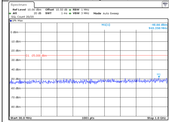
30.0MHz-1000.0MHz Band 41 20MHz/2675.0/High 16QAM 1@99 Band 41 5MHz/2686.7/High 16QAM 1@0
