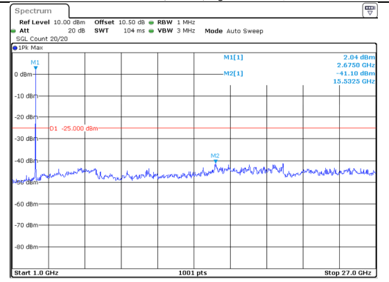
1000.0MHz-27000.0MHz Band 41 20MHz/2675.0/High 16QAM 1@99 Band 41 5MHz/2686.7/High 16QAM 1@0
