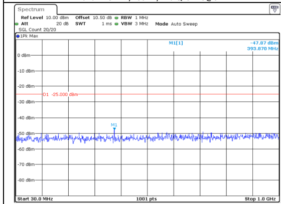
30.0MHz-1000.0MHz Band 41 20MHz/2590.5/Mid QPSK 100@0 Band 41 5MHz/2602.2/Mid QPSK 25@0
