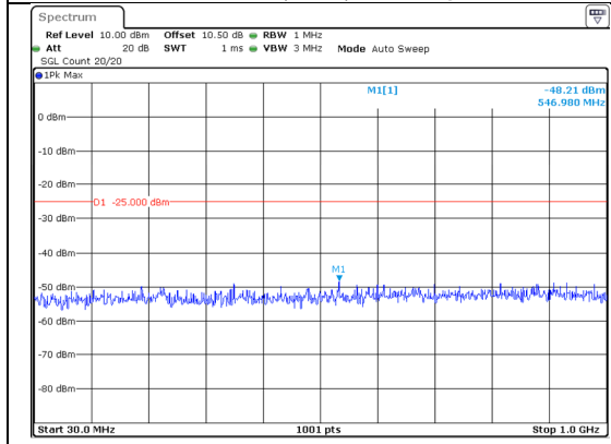
30.0MHz-1000.0MHz Band 41 20MHz/2590.5/Mid QPSK 1@99 Band 41 5MHz/2602.2/Mid QPSK 1@0
