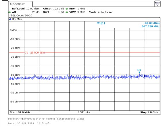
30.0MHz-1000.0MHz Band 41 5MHz/2499.3/Low 64QAM 1@24 Band 41 20MHz/2511.0/Low 64QAM 1@0
