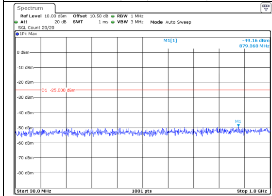
30.0MHz-1000.0MHz Band 41 20MHz/2506.0/Low 64QAM 100@0 Band 41 5MHz/2517.7/Low 64QAM 25@0
