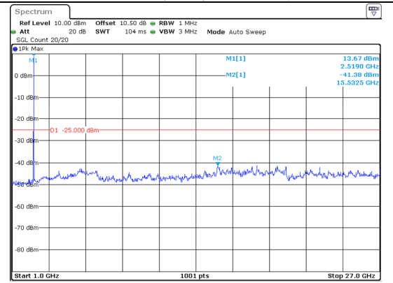
1000.0MHz-27000.0MHz Band 41 20MHz/2506.0/Low 64QAM 100@0 Band 41 5MHz/2517.7/Low 64QAM 25@0
