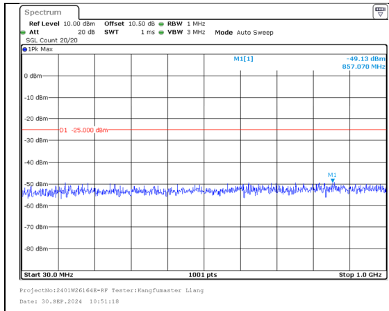
30.0MHz-1000.0MHz Band 41 5MHz/2499.3/Low 16QAM 25@0 Band 41 20MHz/2511.0/Low 16QAM 100@0
