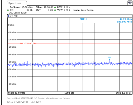
30.0MHz-1000.0MHz Band 41 5MHz/2499.3/Low 64QAM 25@0 Band 41 20MHz/2511.0/Low 64QAM 100@0
