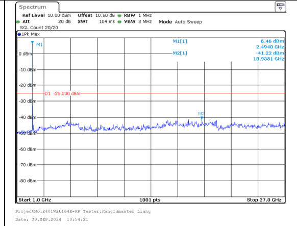
1000.0MHz-27000.0MHz Band 41 5MHz/2499.3/Low 64QAM 25@0 Band 41 20MHz/2511.0/Low 64QAM 100@0
