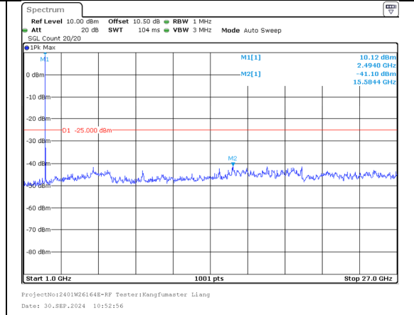
1000.0MHz-27000.0MHz Band 41 5MHz/2499.3/Low 64QAM 1@24 Band 41 20MHz/2511.0/Low 64QAM 1@0
