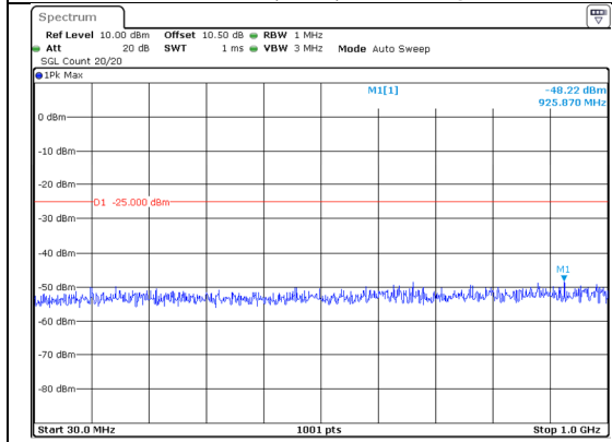
30.0MHz-1000.0MHz Band 41 20MHz/2506.0/Low 64QAM 1@99 Band 41 5MHz/2517.7/Low 64QAM 1@0
