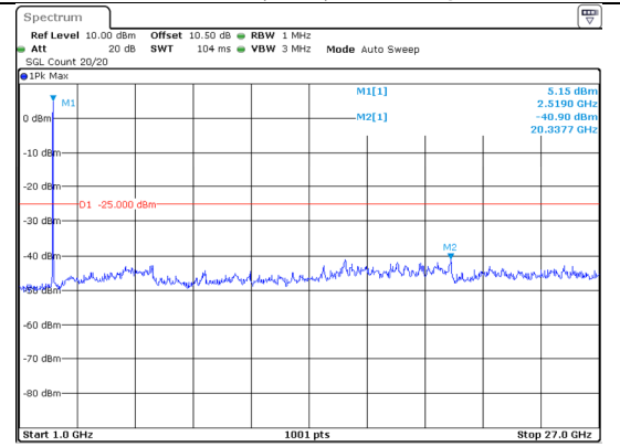
1000.0MHz-27000.0MHz Band 41 20MHz/2506.0/Low 64QAM 1@99 Band 41 5MHz/2517.7/Low 64QAM 1@0
