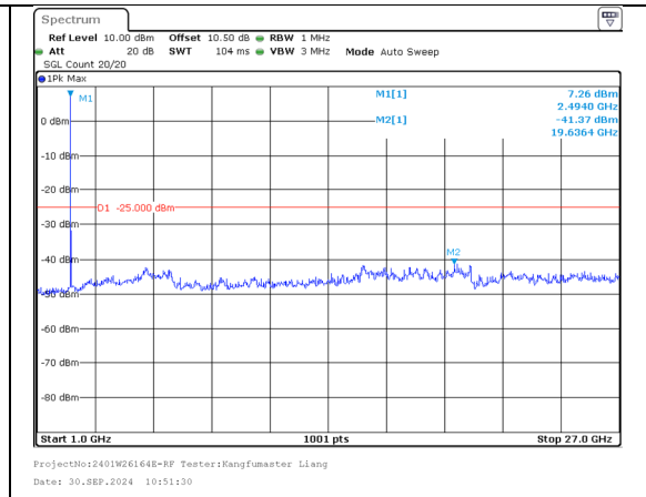
1000.0MHz-27000.0MHz Band 41 5MHz/2499.3/Low 16QAM 25@0 Band 41 20MHz/2511.0/Low 16QAM 100@0
