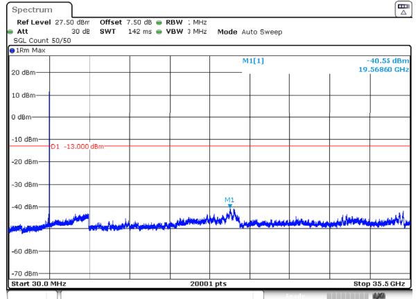
n78_1_100MHz_30kHz_3500MHz_DFT-s-OFDM QPSK_RB1@272 -40.55dBm
