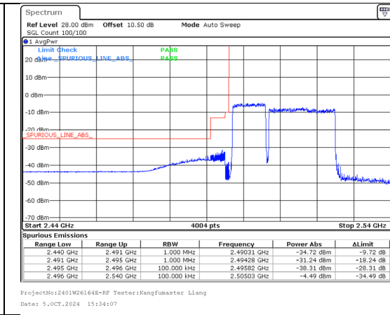
Band 41 10MHz/2501.5/Low QPSK 50@0 Band 41 20MHz/2515.9/Low QPSK 100@0
