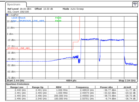
Band 41 15MHz/2503.8/Low 256QAM 75@0 Band 41 20MHz/2520.9/Low 256QAM 100@0
