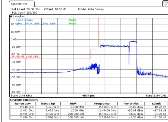
Band 41 5MHz/2499.3/Low 256QAM 25@0 Band 41 20MHz/2511.0/Low 256QAM 100@0
