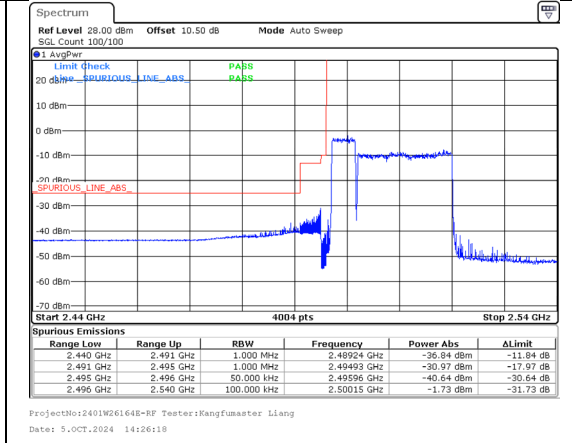
Band 41 5MHz/2499.3/Low 16QAM 25@0 Band 41 20MHz/2511.0/Low 16QAM 100@0
