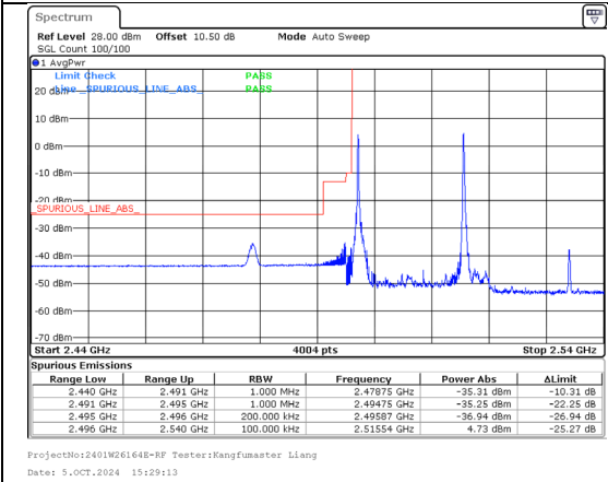
Band 41 20MHz/2506.0/Low 256QAM 1@0 Band 41 5MHz/2517.7/Low 256QAM 1@0
