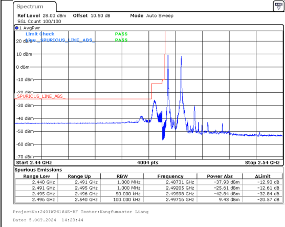
Band 41 5MHz/2499.3/Low 16QAM 1@0 Band 41 20MHz/2511.0/Low 16QAM 1@0
