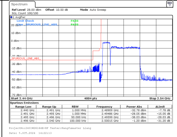
Band 41 5MHz/2499.3/Low QPSK 25@0 Band 41 20MHz/2511.0/Low QPSK 100@0
