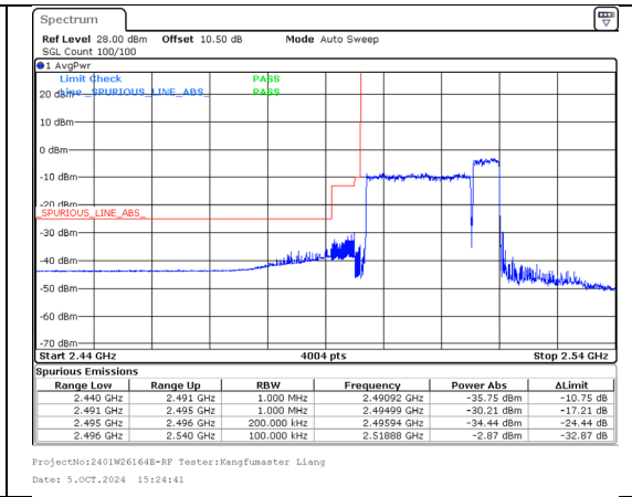
Band 41 20MHz/2506.0/Low 16QAM 100@0 Band 41 5MHz/2517.7/Low 16QAM 25@0
