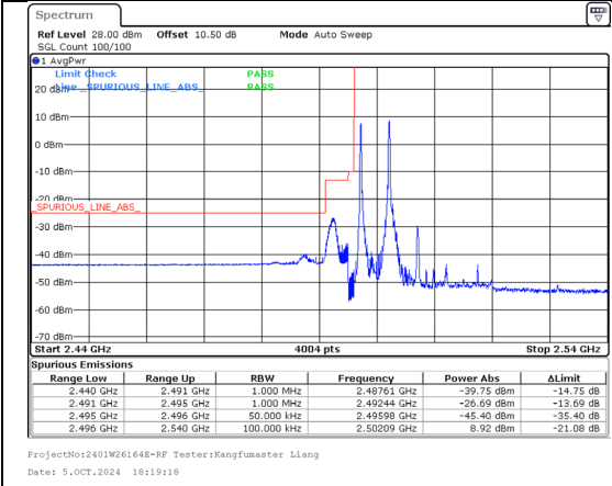
Band 41 5MHz/2499.3/Low QPSK 1@0 Band 41 20MHz/2511.0/Low QPSK 1@0
