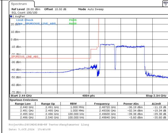
Band 41 10MHz/2501.5/Low 64QAM 50@0 Band 41 20MHz/2515.9/Low 64QAM 100@0
