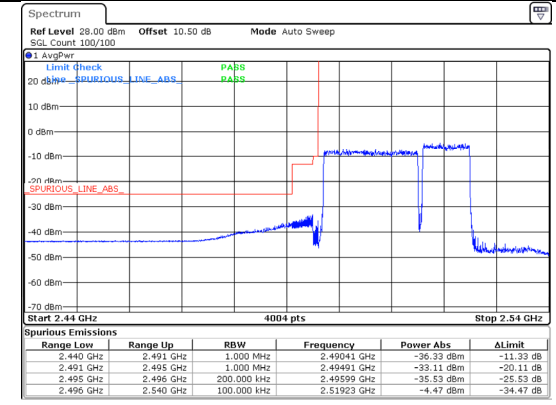
Band 41 10MHz/2501.5/Low 256QAM 50@0 Band 41 20MHz/2515.9/Low 256QAM 100@0
