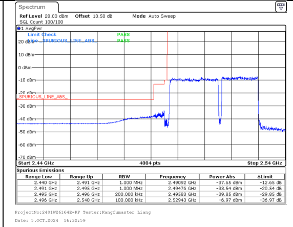
Band 41 20MHz/2506.0/Low 256QAM 100@0 Band 41 15MHz/2523.1/Low 256QAM 75@0
