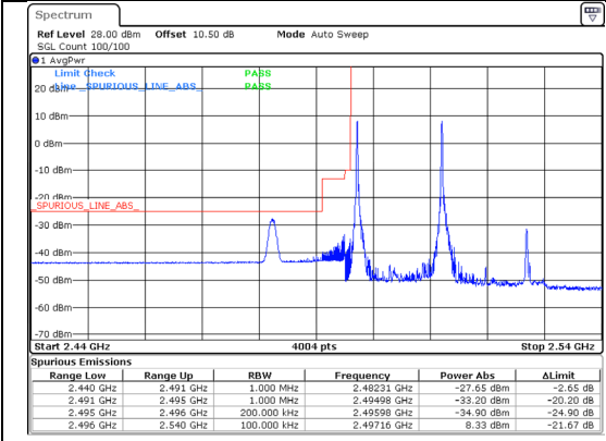
Band 41 15MHz/2503.8/Low QPSK 1@0 Band 41 20MHz/2520.9/Low QPSK 1@0
