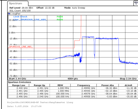
Band 41 10MHz/2501.5/Low 16QAM 50@0 Band 41 20MHz/2515.9/Low 16QAM 100@0
