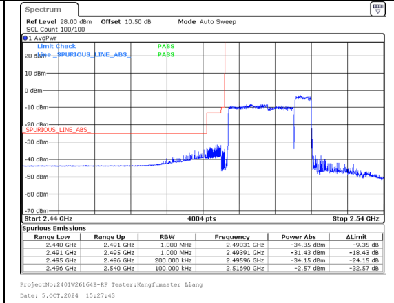
Band 41 20MHz/2506.0/Low 64QAM 100@0 Band 41 5MHz/2517.7/Low 64QAM 25@0
