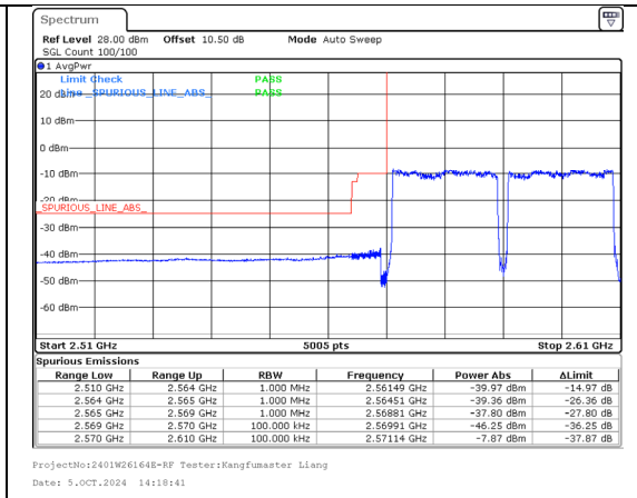
Band 38 20MHz/2580.0/Low 256QAM 100@0 Band 38 20MHz/2599.8/Low 256QAM 100@0
