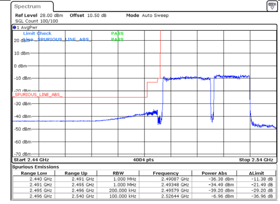
Band 41 20MHz/2506.0/Low QPSK 100@0 Band 41 15MHz/2523.1/Low QPSK 75@0
