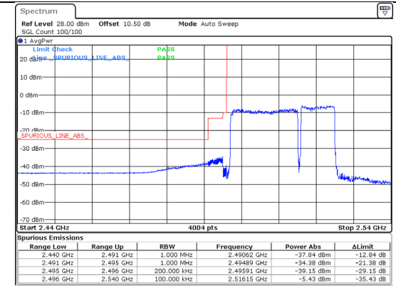
Band 41 20MHz/2506.0/Low QPSK 100@0 Band 41 10MHz/2520.4/Low QPSK 50@0
