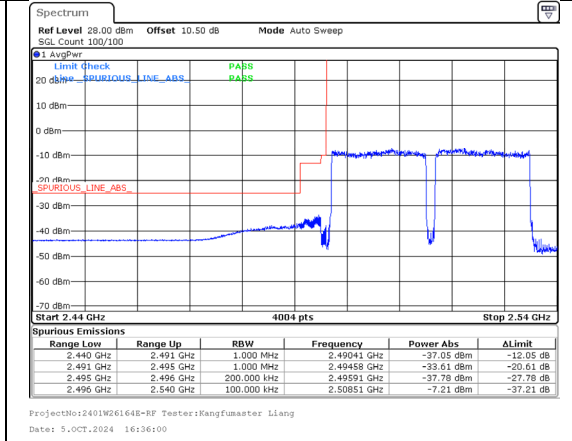
Band 41 20MHz/2506.0/Low QPSK 100@0 Band 41 20MHz/2525.8/Low QPSK 100@0
