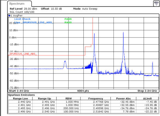
Band 41 20MHz/2506.0/Low QPSK 1@0 Band 41 15MHz/2523.1/Low QPSK 1@0
