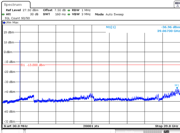
n77_3_15MHz_30kHz_3840MHz_DFT-s-OFDM QPSK_RB1@37 -36.96dBm
