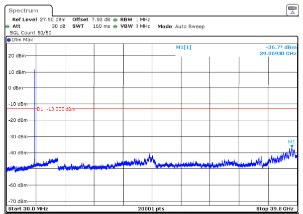
n77_3_30MHz_30kHz_3840MHz_DFT-s-OFDM QPSK_RB1@0 -36.77dBm
