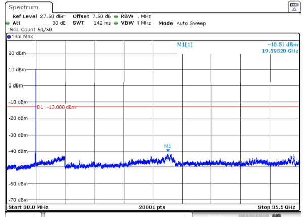
n77_1_80MHz_30kHz_3490MHz_DFT-s-OFDM QPSK_RB1@216 -40.51dBm
