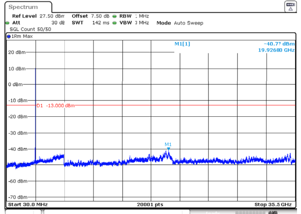
n77_1_80MHz_30kHz_3510MHz_DFT-s-OFDM QPSK_RB1@216 -40.77dBm
