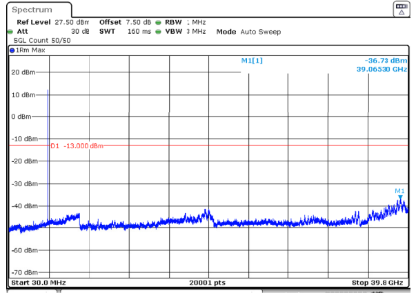
n77_3_10MHz_30kHz_3840MHz_DFT-s-OFDM QPSK_RB1@23 -36.73dBm
