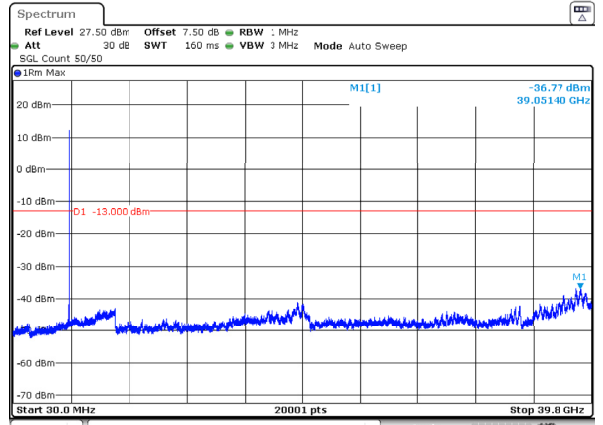
n77_3_20MHz_30kHz_3840MHz_DFT-s-OFDM QPSK_RB1@50 -36.77dBm
