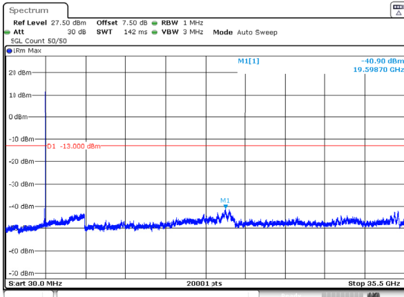
n77_1_90MHz_30kHz_3505MHz_DFT-s-OFDM QPSK_RB1@244 -40.90dBm
