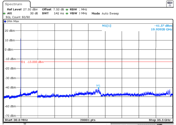
n77_1_100MHz_30kHz_3500MHz_DFT-s-OFDM QPSK_RB1@272 -41.57dBm
