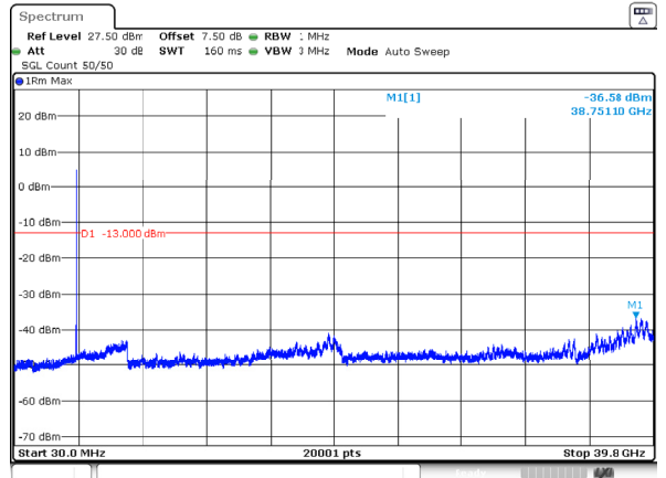
n77_3_15MHz_30kHz_3840MHz_DFT-s-OFDM QPSK_RB36@0 -36.58dBm
