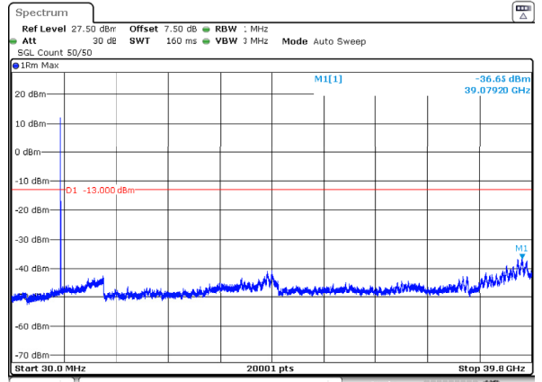
n77_3_30MHz_30kHz_3715MHz_DFT-s-OFDM QPSK_RB1@77 -36.65dBm
