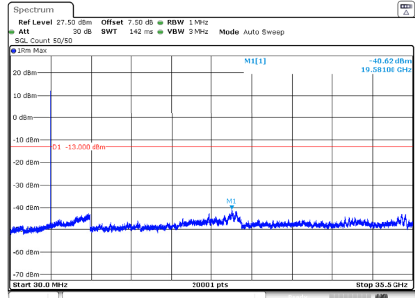
n77_1_10MHz_30kHz_3545MHz_DFT-s-OFDM QPSK_RB1@23 -40.62dBm
