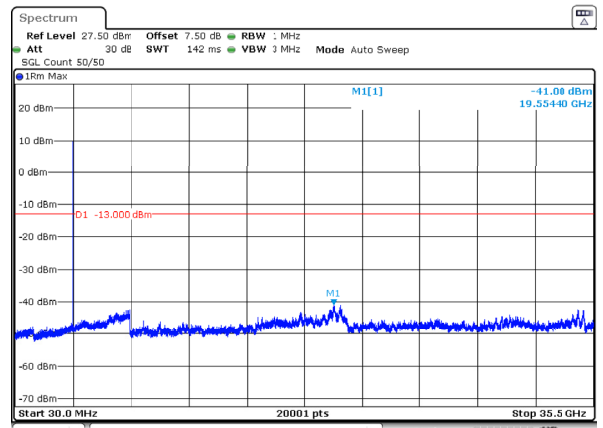
n77_1_15MHz_30kHz_3542.5MHz_DFT-s-OFDM QPSK_RB1@0 -41dBm
