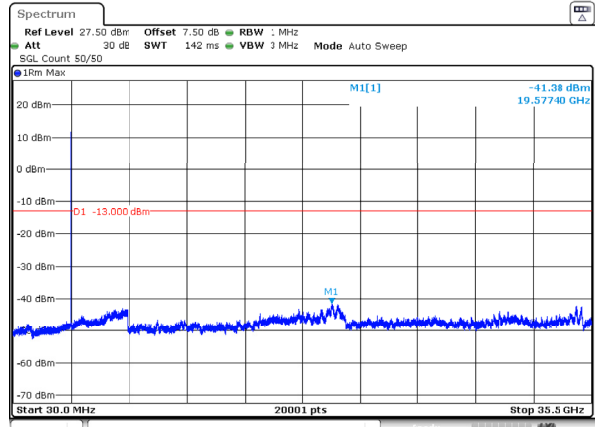
n77_1_20MHz_30kHz_3540MHz_DFT-s-OFDM QPSK_RB1@50 -41.38dBm
