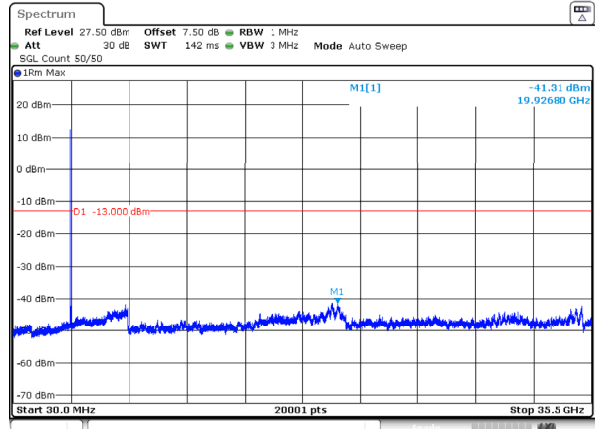
n77_1_50MHz_30kHz_3500MHz_DFT-s-OFDM QPSK_RB1@0 -41.31dBm
