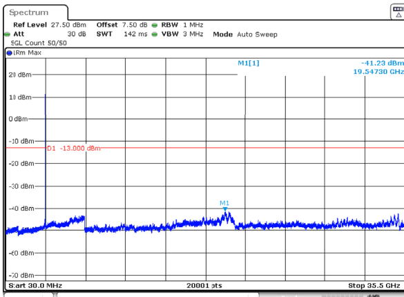
n77_1_60MHz_30kHz_3520MHz_DFT-s-OFDM QPSK_RB1@161 -41.23dBm
