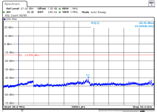
n77_1_50MHz_30kHz_3525MHz_DFT-s-OFDM QPSK_RB1@132 -40.53dBm
