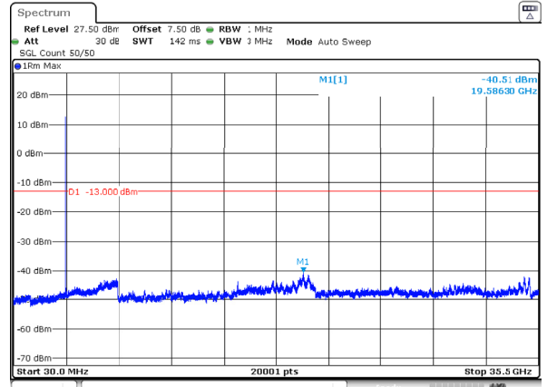
n77_1_15MHz_30kHz_3500MHz_DFT-s-OFDM QPSK_RB1@37 -40.51dBm
