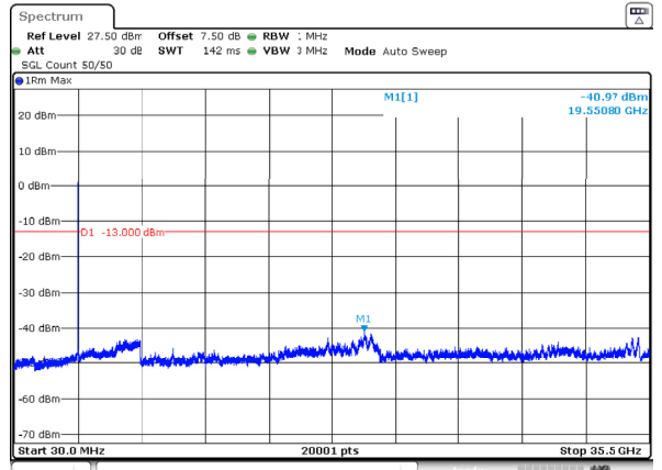
n77_1_30MHz_30kHz_3535MHz_DFT-s-OFDM QPSK_RB75@0 -40.97dBm
