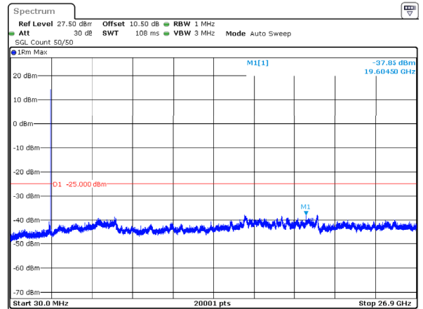
n41_100MHz_30kHz_2592.99MHz_DFT-s-OFDM QPSK_RB1@272 -37.85dBm
