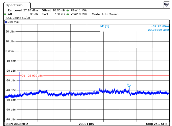
n41_50MHz_30kHz_2521.02MHz_DFT-s-OFDM QPSK_RB128@0 -37.73dBm
