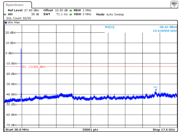
n66_30MHz_15kHz_1725MHz_DFT-s-OFDM QPSK_RB160@0 -36.67dBm
