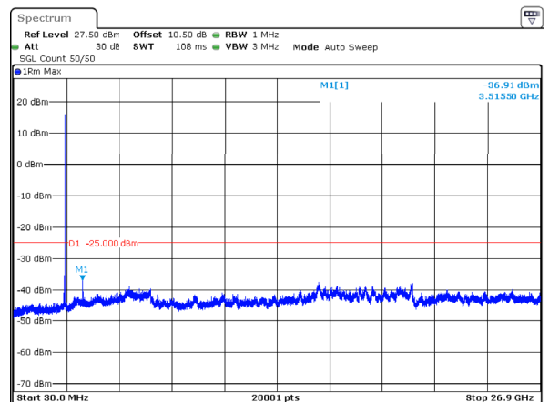
n41_40MHz_30kHz_2592.99MHz_DFT-s-OFDM QPSK_RB1@105 -36.91dBm
