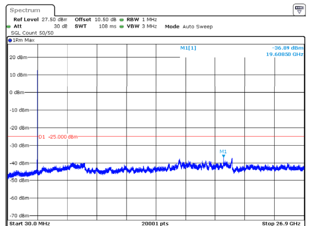
n41_50MHz_30kHz_2664.99MHz_DFT-s-OFDM QPSK_RB1@132 -36.89dBm
