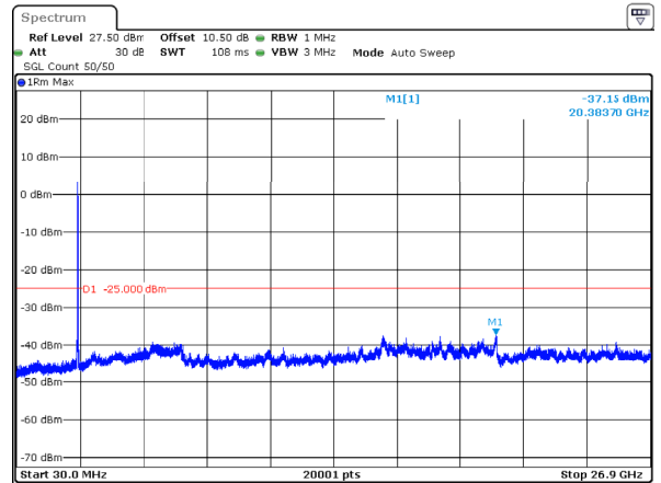
n41_40MHz_30kHz_2592.99MHz_DFT-s-OFDM QPSK_RB100@0 -37.15dBm
