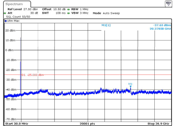
n41_15MHz_30kHz_2592.99MHz_DFT-s-OFDM QPSK_RB1@37 -37.63dBm
