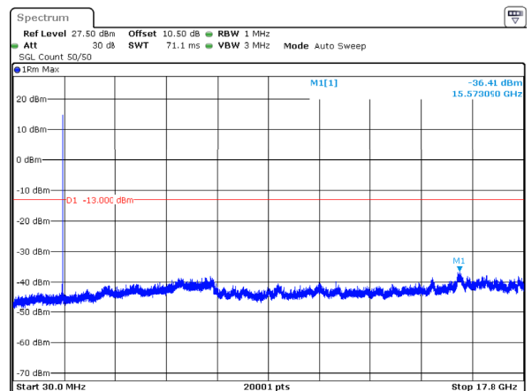
n66_30MHz_15kHz_1725MHz_DFT-s-OFDM QPSK_RB1@159 -36.41dBm
