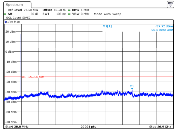
n41_20MHz_30kHz_2506.02MHz_DFT-s-OFDM QPSK_RB1@50 -37.72dBm
