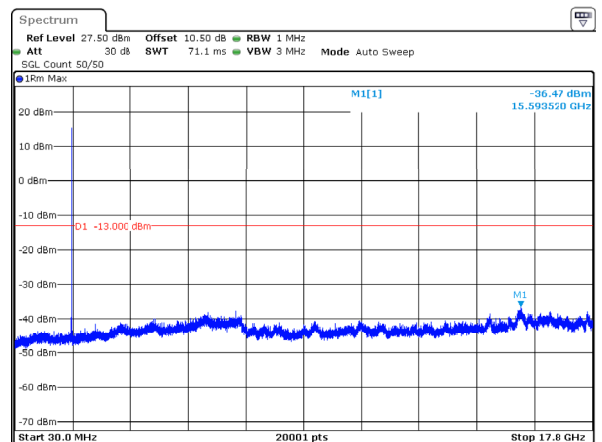
n66_25MHz_15kHz_1745MHz_DFT-s-OFDM QPSK_RB1@132 -36.47dBm
