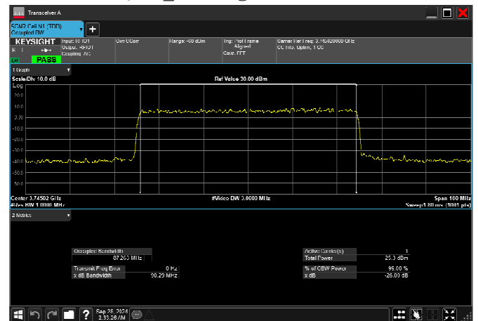
n78_3_90MHz_30kHz_3745MHz_CP-OFDM 256 QAM_RB245@0 87.263MHz
