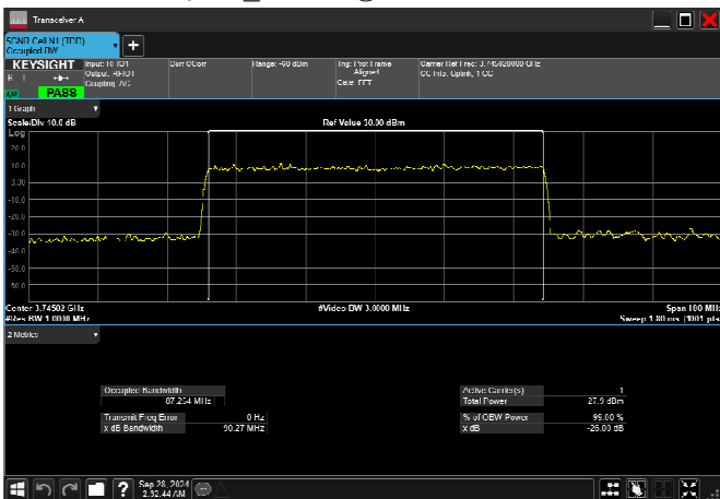
n78_3_90MHz_30kHz_3745MHz_CP-OFDM 64 QAM_RB245@0 87.264MHz
