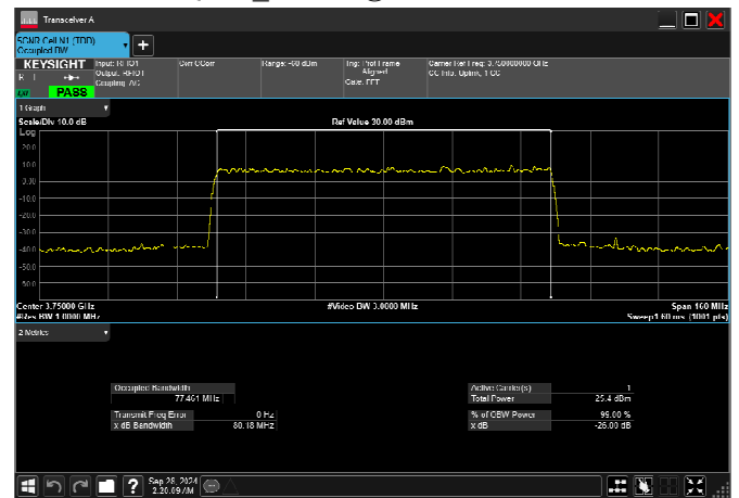
n78_3_80MHz_30kHz_3750MHz_CP-OFDM 256 QAM_RB217@0 77.461MHz
