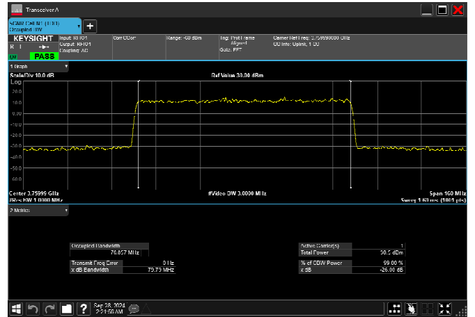
n78_3_80MHz_30kHz_3760MHz_DFT-s-OFDM 64 QAM_RB216@0 76.956MHz
