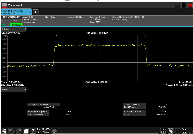
n78_3_90MHz_30kHz_3750MHz_DFT-s-OFDM 256 QAM_RB243@0 86.425MHz
