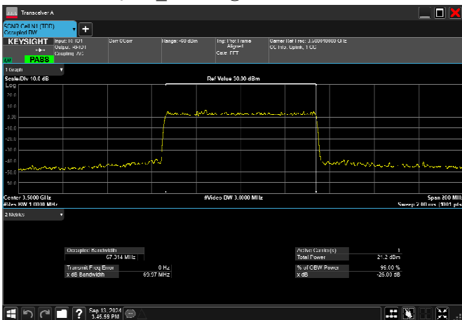
n78_1_70MHz_30kHz_3500MHz_CP-OFDM 64 QAM_RB189@0 67.314MHz
