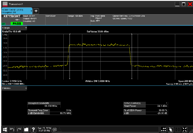
n78_1_70MHz_30kHz_3515MHz_DFT-s-OFDM 16 QAM_RB180@0 66.544MHz
