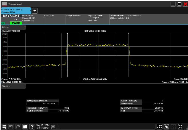
n78_1_70MHz_30kHz_3515MHz_CP-OFDM 256 QAM_RB189@0 67.349MHz
