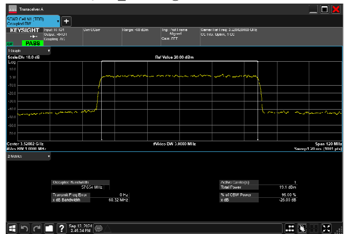
n78_1_60MHz_30kHz_3520MHz_CP-OFDM 256 QAM_RB162@0 57.654MHz
