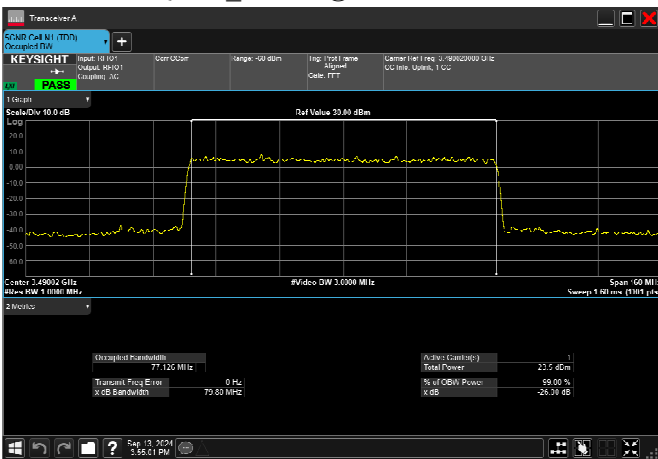
n78_1_80MHz_30kHz_3490MHz_DFT-s-OFDM QPSK_RB216@0 77.126MHz
