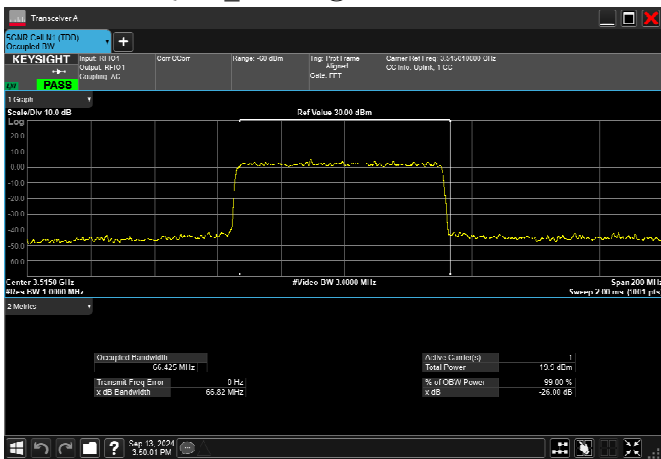
n78_1_70MHz_30kHz_3515MHz_DFT-s-OFDM 256 QAM_RB180@0 66.425MHz
