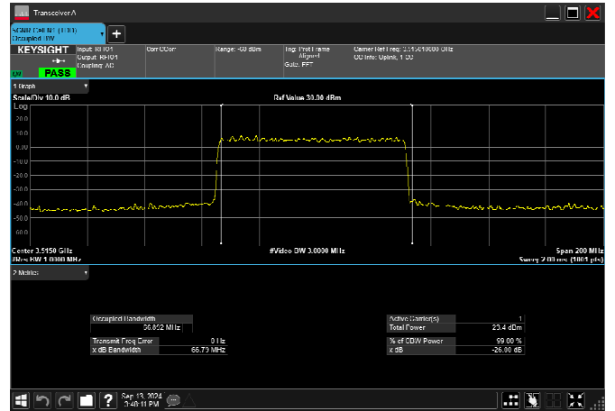
n78_1_70MHz_30kHz_3515MHz_DFT-s-OFDM 64 QAM_RB180@0 66.816MHz
