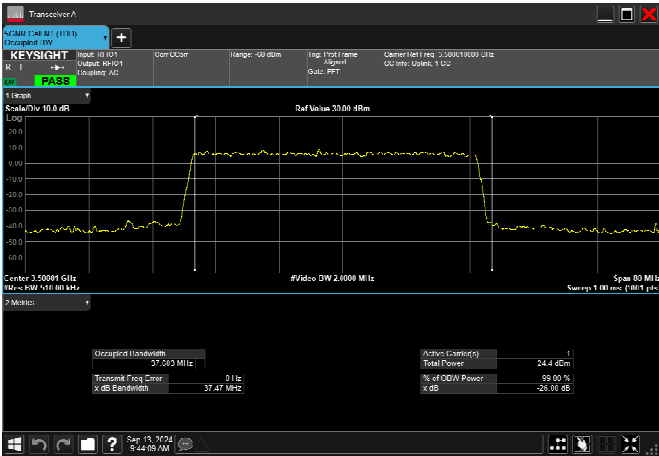
n78_1_40MHz_30kHz_3500MHz_DFT-s-OFDM 16 QAM_RB100@0 37.445MHz
