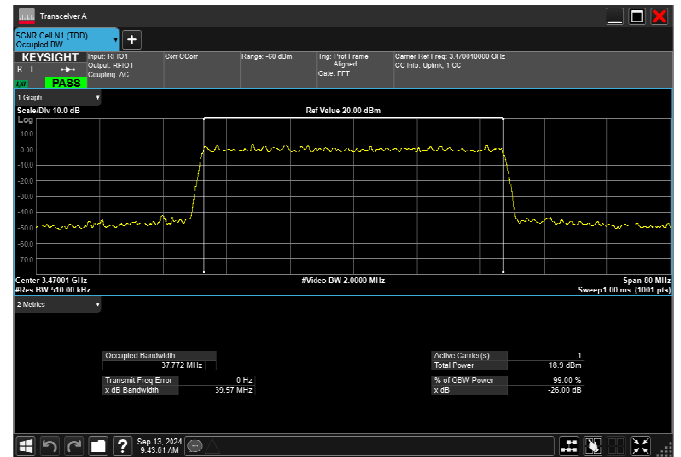
n78_1_40MHz_30kHz_3470MHz_CP-OFDM 256 QAM_RB106@0 37.772MHz
