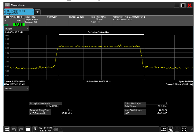
n78_1_40MHz_30kHz_3530MHz_DFT-s-OFDM 16 QAM_RB100@0 37.343MHz
