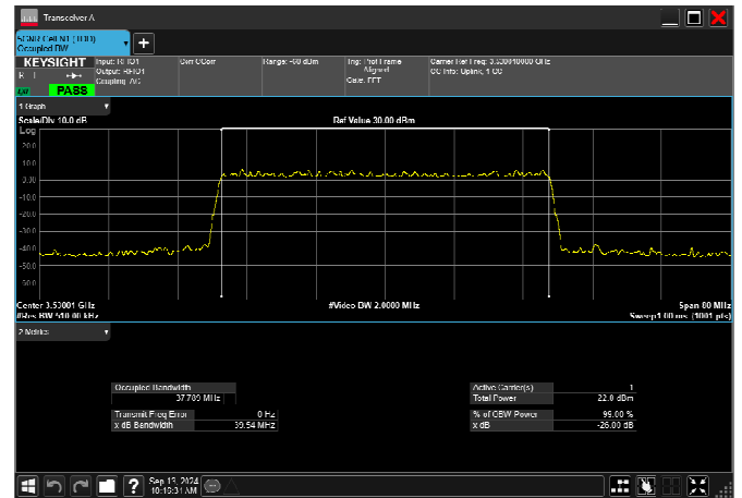
n78_1_40MHz_30kHz_3530MHz_CP-OFDM 256 QAM_RB106@0 37.794MHz
