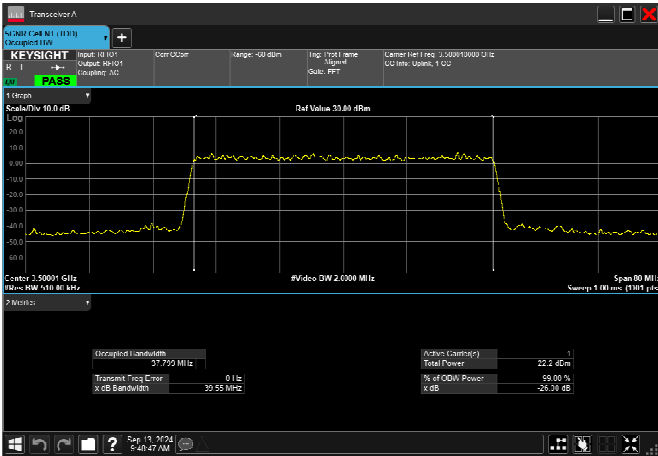
n78_1_40MHz_30kHz_3500MHz_CP-OFDM 256 QAM_RB106@0 37.784MHz
