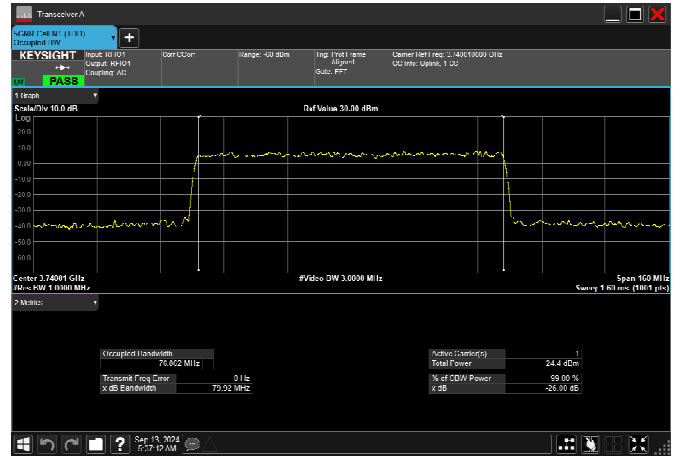
n77_3_80MHz_30kHz_3740MHz_DFT-s-OFDM 64 QAM_RB216@0 76.955MHz
