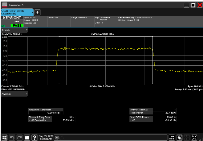
n77_3_80MHz_30kHz_3740MHz_DFT-s-OFDM 256 QAM_RB216@0 76.837MHz
