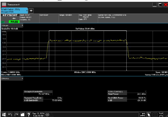
n77_3_80MHz_30kHz_3840MHz_DFT-s-OFDM QPSK_RB216@0 76.947MHz
