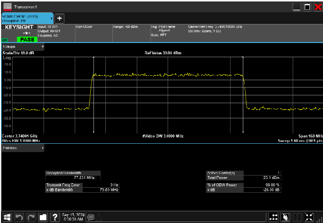
n77_3_80MHz_30kHz_3740MHz_DFT-s-OFDM 16 QAM_RB216@0 76.880MHz
