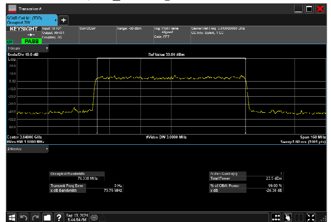
n77_3_80MHz_30kHz_3840MHz_DFT-s-OFDM 16 QAM_RB216@0 76.938MHz
