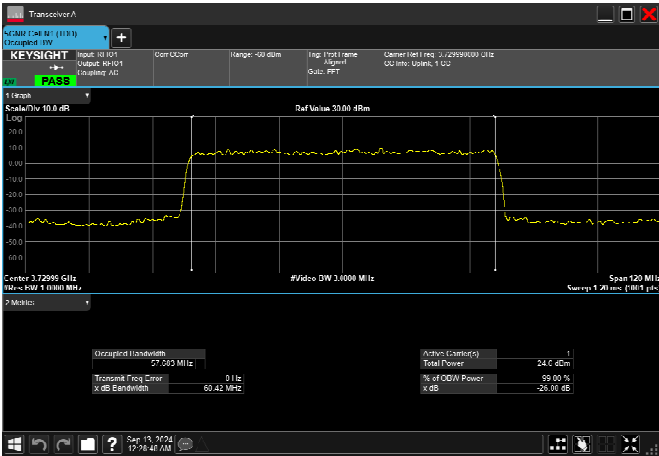
n77_3_60MHz_30kHz_3730MHz_DFT-s-OFDM 16 QAM_RB162@0 57.687MHz
