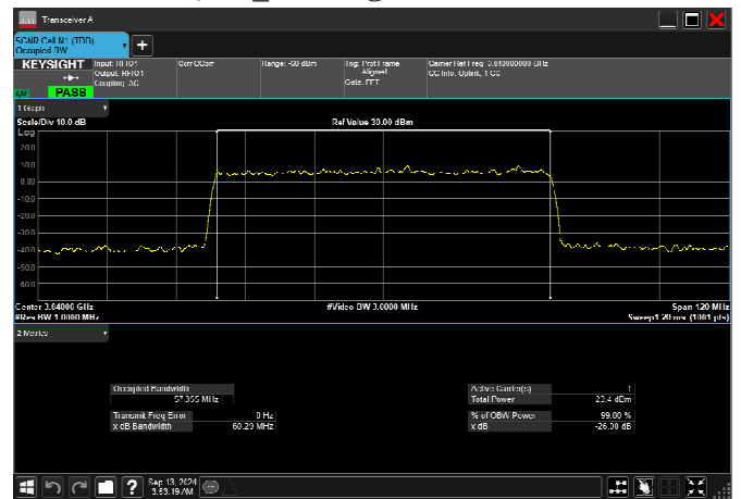
n77_3_60MHz_30kHz_3840MHz_DFT-s-OFDM 16 QAM_RB162@0 57.855MHz
