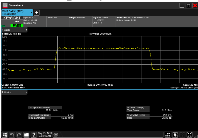
n77_3_60MHz_30kHz_3840MHz_CP-OFDM 64 QAM_RB162@0 57.712MHz
