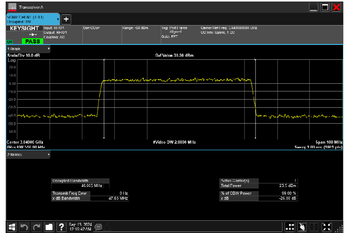
n77_3_50MHz_30kHz_3840MHz_DFT-s-OFDM 64 QAM_RB128@0 46.868MHz
