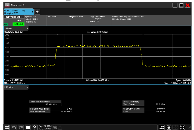
n77_3_50MHz_30kHz_3955MHz_DFT-s-OFDM 16 QAM_RB128@0 46.894MHz
