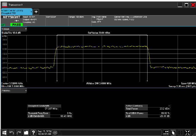
n77_3_60MHz_30kHz_3730MHz_DFT-s-OFDM 256 QAM_RB162@0 57.607MHz
