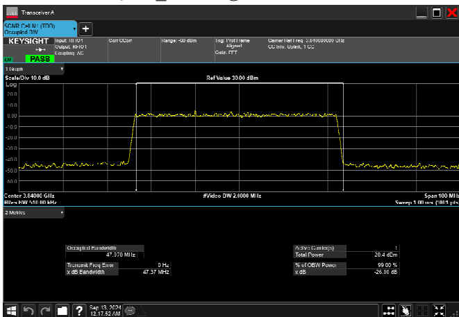
n77_3_50MHz_30kHz_3840MHz_DFT-s-OFDM 256 QAM_RB128@0 47.070MHz
