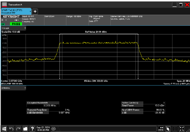
n77_3_10MHz_30kHz_3975MHz_DFT-s-OFDM 256 QAM_RB24@0 8.540MHz
