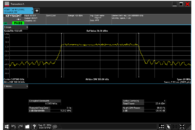
n77_3_10MHz_30kHz_3975MHz_DFT-s-OFDM 64 QAM_RB24@0 8.538MHz
