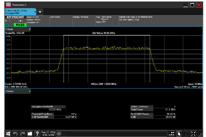
n77_3_15MHz_30kHz_3707.5MHz_CP-OFDM 256 QAM_RB38@0 13.529MHz
