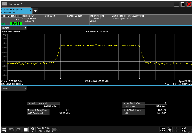
n77_3_10MHz_30kHz_3975MHz_DFT-s-OFDM 16 QAM_RB24@0 8.577MHz
