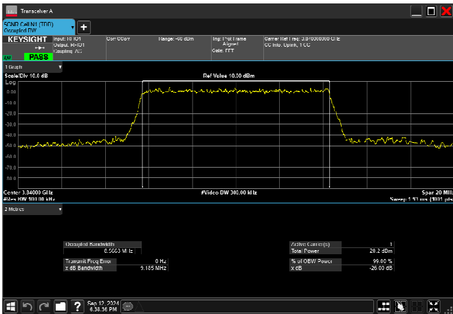
n77_3_10MHz_30kHz_3840MHz_CP-OFDM 64 QAM_RB24@0 8.566MHz
