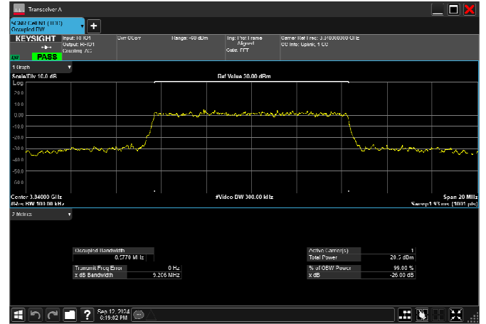
n77_3_10MHz_30kHz_3840MHz_CP-OFDM 256 QAM_RB24@0 8.611MHz
