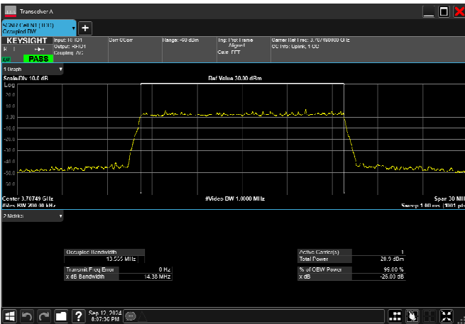
n77_3_15MHz_30kHz_3707.5MHz_CP-OFDM 64 QAM_RB38@0 13.567MHz
