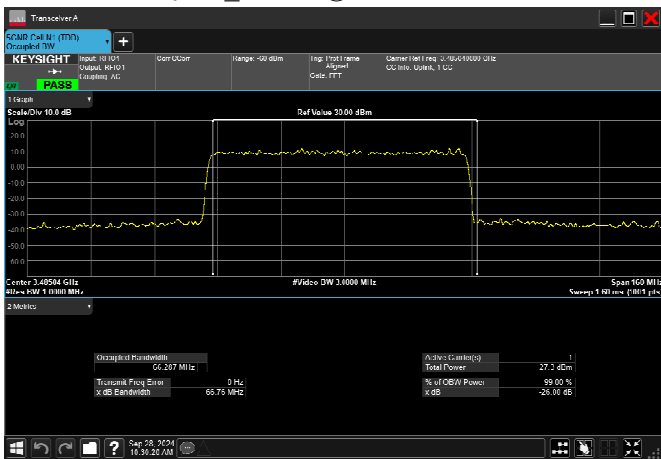
n77_1_70MHz_30kHz_3485MHz_DFT-s-OFDM 256 QAM_RB180@0 66.287MHz
