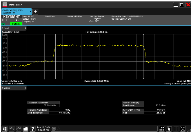
n77_1_60MHz_30kHz_3520MHz_CP-OFDM 64 QAM_RB162@0 57.685MHz
