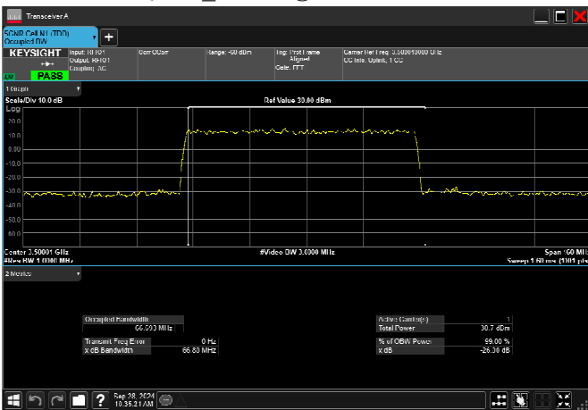
n77_1_70MHz_30kHz_3500MHz_DFT-s-OFDM QPSK_RB180@0 66.693MHz
