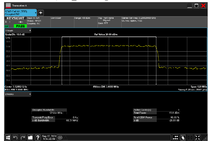
n77_1_60MHz_30kHz_3520MHz_CP-OFDM 256 QAM_RB162@0 57.664MHz
