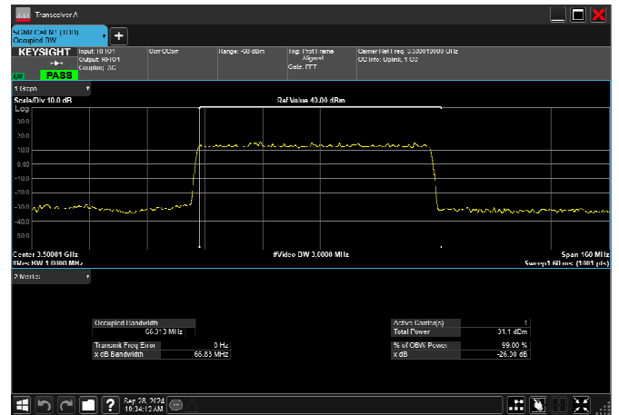
n77_1_70MHz_30kHz_3500MHz_DFT-s-OFDM 16 QAM_RB180@0 66.381MHz
