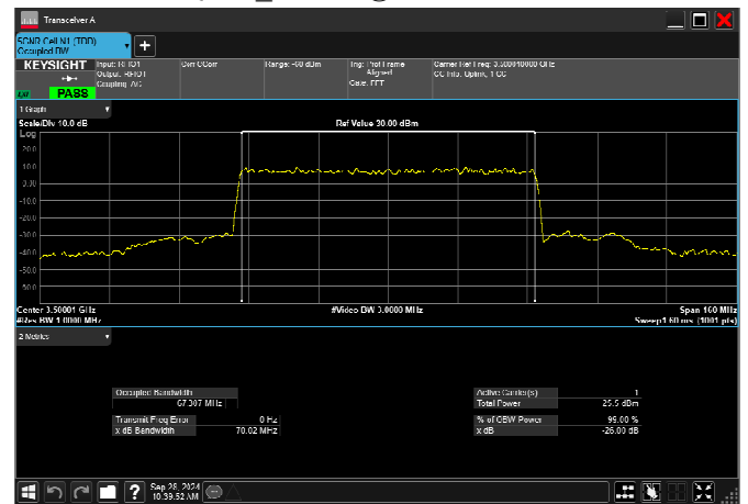
n77_1_70MHz_30kHz_3500MHz_CP-OFDM 256 QAM_RB189@0 67.307MHz
