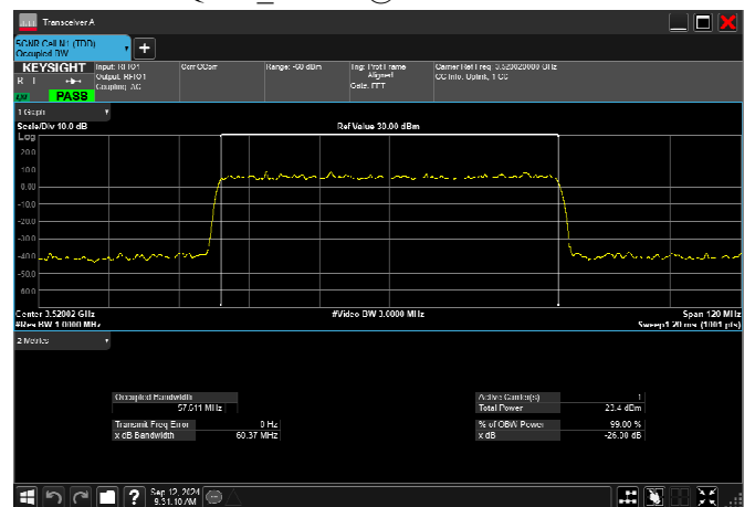
n77_1_60MHz_30kHz_3520MHz_DFT-s-OFDM 16 QAM_RB162@0 57.611MHz
