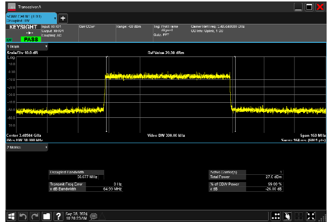
n77_1_70MHz_30kHz_3485MHz_DFT-s-OFDM 64 QAM_RB180@0 66.605MHz
