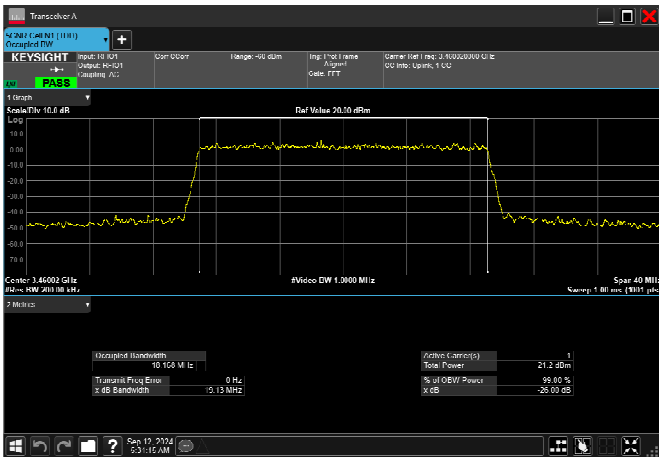
n77_1_20MHz_30kHz_3460MHz_CP-OFDM 64 QAM_RB51@0 18.190MHz
