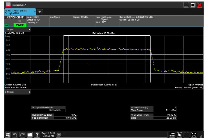
n77_1_20MHz_30kHz_3460MHz_CP-OFDM 256 QAM_RB51@0 18.190MHz
