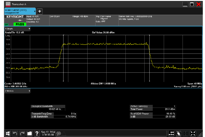
n77_1_20MHz_30kHz_3460MHz_CP-OFDM 16 QAM_RB51@0 18.116MHz
