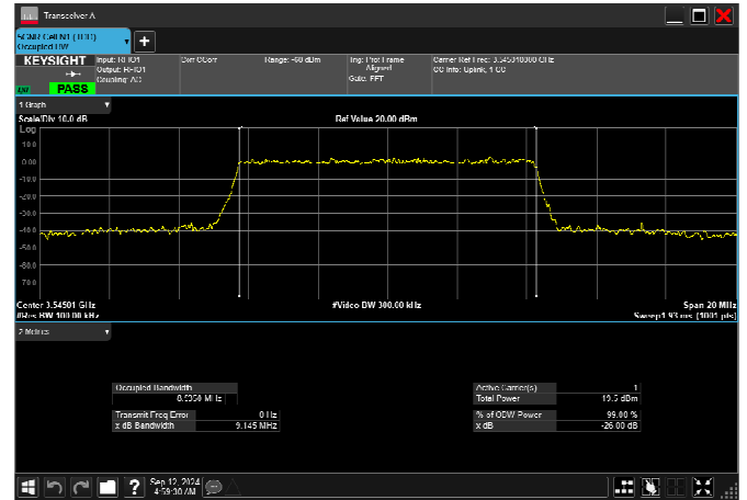
n77_1_10MHz_30kHz_3545MHz_CP-OFDM 16 QAM_RB24@0 8.609MHz
