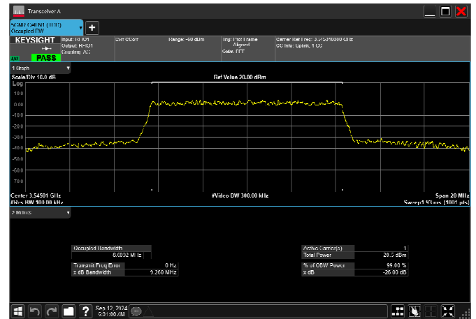
n77_1_10MHz_30kHz_3545MHz_CP-OFDM 256 QAM_RB24@0 8.619MHz
