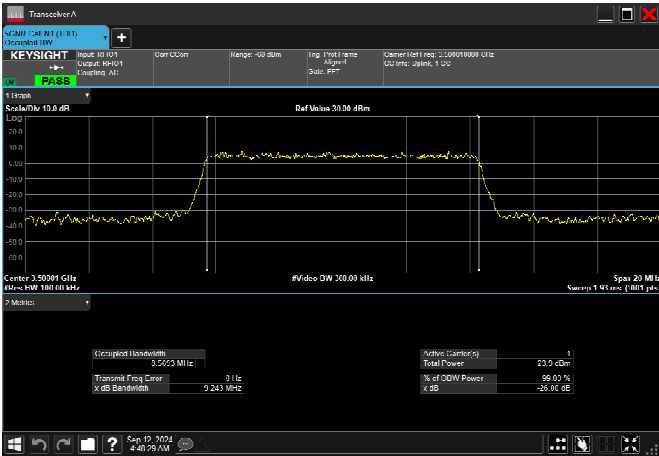
n77_1_10MHz_30kHz_3500MHz_DFT-s-OFDM 16 QAM_RB24@0 8.602MHz
