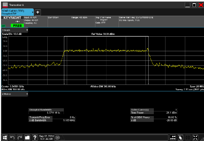
n77_1_10MHz_30kHz_3545MHz_CP-OFDM 64 QAM_RB24@0 8.571MHz
