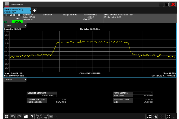
n77_1_10MHz_30kHz_3455MHz_DFT-s-OFDM 16 QAM_RB24@0 8.602MHz
