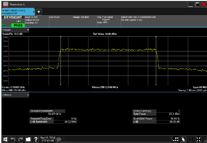
n66_40MHz_15kHz_1760MHz_CP-OFDM 16 QAM_RB216@0 38.479MHz
