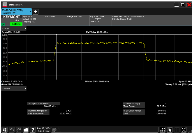
n66_30MHz_15kHz_1725MHz_CP-OFDM 64 QAM_RB160@0 28.466MHz
