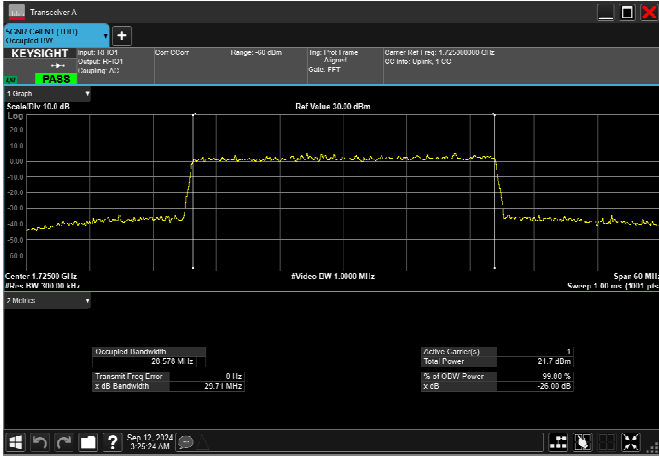
n66_30MHz_15kHz_1725MHz_CP-OFDM QPSK_RB160@0 28.563MHz
