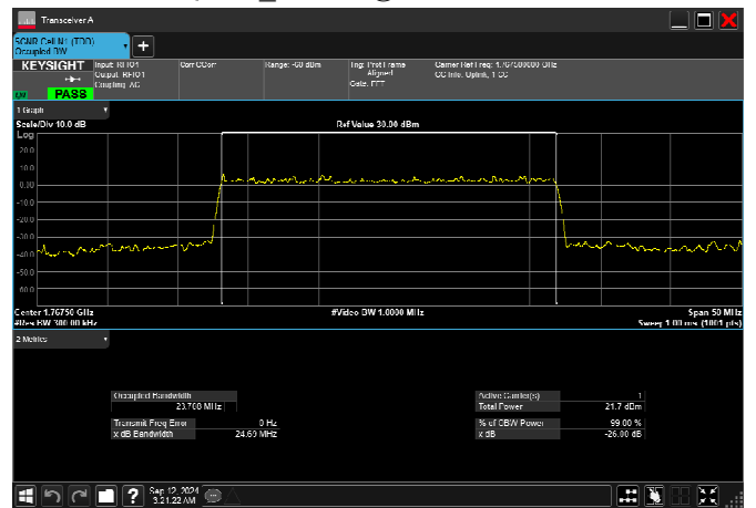
n66_25MHz_15kHz_1767.5MHz_CP-OFDM QPSK_RB133@0 23.708MHz
