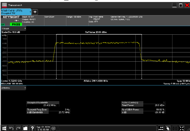
n66_25MHz_15kHz_1722.5MHz_DFT-s-OFDM 256 QAM_RB128@0 23.432MHz
