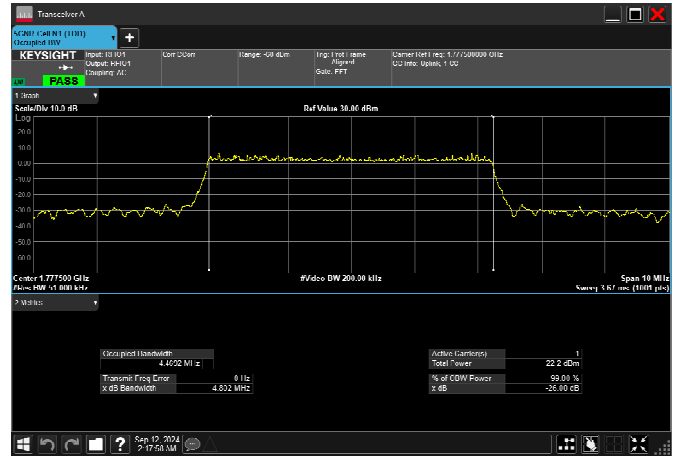
n66_5MHz_15kHz_1777.5MHz_DFT-s-OFDM 64 QAM_RB25@0 4.489MHz
