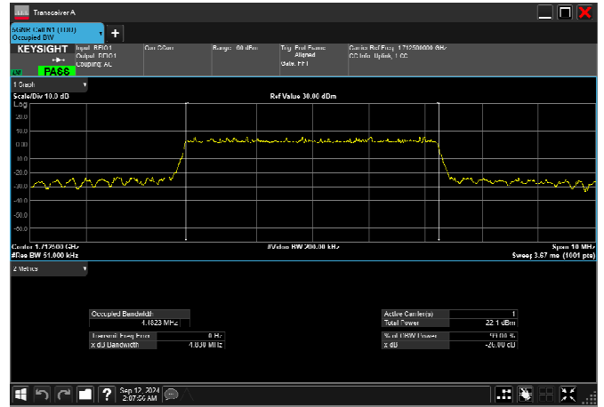
n66_5MHz_15kHz_1712.5MHz_DFT-s-OFDM 64 QAM_RB25@0 4.488MHz
