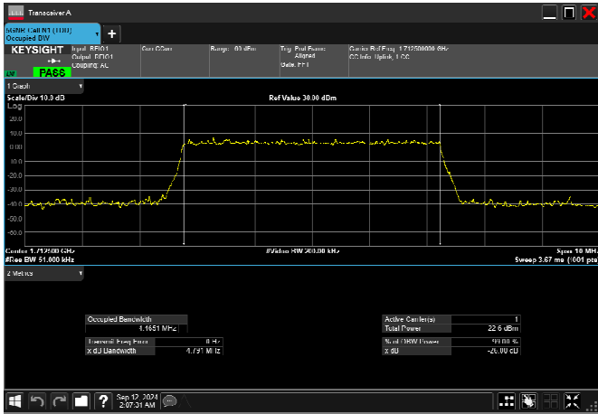
n66_5MHz_15kHz_1712.5MHz_DFT-s-OFDM 16 QAM_RB25@0 4.449MHz
