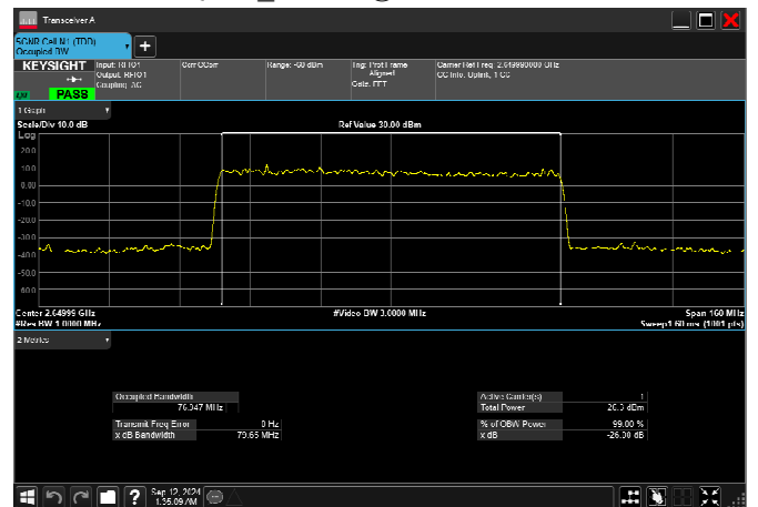
n41_80MHz_30kHz_2649.99MHz_DFT-s-OFDM 16 QAM_RB216@0 76.947MHz
