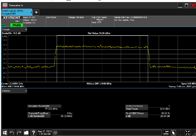
n41_80MHz_30kHz_2649.99MHz_CP-OFDM 64 QAM_RB217@0 77.533MHz
