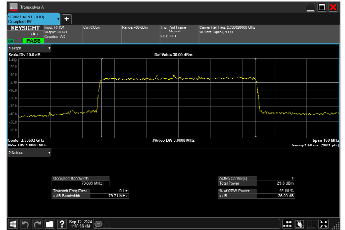
n41_80MHz_30kHz_2536.02MHz_CP-OFDM 16 QAM_RB217@0 77.202MHz
