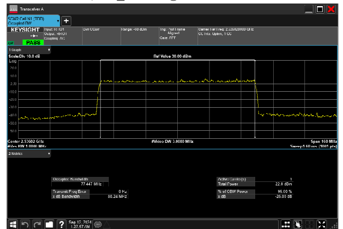
n41_80MHz_30kHz_2536.02MHz_CP-OFDM 256 QAM_RB217@0 77.447MHz
