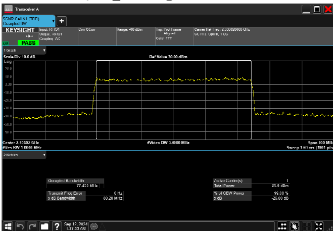
n41_80MHz_30kHz_2536.02MHz_CP-OFDM 64 QAM_RB217@0 77.453MHz
