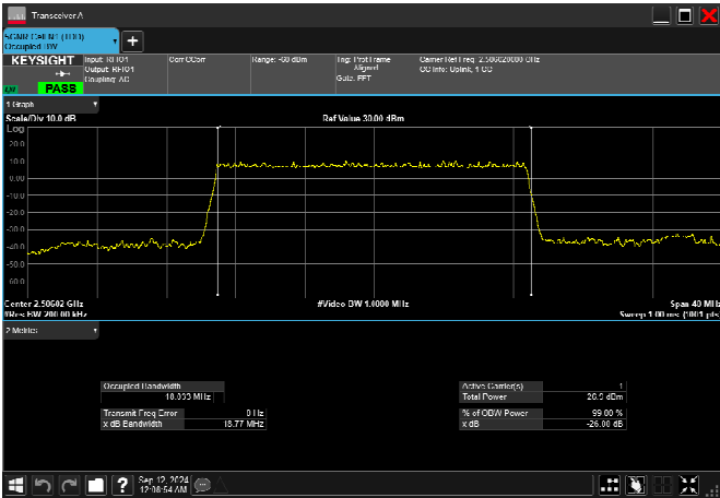
n41_20MHz_30kHz_2506.02MHz_DFT-s-OFDM 16 QAM_RB50@0 18.095MHz
