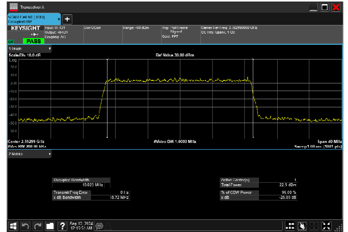
n41_20MHz_30kHz_2592.99MHz_CP-OFDM 16 QAM_RB51@0 18.167MHz
