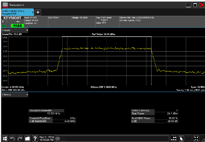
n41_15MHz_30kHz_2503.5MHz_CP-OFDM 64 QAM_RB38@0 13.580MHz
