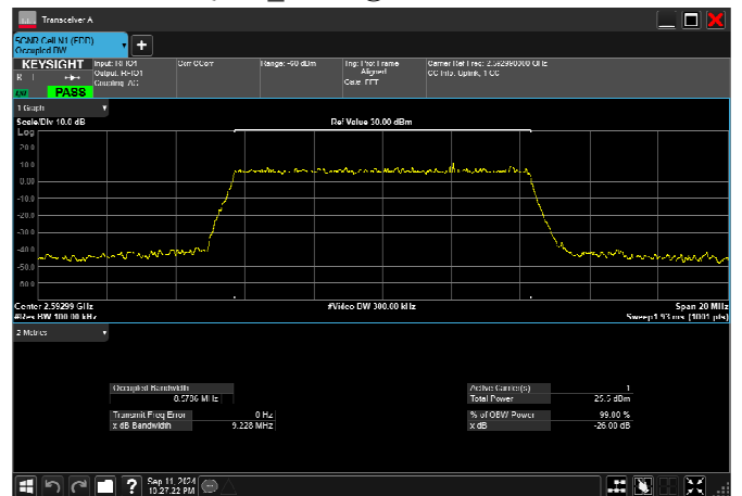
n41_10MHz_30kHz_2592.99MHz_DFT-s-OFDM 16 QAM_RB24@0 8.579MHz
