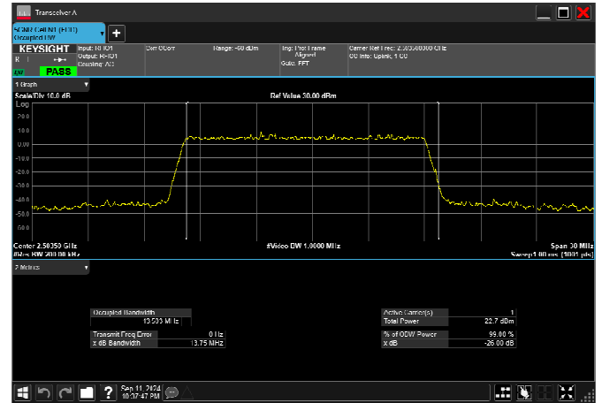
n41_15MHz_30kHz_2503.5MHz_CP-OFDM 16 QAM_RB38@0 13.574MHz
