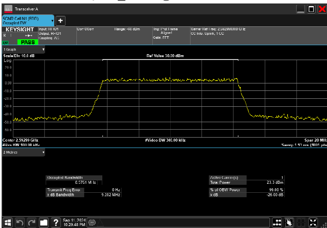
n41_10MHz_30kHz_2592.99MHz_CP-OFDM 64 QAM_RB24@0 8.576MHz
