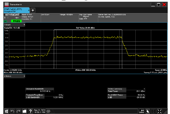
n41_10MHz_30kHz_2592.99MHz_CP-OFDM 256 QAM_RB24@0 8.611MHz
