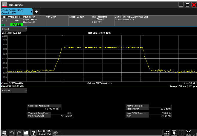
n38_10MHz_30kHz_2575MHz_DFT-s-OFDM 256 QAM_RB24@0 8.535MHz
