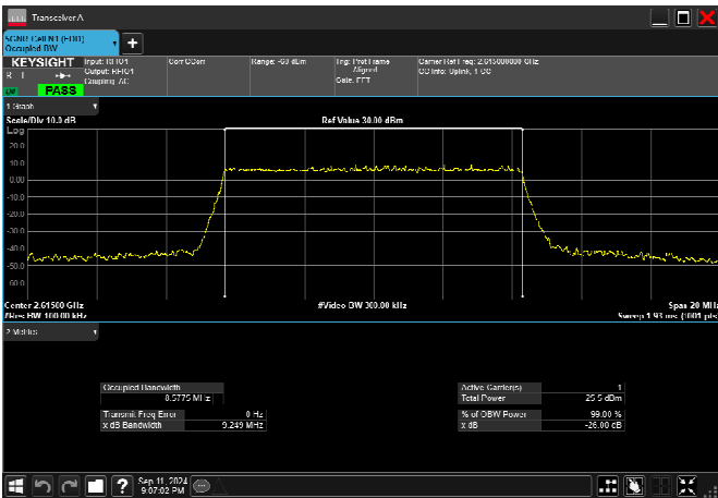
n38_10MHz_30kHz_2615MHz_DFT-s-OFDM 256 QAM_RB24@0 8.537MHz
