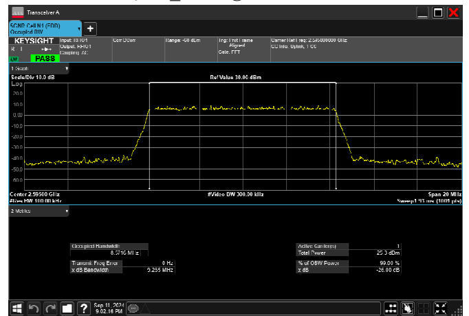
n38_10MHz_30kHz_2595MHz_DFT-s-OFDM 16 QAM_RB24@0 8.572MHz
