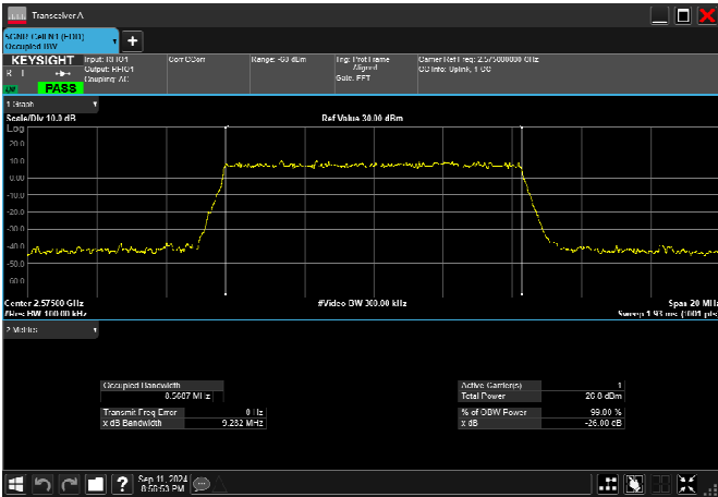
n38_10MHz_30kHz_2575MHz_DFT-s-OFDM 16 QAM_RB24@0 8.570MHz
