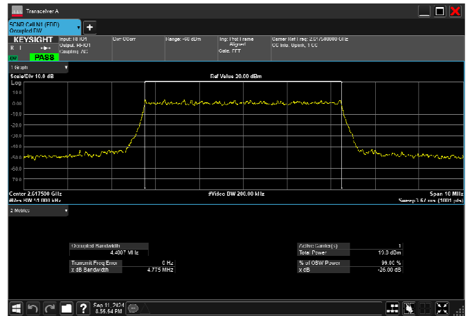
n38_5MHz_15kHz_2617.5MHz_CP-OFDM 256 QAM_RB25@0 4.481MHz
