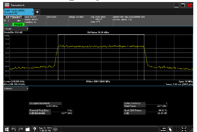
n7_15MHz_15kHz_2562.5MHz_CP-OFDM QPSK_RB79@0 14.063MHz
