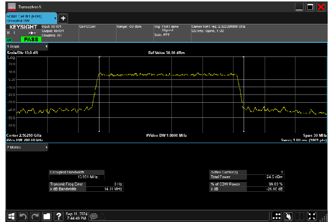
n7_15MHz_15kHz_2562.5MHz_DFT-s-OFDM 64 QAM_RB75@0 13.941MHz
