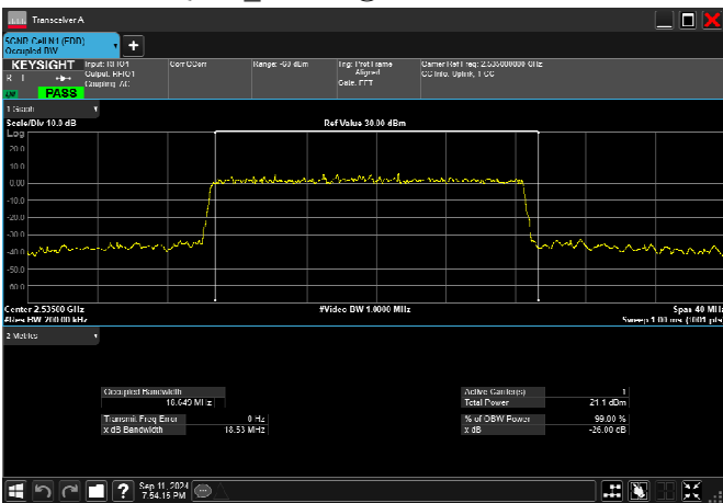
n7_20MHz_15kHz_2535MHz_DFT-s-OFDM 256 QAM_RB100@0 18.649MHz
