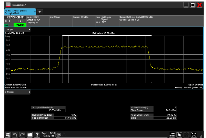
n7_15MHz_15kHz_2535MHz_DFT-s-OFDM 16 QAM_RB75@0 13.946MHz
