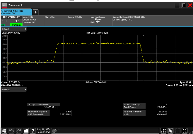
n7_10MHz_15kHz_2535MHz_DFT-s-OFDM 256 QAM_RB50@0 9.204MHz
