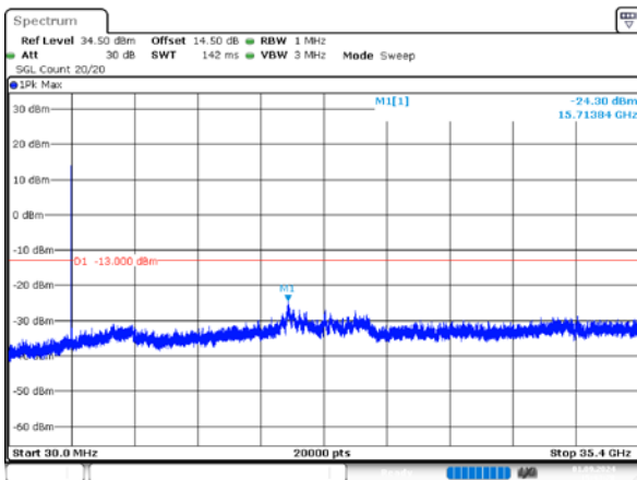
1_20MHz_High_QPSK_1@0
