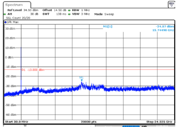
1_5MHz_Low_QPSK_25@0
