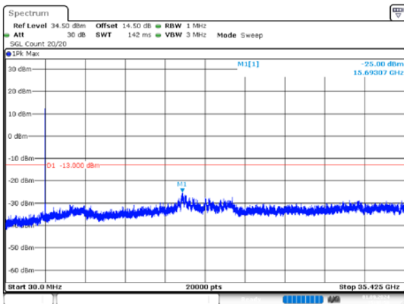
1_15MHz_High_QPSK_1@0
