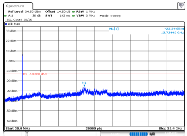
1_20MHz_High_QPSK_100@0
