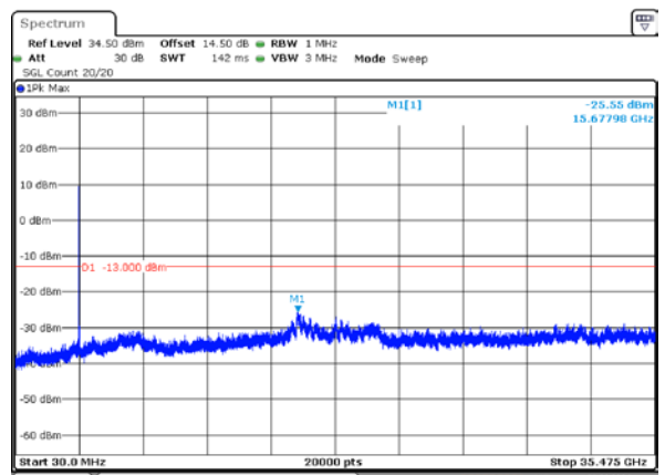
1_5MHz_High_QPSK_25@0
