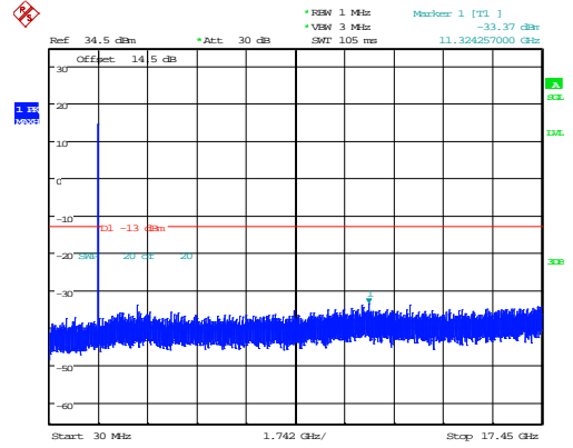
1.4MHz_Middle_QPSK_6@0
