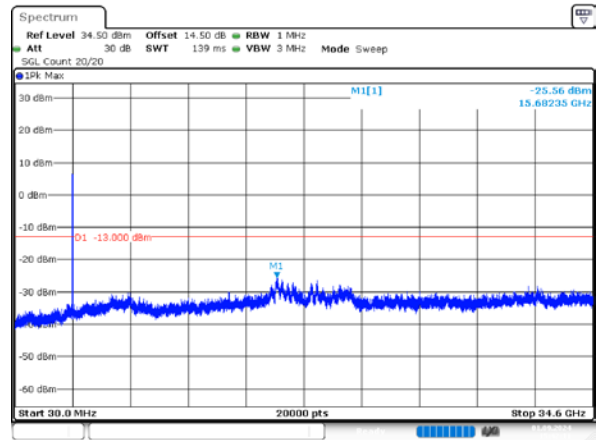
1_20MHz_Low_QPSK_100@0
