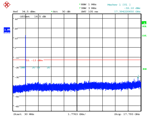
1.4MHz_High_QPSK_6@0
