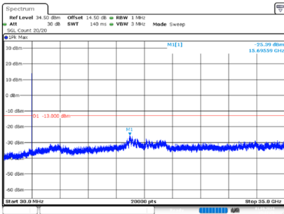
1_10MHz_Middle_QPSK_1@0
