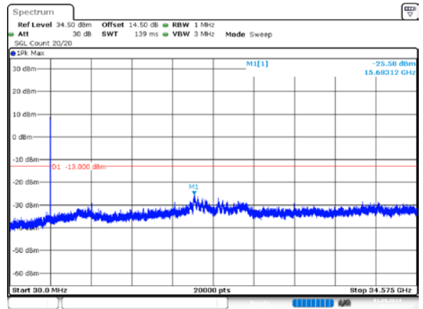
1_15MHz_Low_QPSK_75@0
