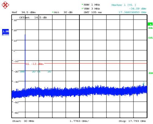
1.4MHz_High_QPSK_1@0
