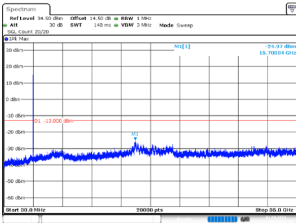
1_20MHz_Middle_QPSK_1@0
