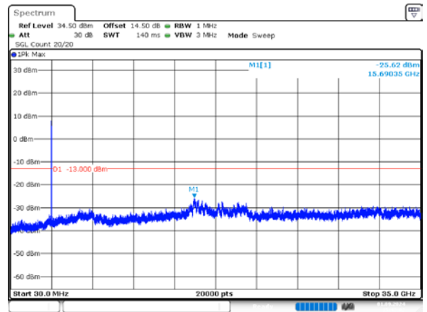
1_20MHz_Middle_QPSK_100@0
