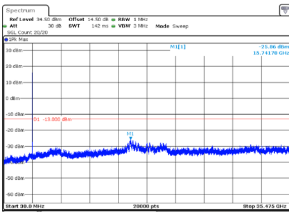
1_5MHz_High_QPSK_1@0
