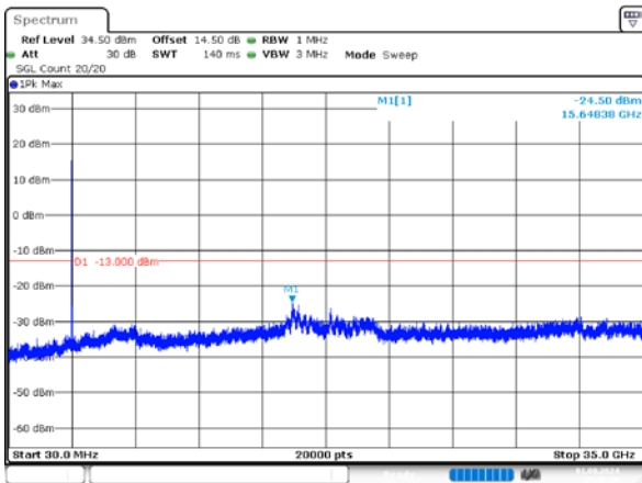
1_15MHz_Middle_QPSK_1@0
