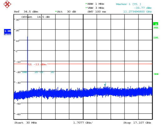
1.4MHz_Low_QPSK_6@0
