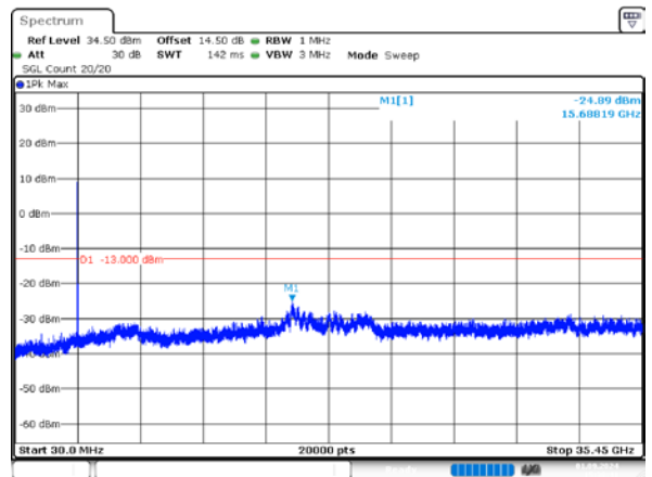
1_10MHz_High_QPSK_50@0
