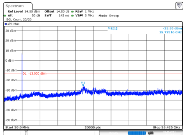
1_15MHz_High_QPSK_75@0
