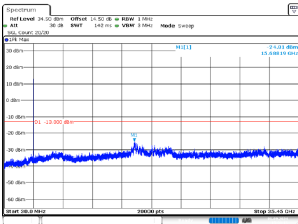
1_10MHz_High_QPSK_1@0
