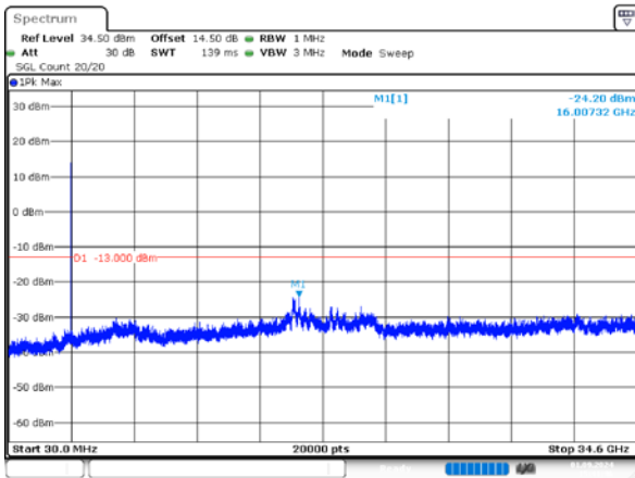
1_20MHz_Low_QPSK_1@0
