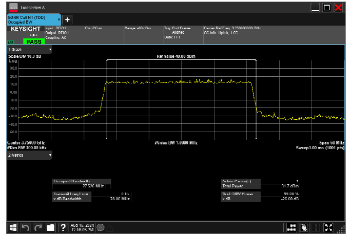
n78_3_30MHz_30kHz_3750MHz_DFT-s-OFDM 16 QAM_RB75@0 27.737MHz
