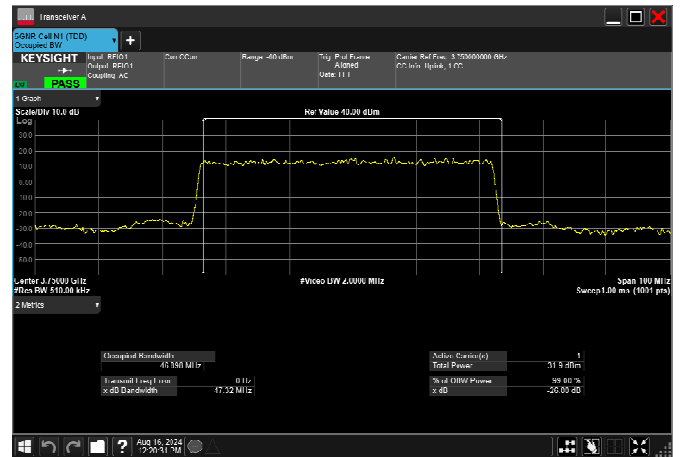
n78_3_50MHz_30kHz_3750MHz_DFT-s-OFDM 16 QAM_RB128@0 46.886MHz
