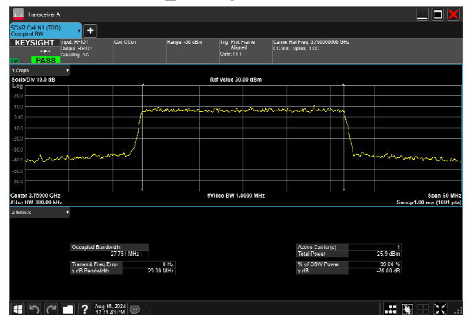
n78_3_30MHz_30kHz_3750MHz_CP-OFDM 256 QAM_RB78@0 27.761MHz
