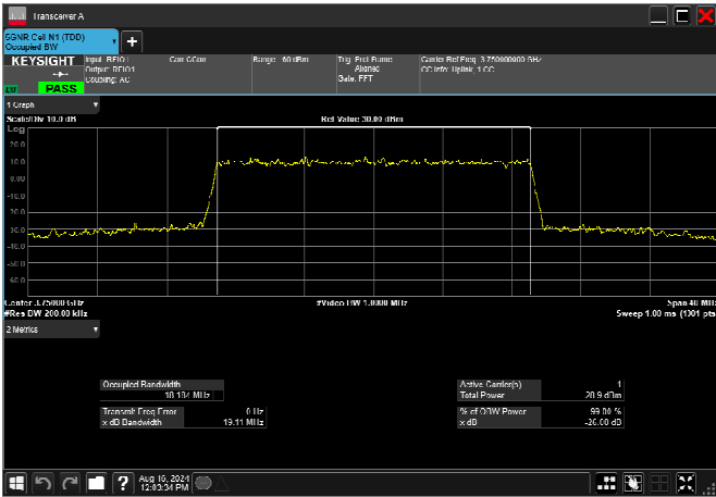
n78_3_20MHz_30kHz_3750MHz_CP-OFDM 256 QAM_RB51@0 18.187MHz
