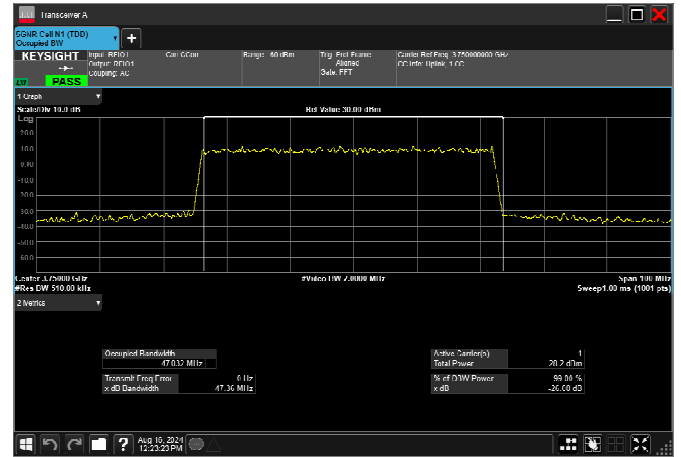
n78_3_50MHz_30kHz_3750MHz_CP-OFDM 16 QAM_RB133@0 47.413MHz
