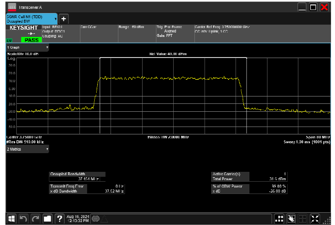
n78_3_40MHz_30kHz_3750MHz_DFT-s-OFDM 64 QAM_RB100@0 37.164MHz
