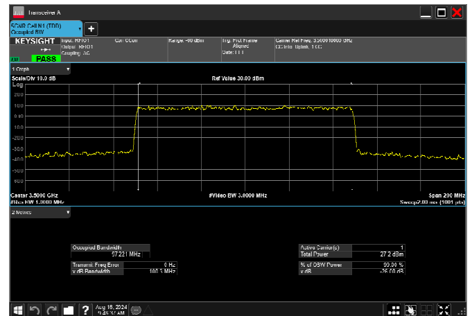
n78_1_100MHz_30kHz_3500MHz_CP-OFDM 256 QAM_RB273@0 97.221MHz
