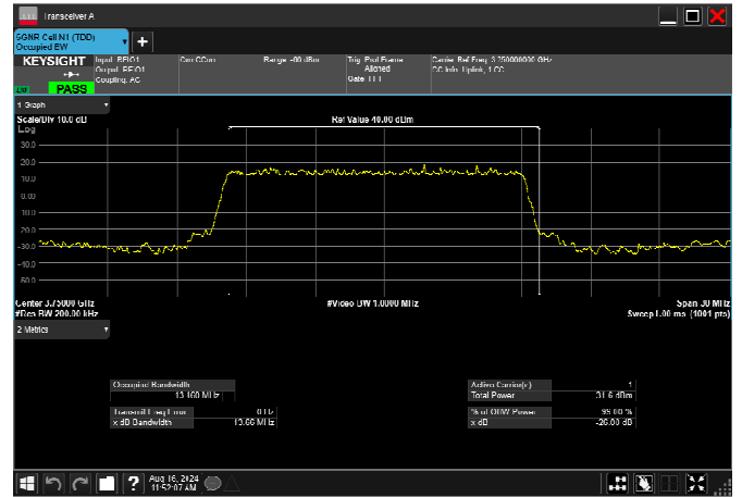
n78_3_15MHz_30kHz_3750MHz_DFT-s-OFDM 16 QAM_RB36@0 13.521MHz
