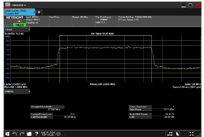
n78_1_60MHz_30kHz_3500MHz_DFT-s-OFDM 16 QAM_RB162@0 57.477MHz
