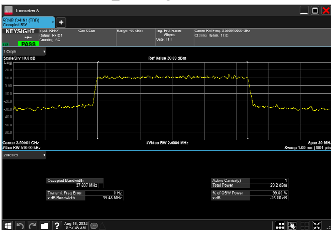
n78_1_40MHz_30kHz_3500MHz_CP-OFDM 64 QAM_RB106@0 37.807MHz
