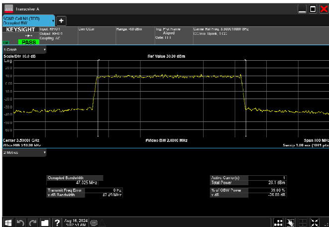
n78_1_50MHz_30kHz_3500MHz_DFT-s-OFDM 256 QAM_RB128@0 47.025MHz
