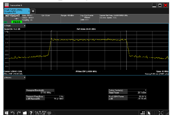
n78_1_40MHz_30kHz_3500MHz_CP-OFDM 256 QAM_RB106@0 37.769MHz
