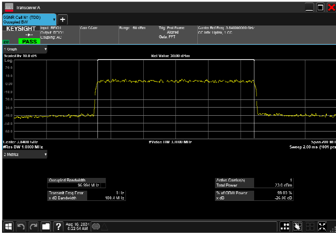
n77_3_100MHz_30kHz_3840MHz_CP-OFDM 16 QAM_RB273@0 96.994MHz
