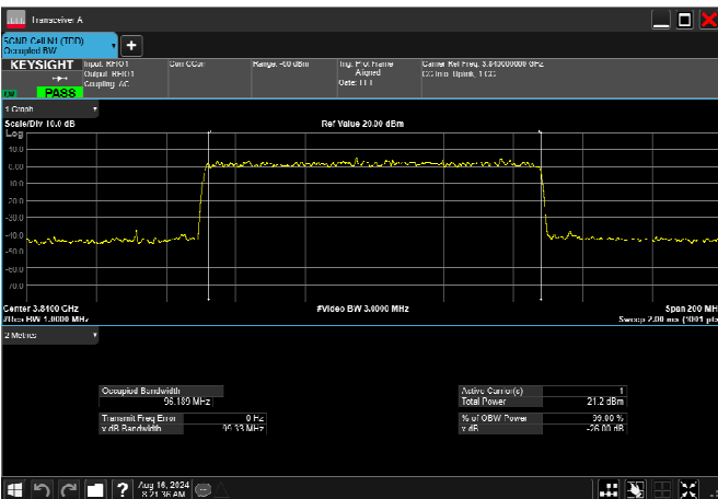
n77_3_100MHz_30kHz_3840MHz_DFT-s-OFDM 256 QAM_RB270@0 96.189MHz
