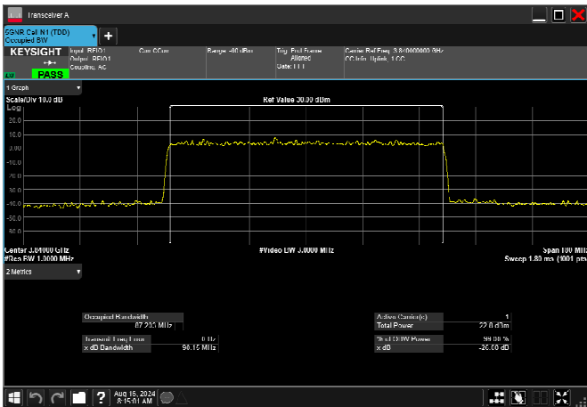
n77_3_90MHz_30kHz_3840MHz_CP-OFDM 64 QAM_RB245@0 87.205MHz
