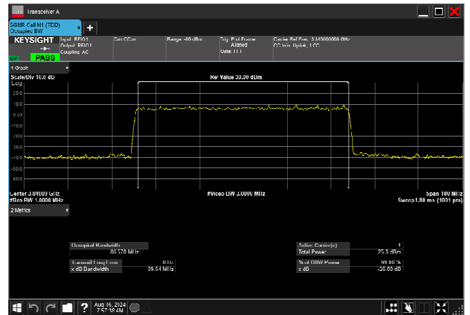
n77_3_90MHz_30kHz_3840MHz_DFT-s-OFDM 16 QAM_RB243@0 86.529MHz
