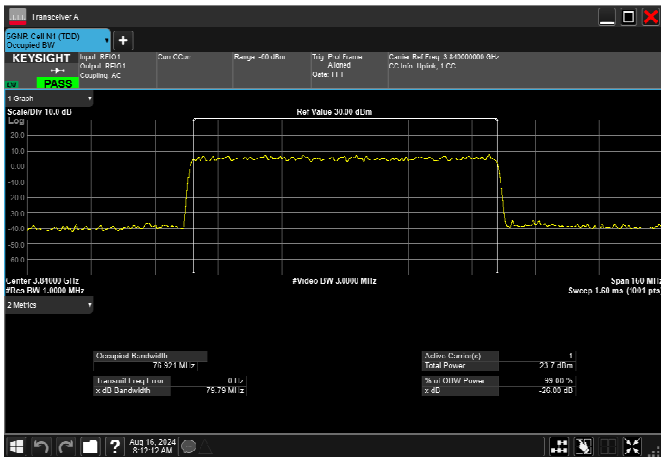
n77_3_80MHz_30kHz_3840MHz_DFT-s-OFDM 256 QAM_RB216@0 76.837MHz
