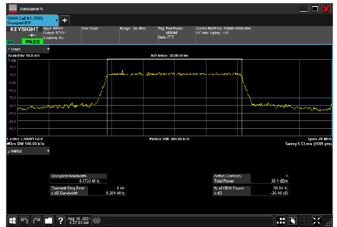
n78_1_10MHz_30kHz_3500MHz_DFT-s-OFDM 16 QAM_RB24@0 8.573MHz
