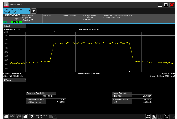
n77_3_20MHz_30kHz_3840MHz_CP-OFDM QPSK_RB51@0 18.167MHz
