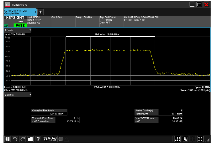
n77_3_15MHz_30kHz_3840MHz_CP-OFDM 16 QAM_RB38@0 13.575MHz
