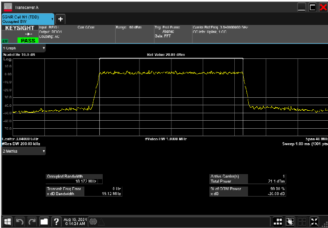
n77_3_20MHz_30kHz_3840MHz_CP-OFDM 256 QAM_RB51@0 18.184MHz
