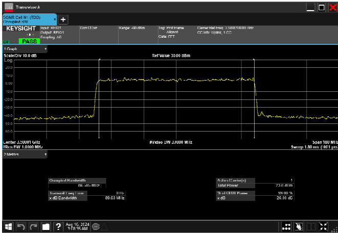
n77_1_90MHz_30kHz_3500MHz_DFT-s-OFDM 256 QAM_RB243@0 86.492MHz
