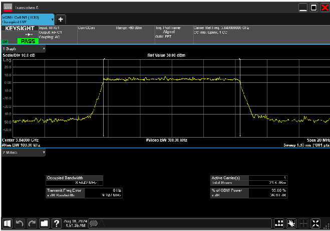
n77_3_10MHz_30kHz_3840MHz_DFT-s-OFDM 16 QAM_RB24@0 8.563MHz
