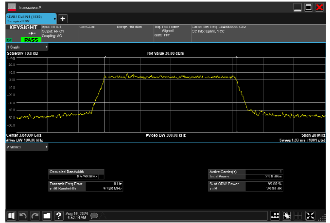
n77_3_10MHz_30kHz_3840MHz_DFT-s-OFDM 64 QAM_RB24@0 8.602MHz
