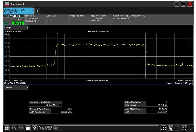
n77_1_90MHz_30kHz_3500MHz_DFT-s-OFDM 64 QAM_RB243@0 86.773MHz
