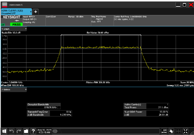
n77_3_10MHz_30kHz_3840MHz_DFT-s-OFDM 256 QAM_RB24@0 8.563MHz
