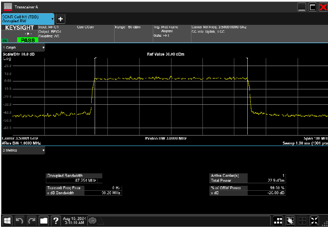
n77_1_90MHz_30kHz_3500MHz_CP-OFDM 256 QAM_RB245@0 87.249MHz
