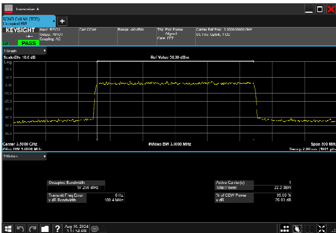
n77_1_100MHz_30kHz_3500MHz_CP-OFDM 64 QAM_RB273@0 97.266MHz
