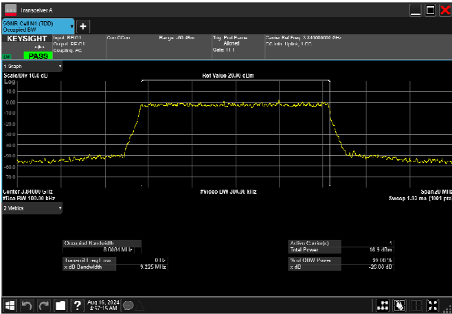
n77_3_15MHz_30kHz_3840MHz_DFT-s-OFDM QPSK_RB36@0 13.441MHz
