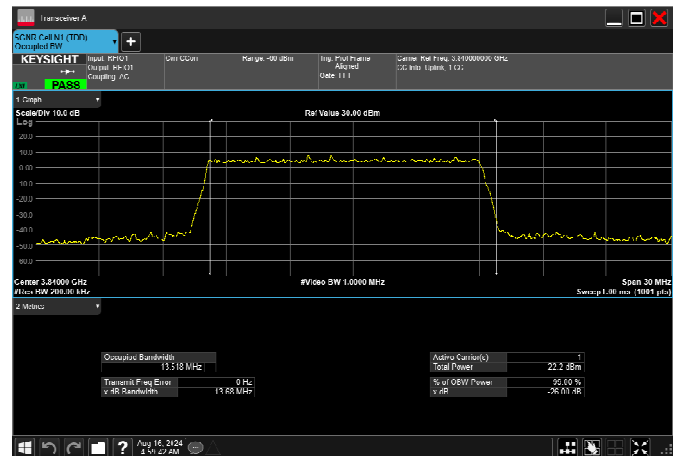
n77_3_15MHz_30kHz_3840MHz_DFT-s-OFDM 16 QAM_RB36@0 13.518MHz
