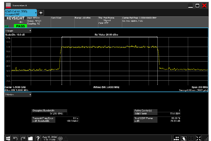
n77_1_100MHz_30kHz_3500MHz_CP-OFDM 256 QAM_RB273@0 97.280MHz
