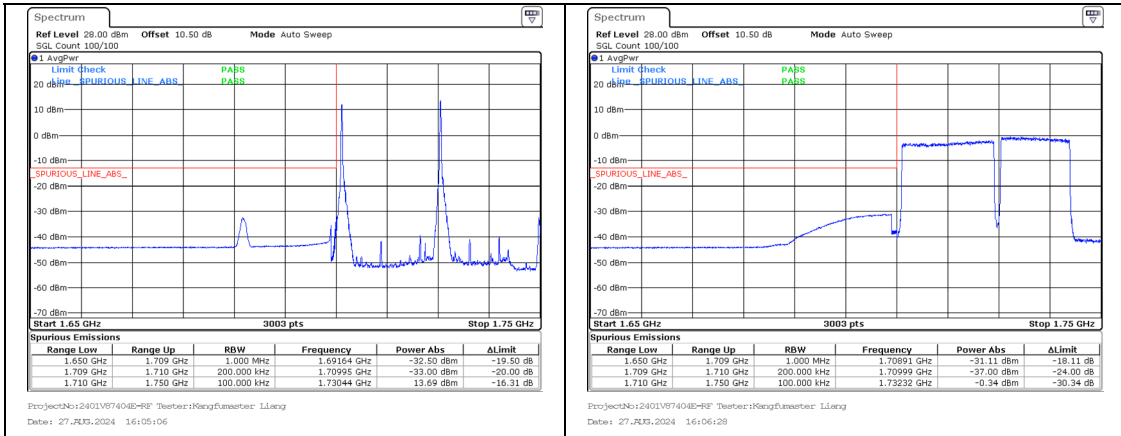
Band 66 20MHz/1720.0/Low QPSK 100@0 Band 66 15MHz/1737.1/Low QPSK 75@0
