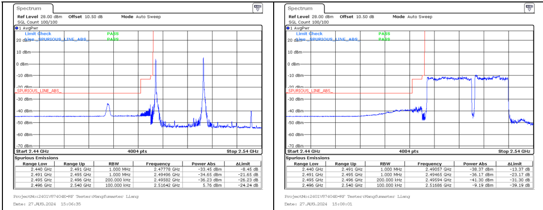
Band 41 20MHz/2506.0/Low 256QAM 1@0 Band 41 15MHz/2523.1/Low 256QAM 1@0
