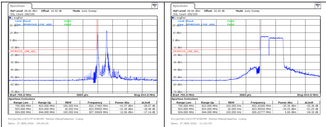
Band 5 3MHz/825.6/Low 16QAM 1@0 Band 5 5MHz/829.5/Low 16QAM 1@0
