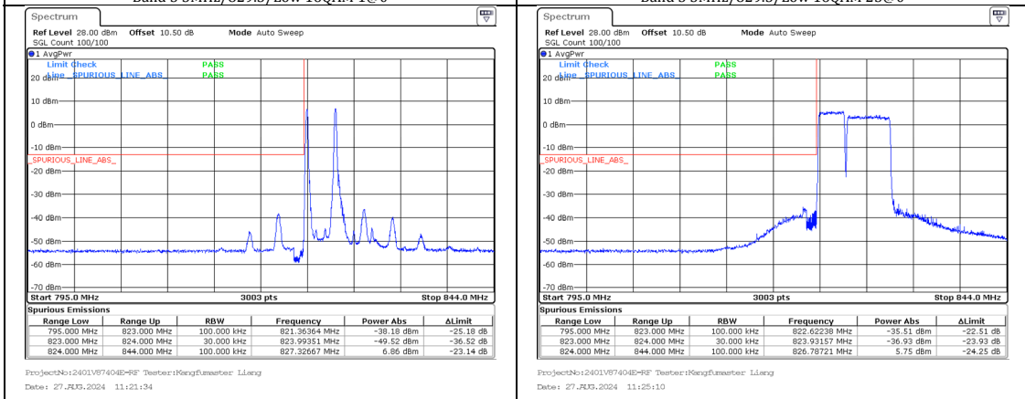
Band 5 3MHz/825.6/Low 64QAM 1@0 Band 5 5MHz/829.5/Low 64QAM 1@0
