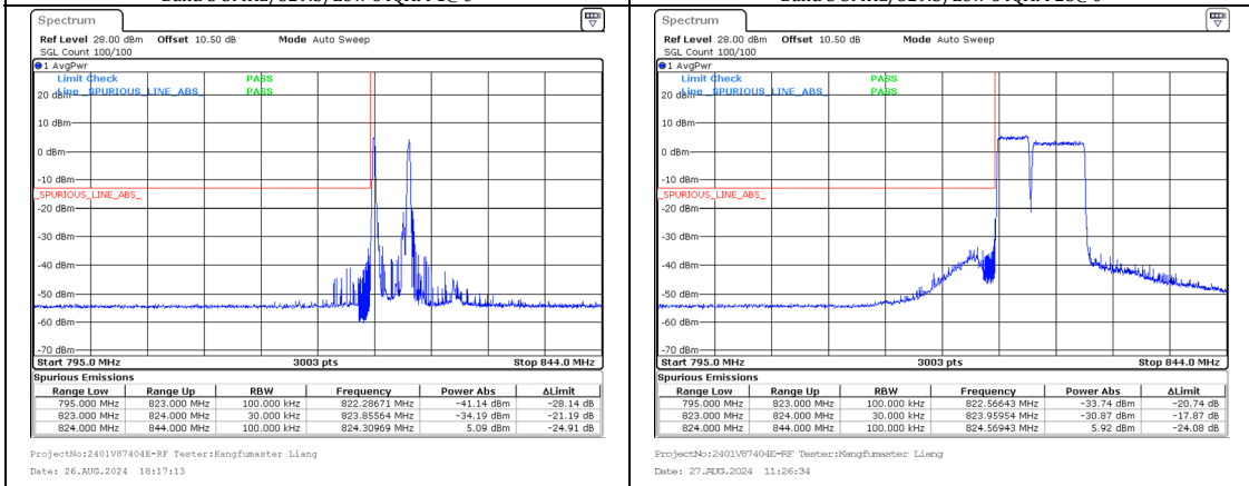
Band 5 3MHz/825.6/Low 256QAM 1@0 Band 5 5MHz/829.5/Low 256QAM 1@0
