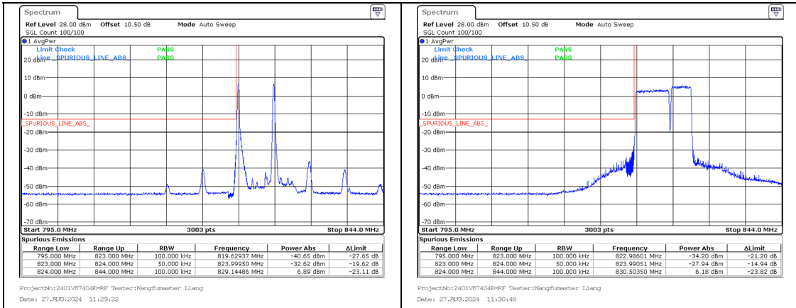
Band 5 5MHz/826.5/Low 256QAM 1@ Band 5 3MHz/830.4/Low 256QAM 1@0
