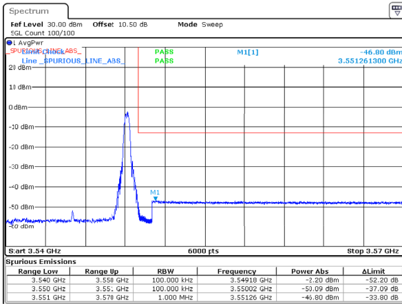
n77_1_10MHz_30kHz_3545MHz_DFT-s-OFDM QPSK_RB1@23 -46.798MHz
