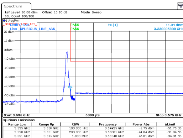
n77_1_15MHz_30kHz_3542.5MHz_DFT-s-OFDM QPSK_RB1@37 -44.844MHz
