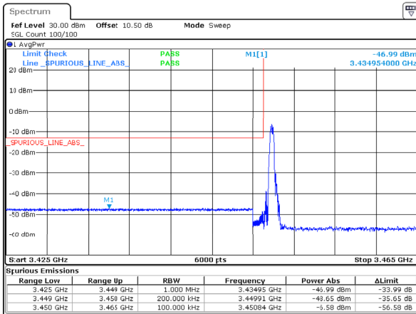
n77_1_15MHz_30kHz_3457.5MHz_DFT-s-OFDM QPSK_RB1@0 -46.989MHz
