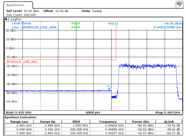
n77_1_15MHz_30kHz_3457.5MHz_DFT-s-OFDM QPSK_RB36@0 -46.946MHz
