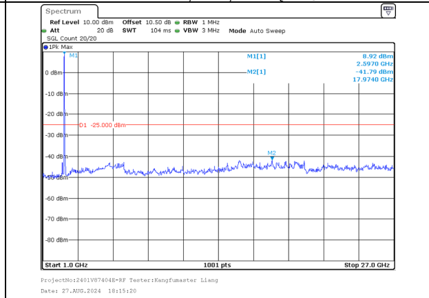
1000.0MHz-27000.0MHz Band 38 15MHz/2587.5/Mid 256QAM 75@0 Band 38 15MHz/2602.5/Mid 256QAM 75@0
