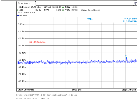
30.0MHz-1000.0MHz Band 38 20MHz/2590.2/High 64QAM 1@99 Band 38 20MHz/2610.0/High 64QAM 1@0
