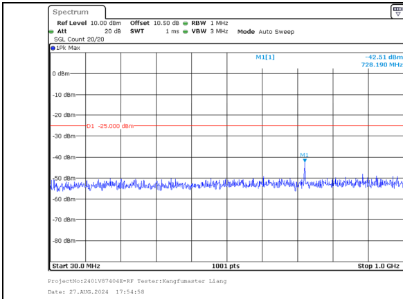
30.0MHz-1000.0MHz Band 38 20MHz/2580.0/Low QPSK 100@0 Band 38 20MHz/2599.8/Low QPSK 100@0
