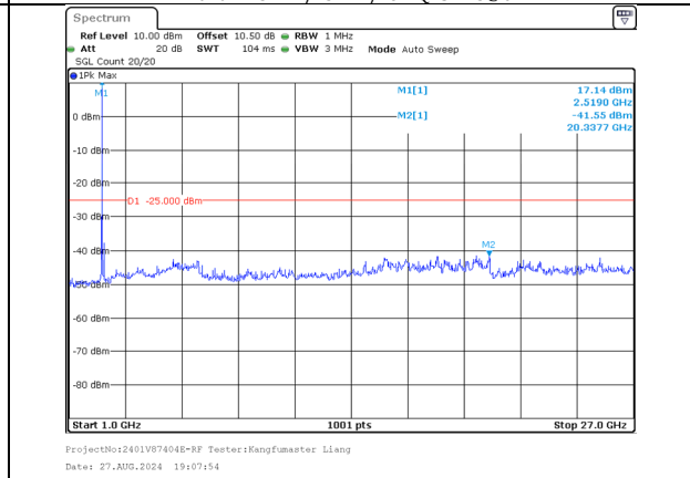
1000.0MHz-27000.0MHz Band 41 20MHz/2506.0/Low 16QAM 1@99 Band 41 5MHz/2517.7/Low 16QAM 1@0
