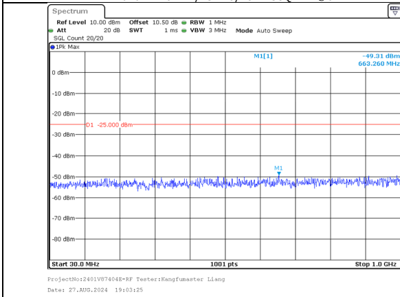
30.0MHz-1000.0MHz Band 41 5MHz/2499.3/Low 256QAM 25@0 Band 41 20MHz/2511.0/Low 256QAM 100@0
