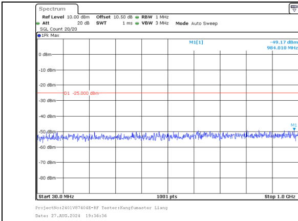
30.0MHz-1000.0MHz Band 41 5MHz/2499.3/Low QPSK 1@24 Band 41 20MHz/2511.0/Low QPSK 1@0
