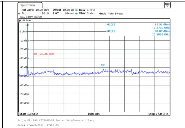
1000.0MHz-27000.0MHz Band 38 15MHz/2577.5/Low 256QAM 1@74 Band 38 15MHz/2592.5/Low 256QAM 1@0
