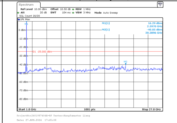
1000.0MHz-27000.0MHz Band 38 15MHz/2577.5/Low 16QAM 1@74 Band 38 15MHz/2592.5/Low 16QAM 1@0
