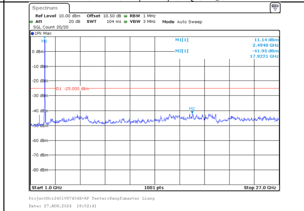
1000.0MHz-27000.0MHz Band 41 5MHz/2499.3/Low QPSK 25@0 Band 41 20MHz/2511.0/Low QPSK 100@0
