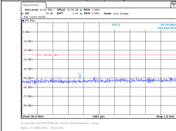
30.0MHz-1000.0MHz Band 38 15MHz/2587.5/Mid 64QAM 1@74 Band 38 15MHz/2602.5/Mid 64QAM 1@0
