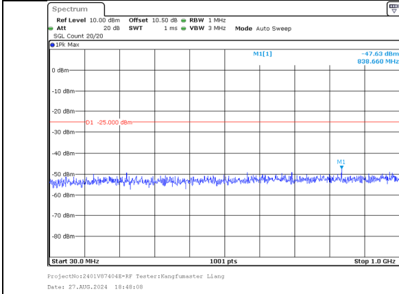
30.0MHz-1000.0MHz Band 38 20MHz/2590.2/High 256QAM 1@99 Band 38 20MHz/2610.0/High 256QAM 1@0
