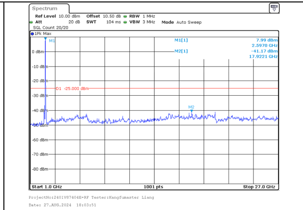
1000.0MHz-27000.0MHz Band 38 20MHz/2580.0/Low 256QAM 100@0 Band 38 20MHz/2599.8/Low 256QAM 100@0
