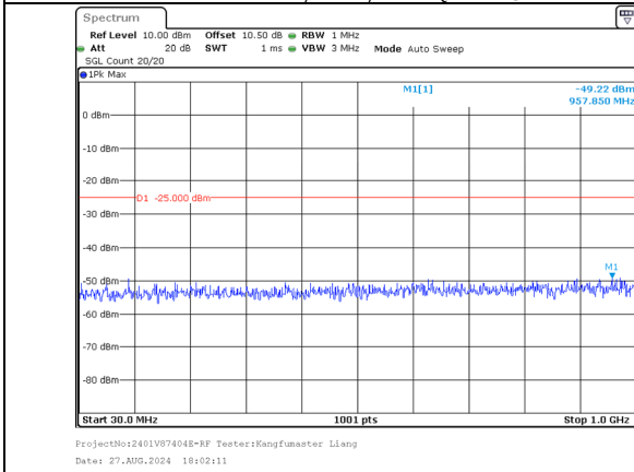
30.0MHz-1000.0MHz Band 38 20MHz/2580.0/Low 256QAM 1@99 Band 38 20MHz/2599.8/Low 256QAM 1@0
