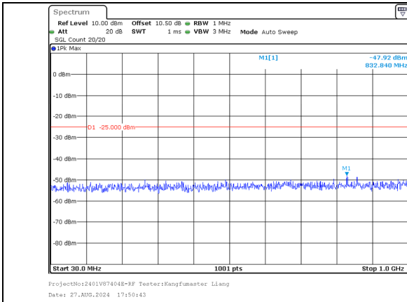
30.0MHz-1000.0MHz Band 38 15MHz/2577.5/Low 256QAM 1@74 Band 38 15MHz/2592.5/Low 256QAM 1@0
