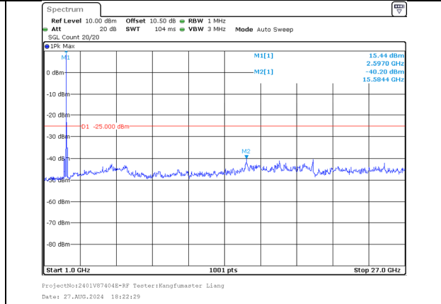
1000.0MHz-27000.0MHz Band 38 20MHz/2585.1/Mid 64QAM 1@99 Band 38 20MHz/2604.9/Mid 64QAM 1@0
