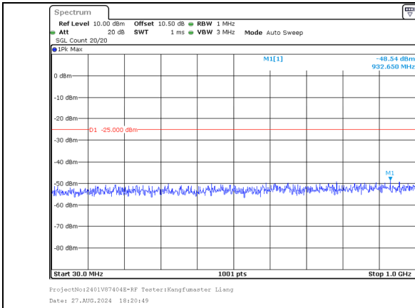
30.0MHz-1000.0MHz Band 38 20MHz/2585.1/Mid 16QAM 100@0 Band 38 20MHz/2604.9/Mid 16QAM 100@0
