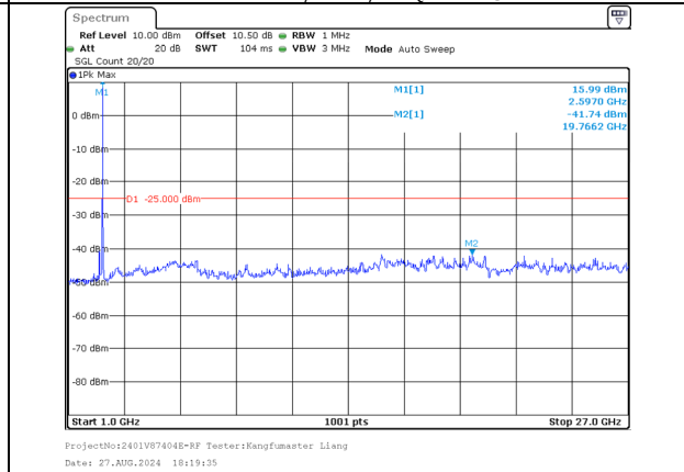
1000.0MHz-27000.0MHz Band 38 20MHz/2585.1/Mid 16QAM 1@99 Band 38 20MHz/2604.9/Mid 16QAM 1@0
