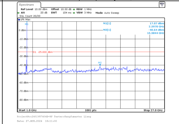
1000.0MHz-27000.0MHz Band 38 15MHz/2587.5/Mid 64QAM 1@74 Band 38 15MHz/2602.5/Mid 64QAM 1@0
