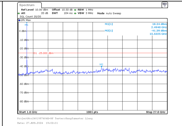
1000.0MHz-27000.0MHz Band 41 5MHz/2499.3/Low 256QAM 1@24 Band 41 20MHz/2511.0/Low 256QAM 1@0
