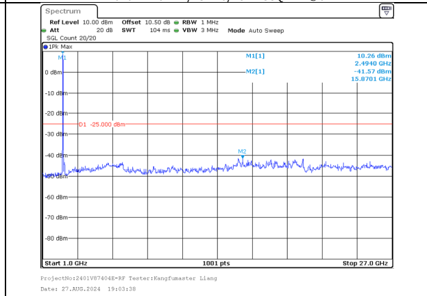
1000.0MHz-27000.0MHz Band 41 5MHz/2499.3/Low 256QAM 25@0 Band 41 20MHz/2511.0/Low 256QAM 100@0
