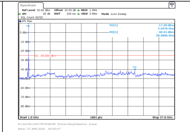
1000.0MHz-27000.0MHz Band 38 15MHz/2587.5/Mid 16QAM 1@74 Band 38 15MHz/2602.5/Mid 16QAM 1@0
