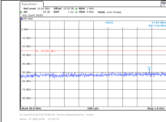
30.0MHz-1000.0MHz Band 41 5MHz/2499.3/Low 64QAM 25@0 Band 41 20MHz/2511.0/Low 64QAM 100@0
