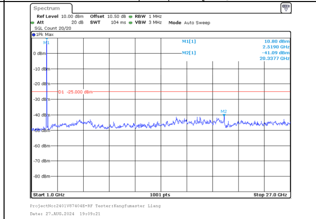
1000.0MHz-27000.0MHz Band 41 20MHz/2506.0/Low 16QAM 100@0 Band 41 5MHz/2517.7/Low 16QAM 25@0
