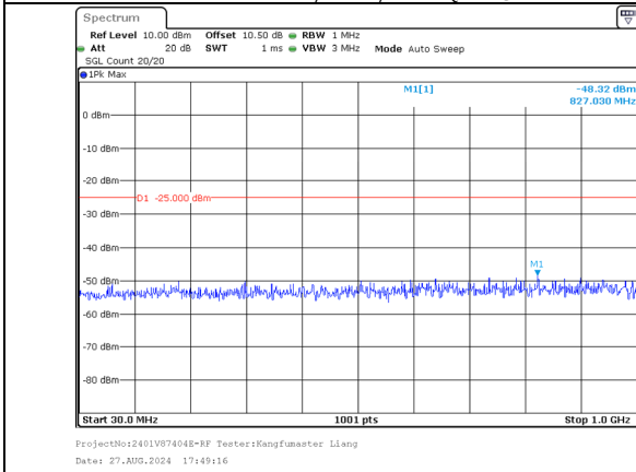
30.0MHz-1000.0MHz Band 38 15MHz/2577.5/Low 64QAM 75@0 Band 38 15MHz/2592.5/Low 64QAM 75@0
