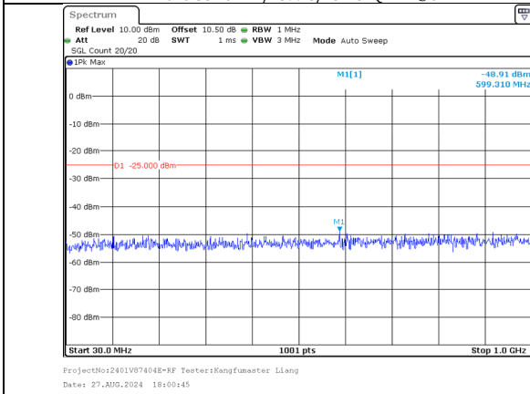
30.0MHz-1000.0MHz Band 38 20MHz/2580.0/Low 64QAM 100@0 Band 38 20MHz/2599.8/Low 64QAM 100@0
