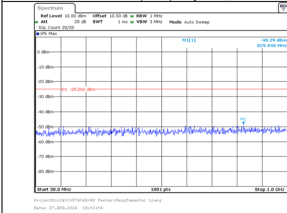
30.0MHz-1000.0MHz Band 41 5MHz/2499.3/Low 16QAM 1@24 Band 41 20MHz/2511.0/Low 16QAM 1@0
