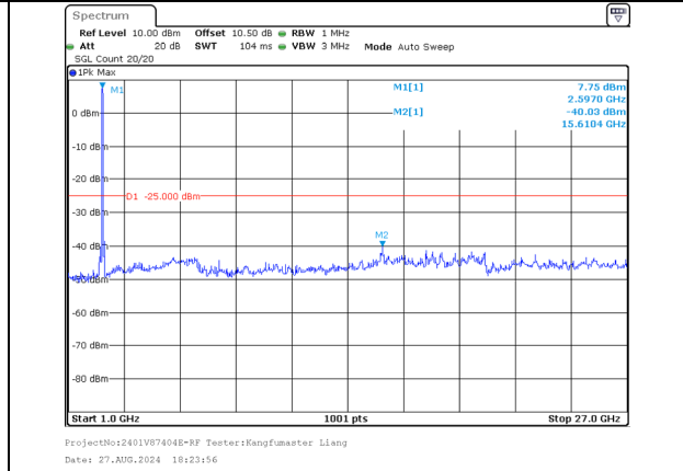
1000.0MHz-27000.0MHz Band 38 20MHz/2585.1/Mid 64QAM 100@0 Band 38 20MHz/2604.9/Mid 64QAM 100@0
