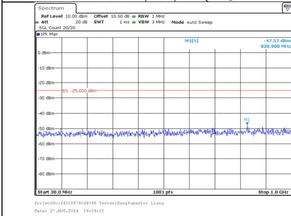
30.0MHz-1000.0MHz Band 38 15MHz/2587.5/Mid 16QAM 75@0 Band 38 15MHz/2602.5/Mid 16QAM 75@0
