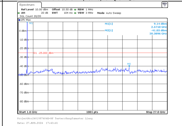
1000.0MHz-27000.0MHz Band 38 15MHz/2577.5/Low QPSK 75@0 Band 38 15MHz/2592.5/Low QPSK 75@0
