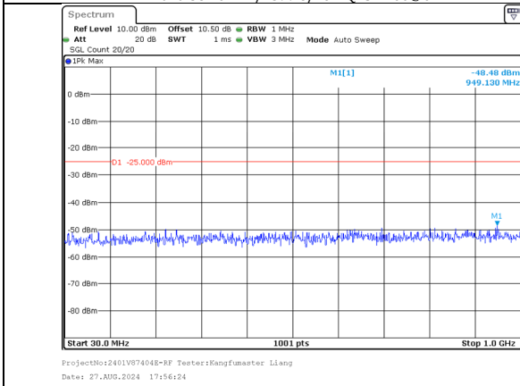
30.0MHz-1000.0MHz Band 38 20MHz/2580.0/Low 16QAM 1@99 Band 38 20MHz/2599.8/Low 16QAM 1@0
