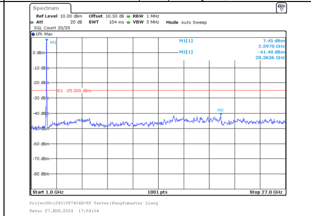
1000.0MHz-27000.0MHz Band 38 20MHz/2580.0/Low 16QAM 100@0 Band 38 20MHz/2599.8/Low 16QAM 100@0
