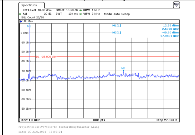
1000.0MHz-27000.0MHz Band 38 20MHz/2580.0/Low 256QAM 1@99 Band 38 20MHz/2599.8/Low 256QAM 1@0
