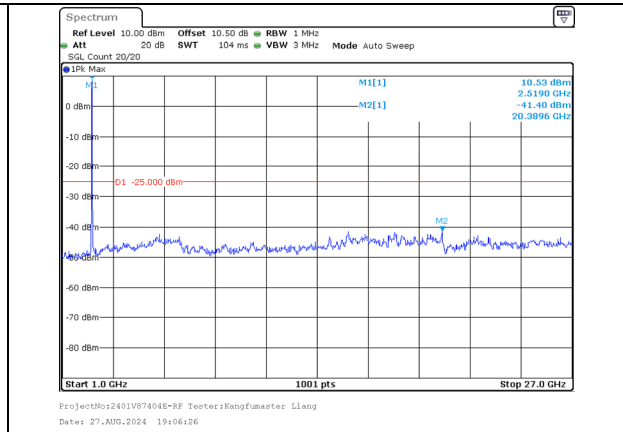
1000.0MHz-27000.0MHz Band 41 20MHz/2506.0/Low QPSK 100@0 Band 41 5MHz/2517.7/Low QPSK 25@0
