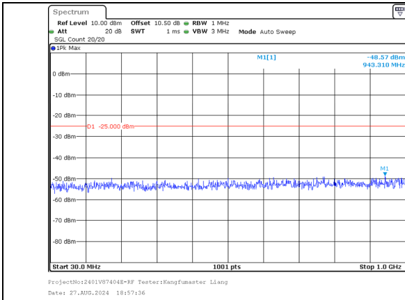
30.0MHz-1000.0MHz Band 41 5MHz/2499.3/Low 16QAM 25@0 Band 41 20MHz/2511.0/Low 16QAM 100@0
