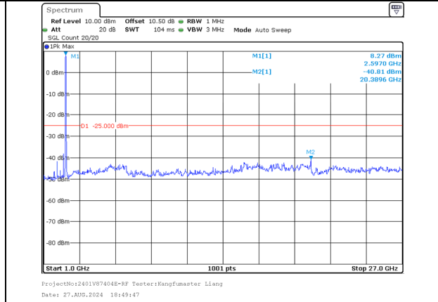
1000.0MHz-27000.0MHz Band 38 20MHz/2590.2/High 256QAM 100@0 Band 38 20MHz/2610.0/High 256QAM 100@0
