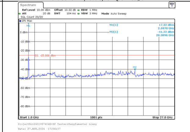
1000.0MHz-27000.0MHz Band 38 20MHz/2580.0/Low 16QAM 1@99 Band 38 20MHz/2599.8/Low 16QAM 1@0
