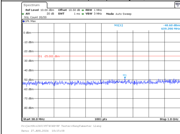
30.0MHz-1000.0MHz Band 38 15MHz/2587.5/Mid 256QAM 75@0 Band 38 15MHz/2602.5/Mid 256QAM 75@0
