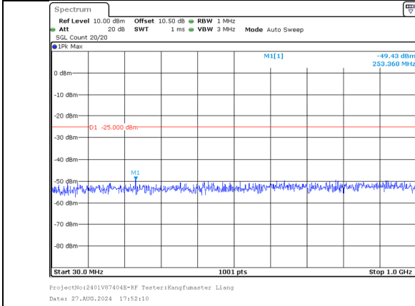
30.0MHz-1000.0MHz Band 38 15MHz/2577.5/Low 256QAM 75@0 Band 38 15MHz/2592.5/Low 256QAM 75@0
