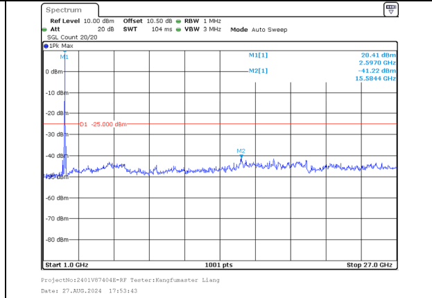
1000.0MHz-27000.0MHz Band 38 20MHz/2580.0/Low QPSK 1@99 Band 38 20MHz/2599.8/Low QPSK 1@0
