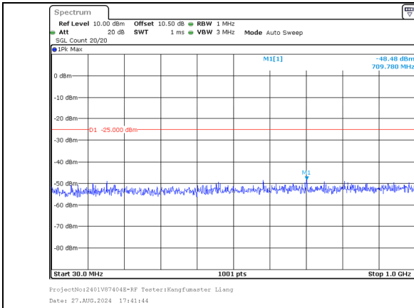
30.0MHz-1000.0MHz Band 38 15MHz/2577.5/Low QPSK 1@74 Band 38 15MHz/2592.5/Low QPSK 1@0
