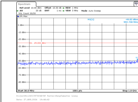
30.0MHz-1000.0MHz Band 38 20MHz/2590.2/High 64QAM 100@0 Band 38 20MHz/2610.0/High 64QAM 100@0
