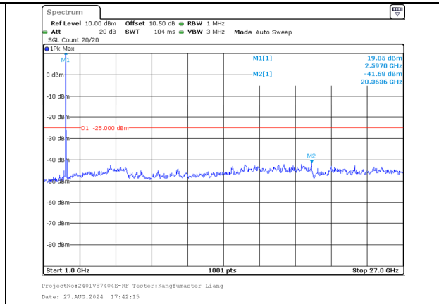
1000.0MHz-27000.0MHz Band 38 15MHz/2577.5/Low QPSK 1@74 Band 38 15MHz/2592.5/Low QPSK 1@0
