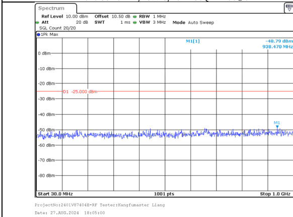
30.0MHz-1000.0MHz Band 38 15MHz/2587.5/Mid QPSK 1@74 Band 38 15MHz/2602.5/Mid QPSK 1@0
