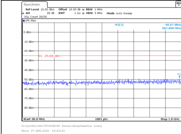
30.0MHz-1000.0MHz Band 38 20MHz/2585.1/Mid 64QAM 100@0 Band 38 20MHz/2604.9/Mid 64QAM 100@0
