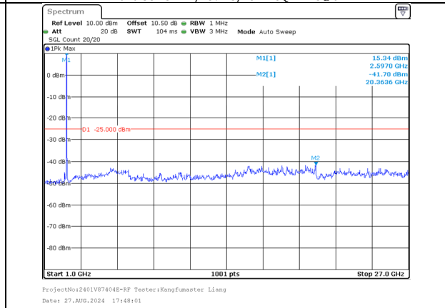
1000.0MHz-27000.0MHz Band 38 15MHz/2577.5/Low 64QAM 1@74 Band 38 15MHz/2592.5/Low 64QAM 1@0
