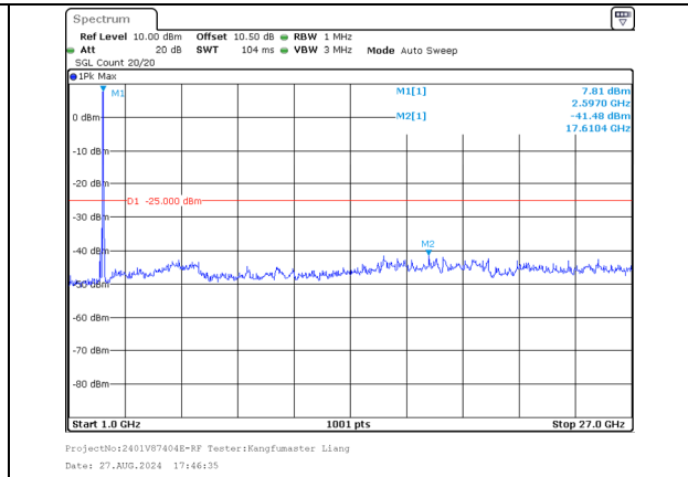
1000.0MHz-27000.0MHz Band 38 15MHz/2577.5/Low 16QAM 75@0 Band 38 15MHz/2592.5/Low 16QAM 75@0
