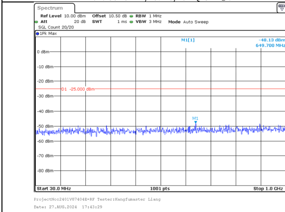
30.0MHz-1000.0MHz Band 38 15MHz/2577.5/Low QPSK 75@0 Band 38 15MHz/2592.5/Low QPSK 75@0
