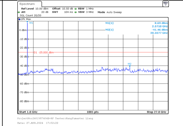
1000.0MHz-27000.0MHz Band 38 15MHz/2577.5/Low 256QAM 75@0 Band 38 15MHz/2592.5/Low 256QAM 75@0
