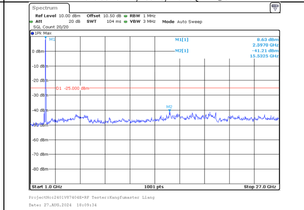
1000.0MHz-27000.0MHz Band 38 15MHz/2587.5/Mid 16QAM 75@0 Band 38 15MHz/2602.5/Mid 16QAM 75@0
