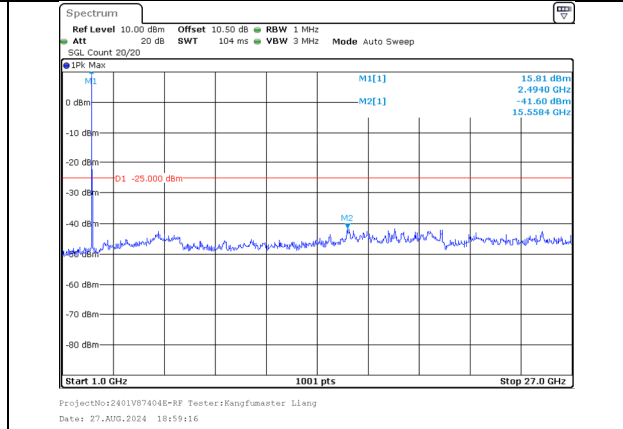
1000.0MHz-27000.0MHz Band 41 5MHz/2499.3/Low 64QAM 1@24 Band 41 20MHz/2511.0/Low 64QAM 1@0
