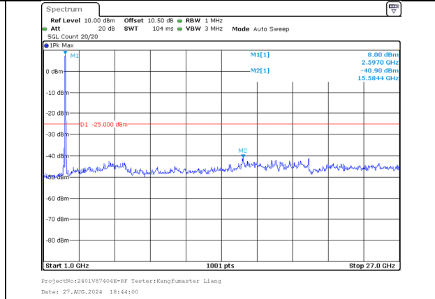
1000.0MHz-27000.0MHz Band 38 20MHz/2590.2/High 16QAM 100@0 Band 38 20MHz/2610.0/High 16QAM 100@0
