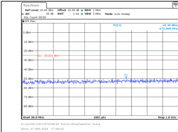
30.0MHz-1000.0MHz Band 38 15MHz/2577.5/Low 16QAM 75@0 Band 38 15MHz/2592.5/Low 16QAM 75@0
