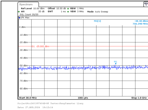
30.0MHz-1000.0MHz Band 38 15MHz/2587.5/Mid 64QAM 75@0 Band 38 15MHz/2602.5/Mid 64QAM 75@0
