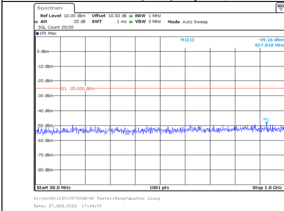
30.0MHz-1000.0MHz Band 38 15MHz/2577.5/Low 16QAM 1@74 Band 38 15MHz/2592.5/Low 16QAM 1@0
