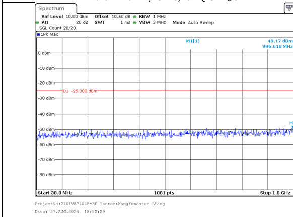
30.0MHz-1000.0MHz Band 41 5MHz/2499.3/Low QPSK 25@0 Band 41 20MHz/2511.0/Low QPSK 100@0
