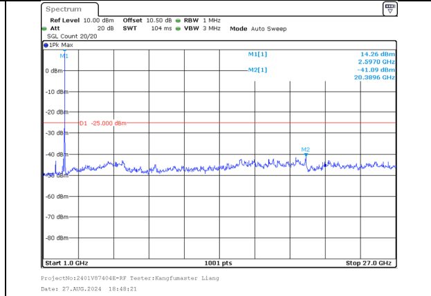
1000.0MHz-27000.0MHz Band 38 20MHz/2590.2/High 256QAM 1@99 Band 38 20MHz/2610.0/High 256QAM 1@0
