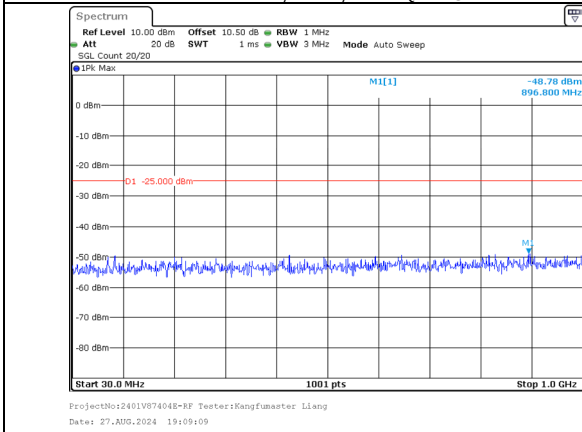
30.0MHz-1000.0MHz Band 41 20MHz/2506.0/Low 16QAM 100@0 Band 41 5MHz/2517.7/Low 16QAM 25@0
