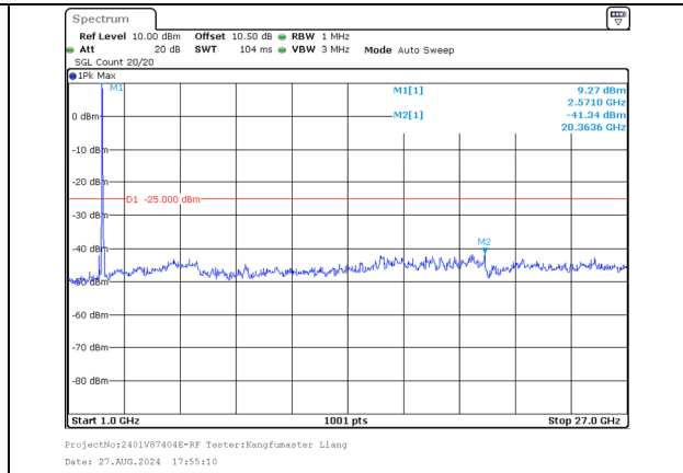
1000.0MHz-27000.0MHz Band 38 20MHz/2580.0/Low QPSK 100@0 Band 38 20MHz/2599.8/Low QPSK 100@0
