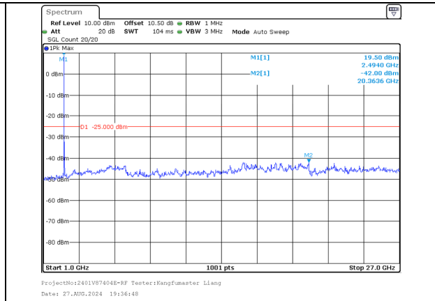
1000.0MHz-27000.0MHz Band 41 5MHz/2499.3/Low QPSK 1@24 Band 41 20MHz/2511.0/Low QPSK 1@0
