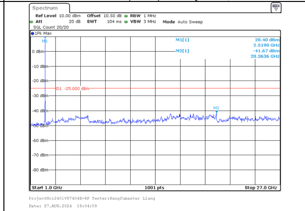
1000.0MHz-27000.0MHz Band 41 20MHz/2506.0/Low QPSK 1@99 Band 41 5MHz/2517.7/Low QPSK 1@0
