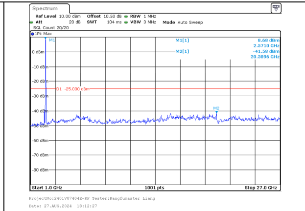
1000.0MHz-27000.0MHz Band 38 15MHz/2587.5/Mid 64QAM 75@0 Band 38 15MHz/2602.5/Mid 64QAM 75@0
