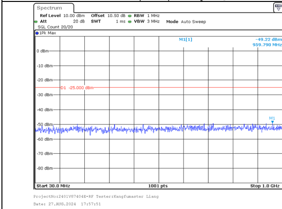
30.0MHz-1000.0MHz Band 38 20MHz/2580.0/Low 16QAM 100@0 Band 38 20MHz/2599.8/Low 16QAM 100@0
