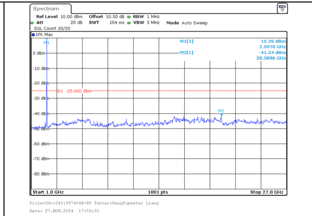
1000.0MHz-27000.0MHz Band 38 20MHz/2580.0/Low 64QAM 1@99 Band 38 20MHz/2599.8/Low 64QAM 1@0
