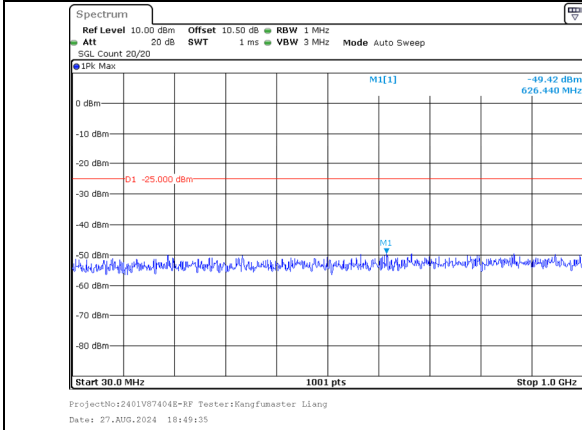
30.0MHz-1000.0MHz Band 38 20MHz/2590.2/High 256QAM 100@0 Band 38 20MHz/2610.0/High 256QAM 100@0
