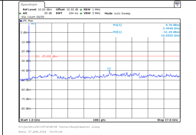
1000.0MHz-27000.0MHz Band 41 5MHz/2499.3/Low 64QAM 25@0 Band 41 20MHz/2511.0/Low 64QAM 100@0
