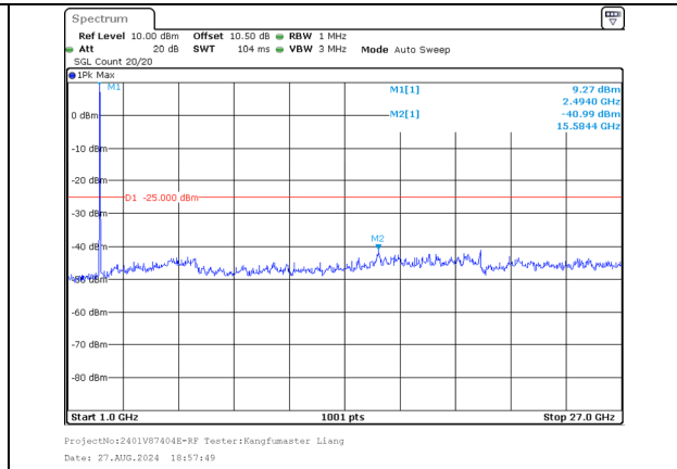
1000.0MHz-27000.0MHz Band 41 5MHz/2499.3/Low 16QAM 25@0 Band 41 20MHz/2511.0/Low 16QAM 100@0
