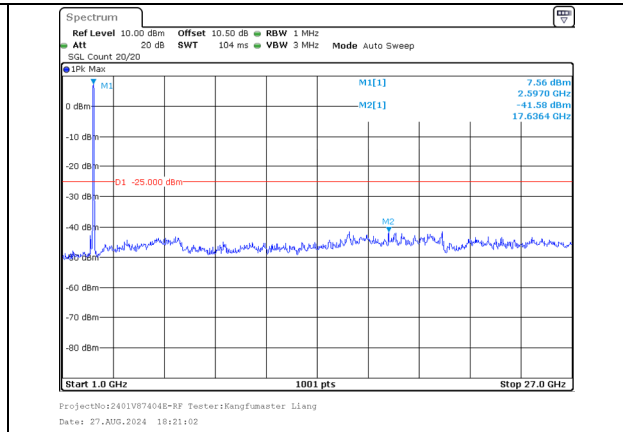
1000.0MHz-27000.0MHz Band 38 20MHz/2585.1/Mid 16QAM 100@0 Band 38 20MHz/2604.9/Mid 16QAM 100@0
