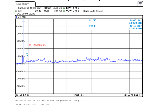
1000.0MHz-27000.0MHz Band 38 15MHz/2587.5/Mid 256QAM 1@74 Band 38 15MHz/2602.5/Mid 256QAM 1@0
