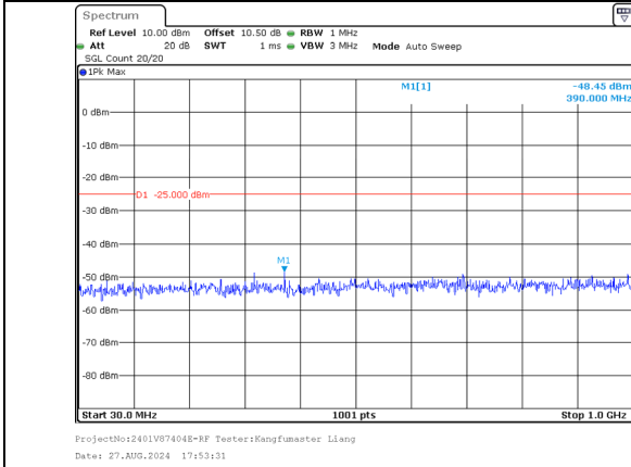
30.0MHz-1000.0MHz Band 38 20MHz/2580.0/Low QPSK 1@99 Band 38 20MHz/2599.8/Low QPSK 1@0
