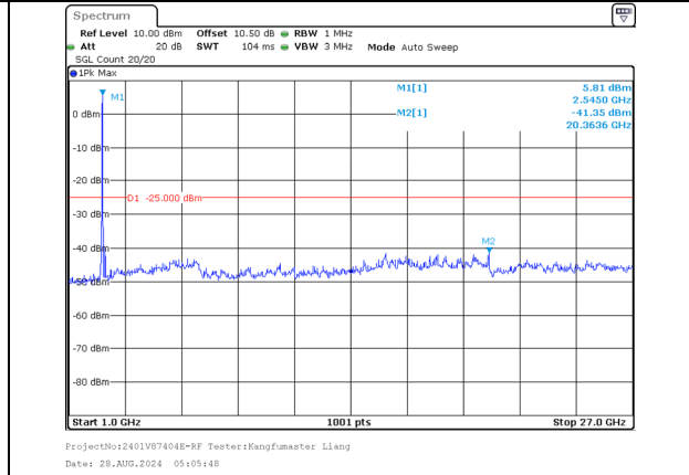
1000.0MHz-27000.0MHz Band 7 20MHz/2540.2/High 256QAM 100@0 Band 7 20MHz/2560.0/High 256QAM 100@0
