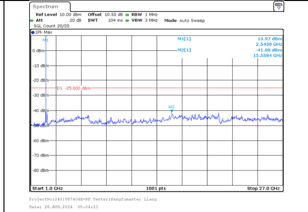
1000.0MHz-27000.0MHz Band 7 20MHz/2540.2/High 256QAM 1@99 Band 7 20MHz/2560.0/High 256QAM 1@0
