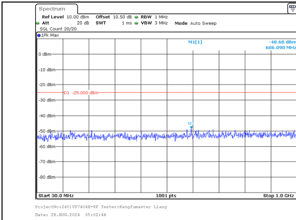
30.0MHz-1000.0MHz Band 7 20MHz/2540.2/High 64QAM 100@0 Band 7 20MHz/2560.0/High 64QAM 100@0
