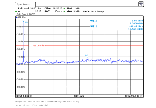
1000.0MHz-27000.0MHz Band 7 15MHz/2542.9/High 16QAM 75@0 Band 7 20MHz/2560.0/High 16QAM 100@0
