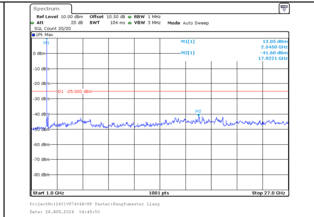
1000.0MHz-27000.0MHz Band 7 20MHz/2545.1/High 64QAM 1@99 Band 7 15MHz/2562.2/High 64QAM 1@0
