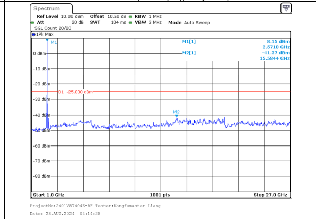
1000.0MHz-27000.0MHz Band 7 20MHz/2550.1/High 16QAM 100@0 Band 7 10MHz/2564.5/High 16QAM 100@0
