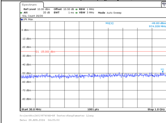
30.0MHz-1000.0MHz Band 7 10MHz/2545.6/High 64QAM 50@0 Band 7 20MHz/2560.0/High 64QAM 100@0
