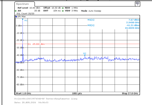
1000.0MHz-27000.0MHz Band 7 10MHz/2545.6/High 64QAM 50@0 Band 7 20MHz/2560.0/High 64QAM 100@0
