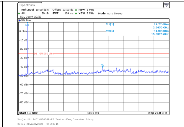
1000.0MHz-27000.0MHz Band 7 20MHz/2540.2/High 16QAM 1@99 Band 7 20MHz/2560.0/High 16QAM 1@0
