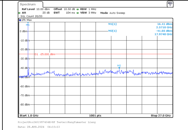
1000.0MHz-27000.0MHz Band 7 20MHz/2550.1/High QPSK 1@99 Band 7 10MHz/2564.5/High QPSK 1@0
