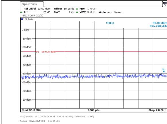
30.0MHz-1000.0MHz Band 7 20MHz/2540.2/High 256QAM 100@0 Band 7 20MHz/2560.0/High 256QAM 100@0
