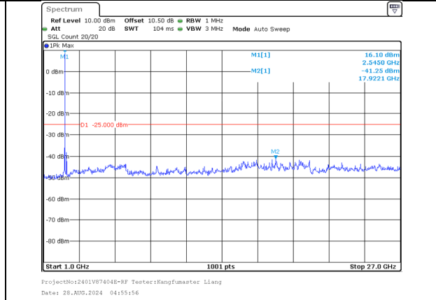
1000.0MHz-27000.0MHz Band 7 20MHz/2540.2/High QPSK 1@99 Band 7 20MHz/2560.0/High QPSK 1@0
