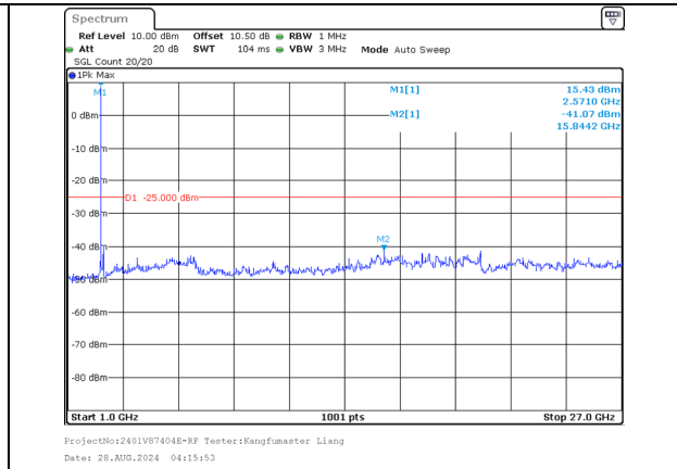
1000.0MHz-27000.0MHz Band 7 20MHz/2550.1/High 64QAM 1@99 Band 7 10MHz/2564.5/High 64QAM 1@0
