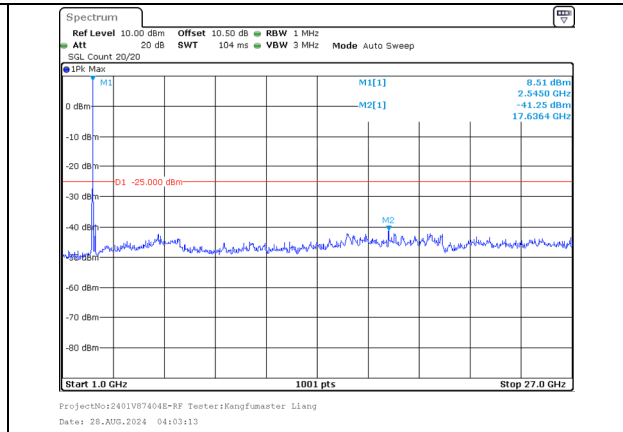
1000.0MHz-27000.0MHz Band 7 10MHz/2545.6/High 16QAM 50@0 Band 7 20MHz/2560.0/High 16QAM 100@0
