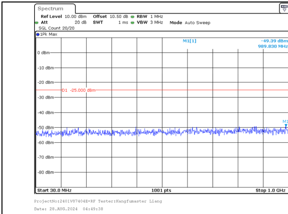
30.0MHz-1000.0MHz Band 7 20MHz/2545.1/High 64QAM 1@99 Band 7 15MHz/2562.2/High 64QAM 1@0
