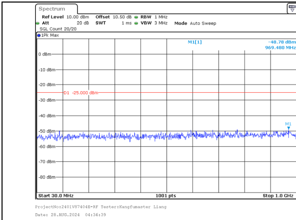
30.0MHz-1000.0MHz Band 7 15MHz/2542.9/High 16QAM 75@0 Band 7 20MHz/2560.0/High 16QAM 100@0
