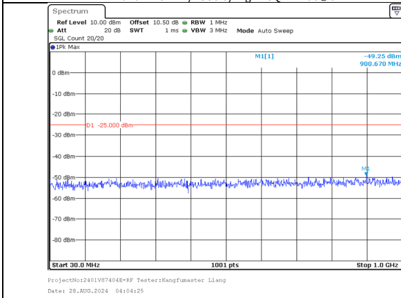
30.0MHz-1000.0MHz Band 7 10MHz/2545.6/High 64QAM 1@49 Band 7 20MHz/2560.0/High 64QAM 1@0
