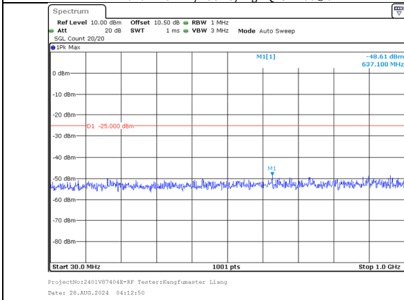
30.0MHz-1000.0MHz Band 7 20MHz/2550.1/High 16QAM 1@99 Band 7 10MHz/2564.5/High 16QAM 1@0
