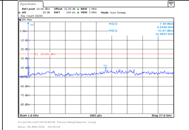
1000.0MHz-27000.0MHz Band 7 10MHz/2545.6/High 256QAM 50@0 Band 7 20MHz/2560.0/High 256QAM 100@0
