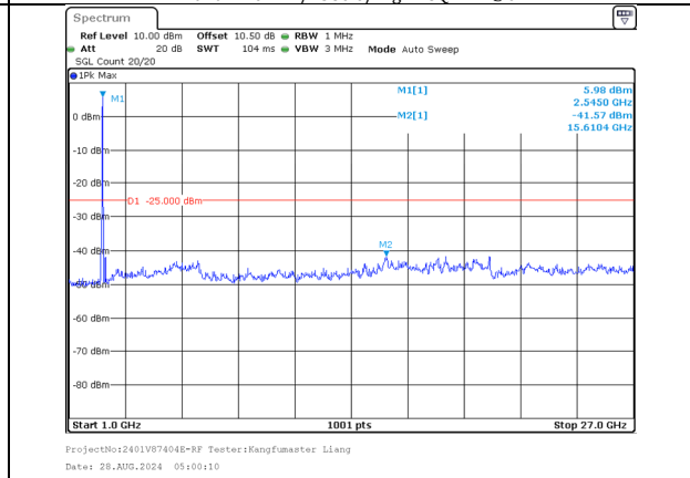
1000.0MHz-27000.0MHz Band 7 20MHz/2540.2/High 16QAM 100@0 Band 7 20MHz/2560.0/High 16QAM 100@0
