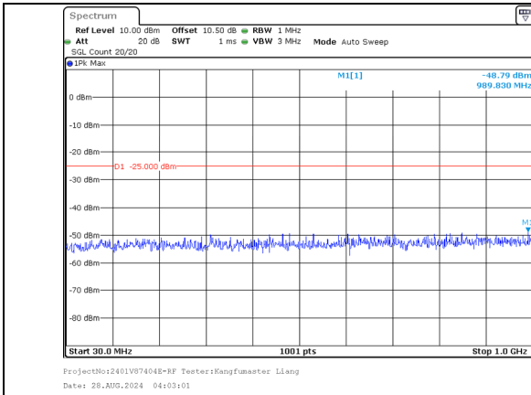
30.0MHz-1000.0MHz Band 7 10MHz/2545.6/High 16QAM 50@0 Band 7 20MHz/2560.0/High 16QAM 100@0
