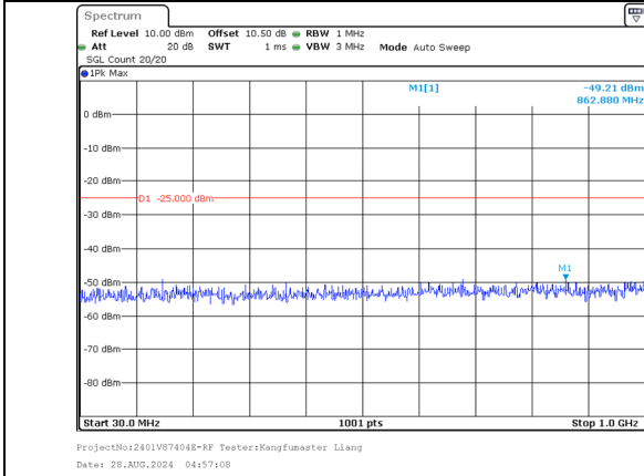
30.0MHz-1000.0MHz Band 7 20MHz/2540.2/High QPSK 100@0 Band 7 20MHz/2560.0/High QPSK 100@0
