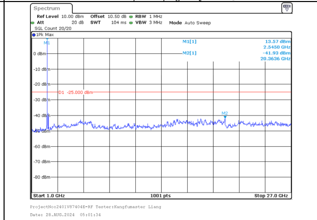
1000.0MHz-27000.0MHz Band 7 20MHz/2540.2/High 64QAM 1@99 Band 7 20MHz/2560.0/High 64QAM 1@0
