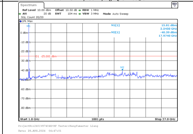
1000.0MHz-27000.0MHz Band 7 20MHz/2545.1/High 16QAM 1@99 Band 7 15MHz/2562.2/High 16QAM 1@0
