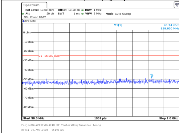
30.0MHz-1000.0MHz Band 7 20MHz/2540.2/High 64QAM 1@99 Band 7 20MHz/2560.0/High 64QAM 1@0
