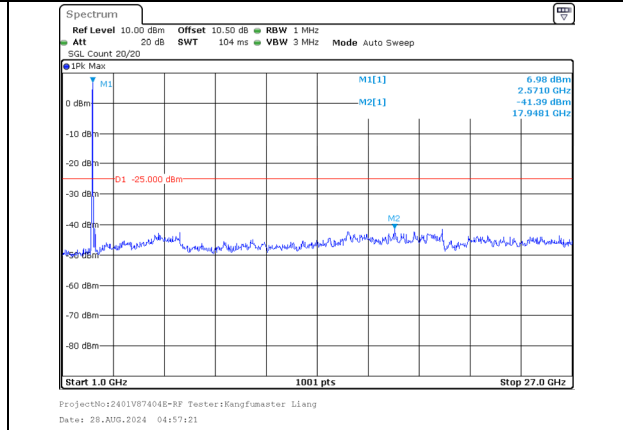
1000.0MHz-27000.0MHz Band 7 20MHz/2540.2/High QPSK 100@0 Band 7 20MHz/2560.0/High QPSK 100@0
