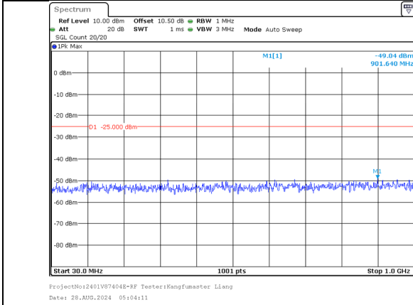
30.0MHz-1000.0MHz Band 7 20MHz/2540.2/High 256QAM 1@99 Band 7 20MHz/2560.0/High 256QAM 1@0
