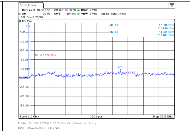
1000.0MHz-27000.0MHz Band 7 10MHz/2545.6/High 256QAM 1@49 Band 7 20MHz/2560.0/High 256QAM 1@0
