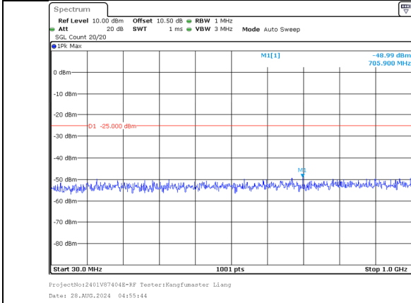
30.0MHz-1000.0MHz Band 7 20MHz/2540.2/High QPSK 1@99 Band 7 20MHz/2560.0/High QPSK 1@0
