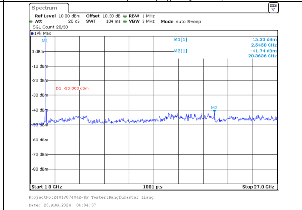
1000.0MHz-27000.0MHz Band 7 10MHz/2545.6/High 64QAM 1@49 Band 7 20MHz/2560.0/High 64QAM 1@0
