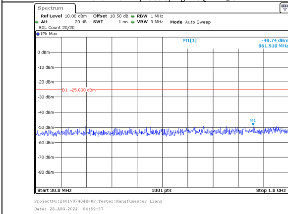
30.0MHz-1000.0MHz Band 7 20MHz/2540.2/High 16QAM 100@0 Band 7 20MHz/2560.0/High 16QAM 100@0
