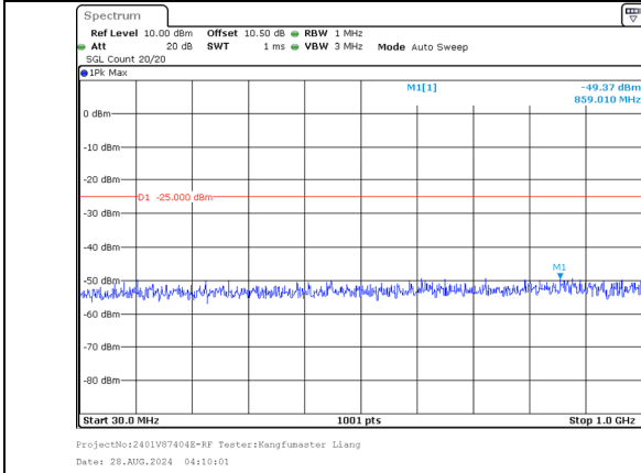
30.0MHz-1000.0MHz Band 7 20MHz/2550.1/High QPSK 1@99 Band 7 10MHz/2564.5/High QPSK 1@0
