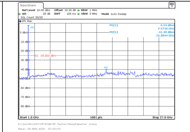
1000.0MHz-27000.0MHz Band 7 20MHz/2540.2/High 64QAM 100@0 Band 7 20MHz/2560.0/High 64QAM 100@0
