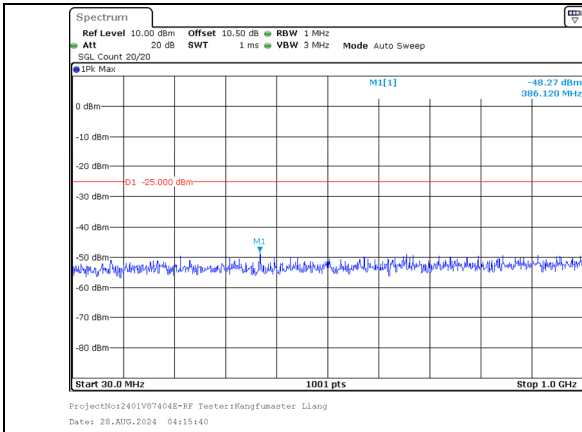
30.0MHz-1000.0MHz Band 7 20MHz/2550.1/High 64QAM 1@99 Band 7 10MHz/2564.5/High 64QAM 1@0
