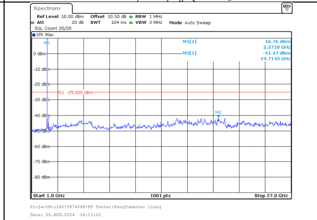
1000.0MHz-27000.0MHz Band 7 20MHz/2550.1/High 16QAM 1@99 Band 7 10MHz/2564.5/High 16QAM 1@0
