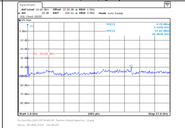
1000.0MHz-27000.0MHz Band 7 20MHz/2545.1/High 16QAM 100@0 Band 7 15MHz/2562.2/High 16QAM 100@0
