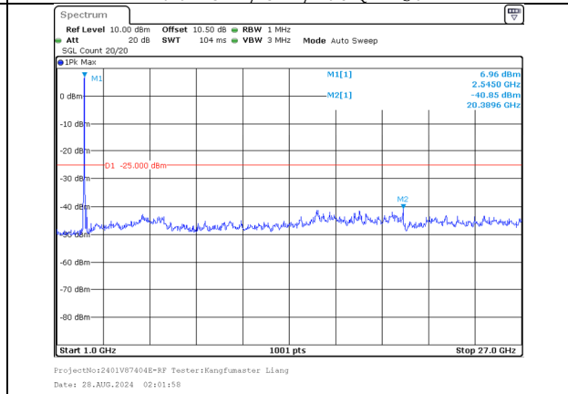
1000.0MHz-27000.0MHz Band 7 20MHz/2527.6/Mid 64QAM 100@0 Band 7 15MHz/2544.7/Mid 64QAM 100@0
