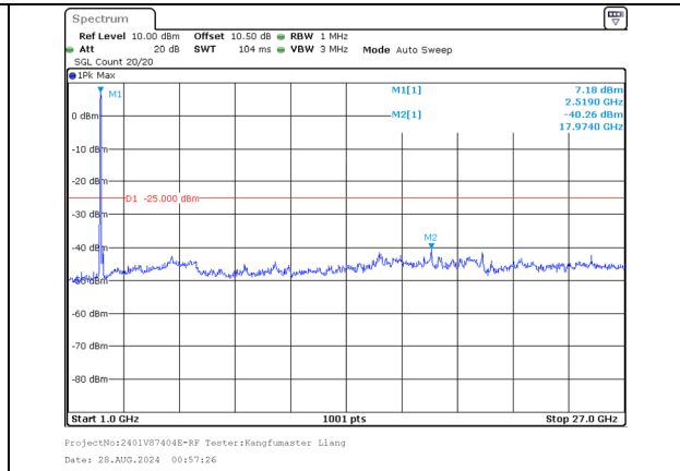
1000.0MHz-27000.0MHz Band 7 20MHz/2510.0/Low 256QAM 100@0 Band 7 15MHz/2527.1/Low 256QAM 100@0
