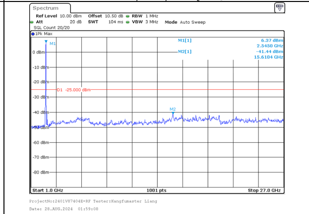
1000.0MHz-27000.0MHz Band 7 20MHz/2527.6/Mid 16QAM 100@0 Band 7 15MHz/2544.7/Mid 16QAM 100@0
