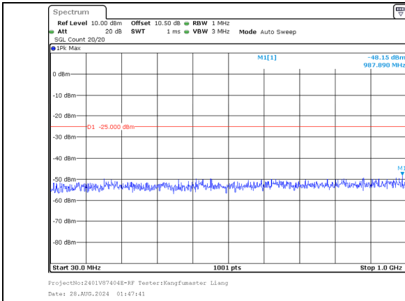
30.0MHz-1000.0MHz Band 7 15MHz/2525.3/Mid 16QAM 75@0 Band 7 20MHz/2542.4/Mid 16QAM 100@0
