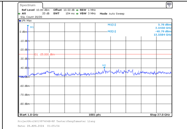
1000.0MHz-27000.0MHz Band 7 20MHz/2510.0/Low 64QAM 100@0 Band 7 20MHz/2529.8/Low 64QAM 100@0
