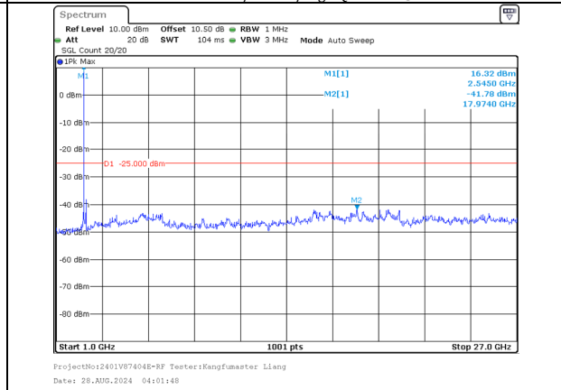
1000.0MHz-27000.0MHz Band 7 10MHz/2545.6/High 16QAM 1@49 Band 7 20MHz/2560.0/High 16QAM 1@0
