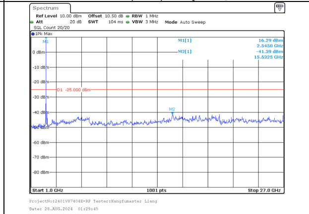
1000.0MHz-27000.0MHz Band 7 20MHz/2530.1/Mid 256QAM 1@99 Band 7 10MHz/2544.5/Mid 256QAM 1@0
