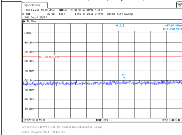
30.0MHz-1000.0MHz Band 7 20MHz/2530.1/Mid 16QAM 1@99 Band 7 10MHz/2544.5/Mid 16QAM 1@0
