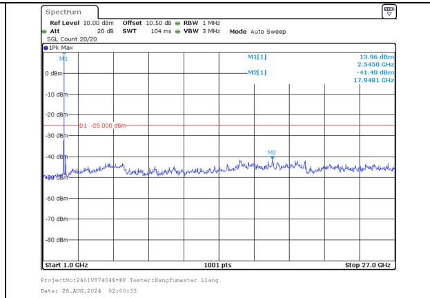
1000.0MHz-27000.0MHz Band 7 20MHz/2527.6/Mid 64QAM 1@99 Band 7 15MHz/2544.7/Mid 64QAM 1@0
