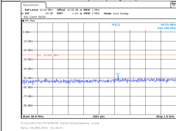
30.0MHz-1000.0MHz Band 7 15MHz/2525.3/Mid QPSK 75@0 Band 7 20MHz/2542.4/Mid QPSK 100@0
