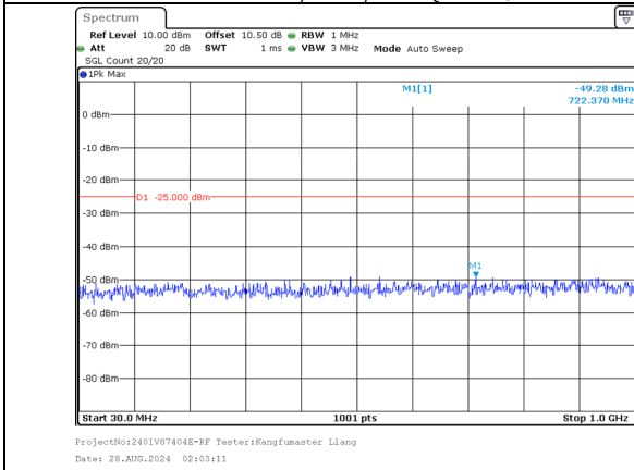
30.0MHz-1000.0MHz Band 7 20MHz/2527.6/Mid 256QAM 1@99 Band 7 15MHz/2544.7/Mid 256QAM 1@0
