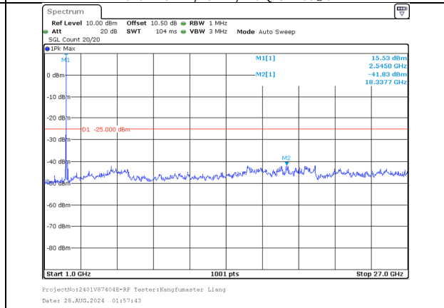
1000.0MHz-27000.0MHz Band 7 20MHz/2527.6/Mid 16QAM 1@99 Band 7 15MHz/2544.7/Mid 16QAM 1@0
