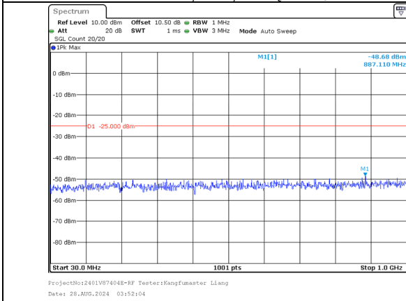
30.0MHz-1000.0MHz Band 7 20MHz/2525.1/Mid 64QAM 1@99 Band 7 20MHz/2544.9/Mid 64QAM 1@0
