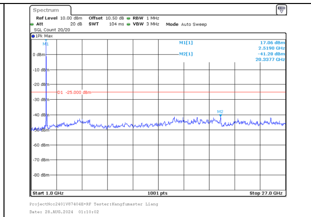
1000.0MHz-27000.0MHz Band 7 10MHz/2525.6/Mid QPSK 1@49 Band 7 20MHz/2540.0/Mid QPSK 1@0
