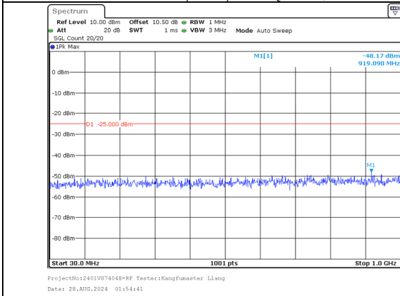
30.0MHz-1000.0MHz Band 7 20MHz/2527.6/Mid QPSK 1@99 Band 7 15MHz/2544.7/Mid QPSK 1@0
