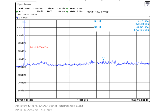
1000.0MHz-27000.0MHz Band 7 15MHz/2525.3/Mid 64QAM 1@74 Band 7 20MHz/2542.4/Mid 64QAM 1@0
