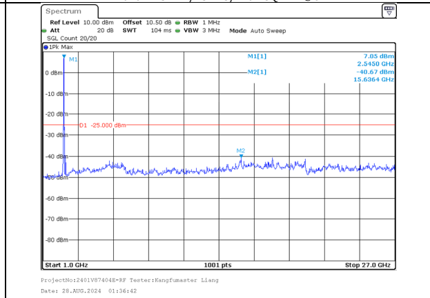
1000.0MHz-27000.0MHz Band 7 15MHz/2527.5/Mid 16QAM 75@0 Band 7 15MHz/2542.5/Mid 16QAM 75@0
