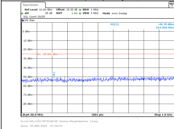
30.0MHz-1000.0MHz Band 7 20MHz/2527.6/Mid 16QAM 100@0 Band 7 15MHz/2544.7/Mid 16QAM 100@0
