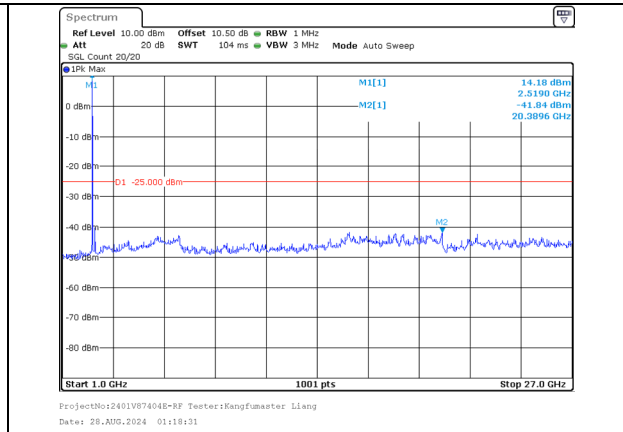
1000.0MHz-27000.0MHz Band 7 10MHz/2525.6/Mid 256QAM 1@49 Band 7 20MHz/2540.0/Mid 256QAM 1@0
