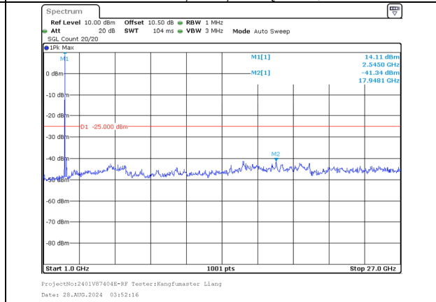
1000.0MHz-27000.0MHz Band 7 20MHz/2525.1/Mid 64QAM 1@99 Band 7 20MHz/2544.9/Mid 64QAM 1@0
