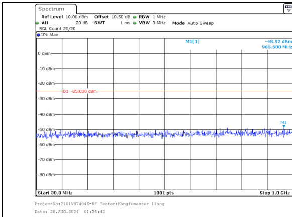
30.0MHz-1000.0MHz Band 7 20MHz/2530.1/Mid 64QAM 1@99 Band 7 10MHz/2544.5/Mid 64QAM 1@0
