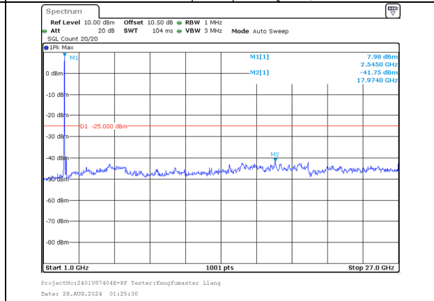
1000.0MHz-27000.0MHz Band 7 20MHz/2530.1/Mid 16QAM 100@0 Band 7 10MHz/2544.5/Mid 16QAM 100@0
