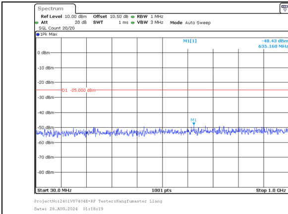
30.0MHz-1000.0MHz Band 7 10MHz/2525.6/Mid 256QAM 1@49 Band 7 20MHz/2540.0/Mid 256QAM 1@0
