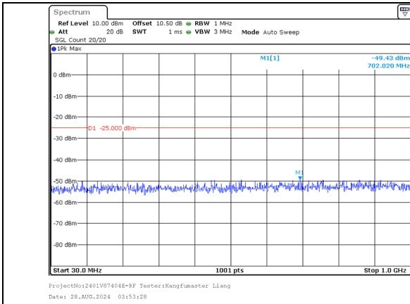
30.0MHz-1000.0MHz Band 7 20MHz/2525.1/Mid 64QAM 100@0 Band 7 20MHz/2544.9/Mid 64QAM 100@0
