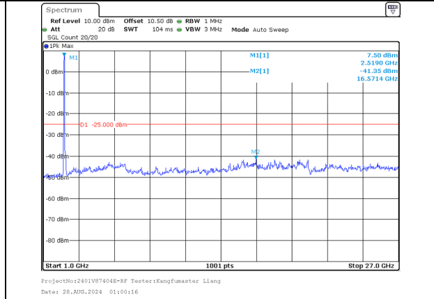
1000.0MHz-27000.0MHz Band 7 20MHz/2510.0/Low QPSK 100@0 Band 7 20MHz/2529.8/Low QPSK 100@0
