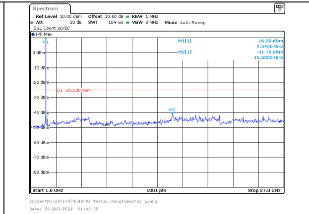
1000.0MHz-27000.0MHz Band 7 15MHz/2525.3/Mid QPSK 1@74 Band 7 20MHz/2542.4/Mid QPSK 1@0
