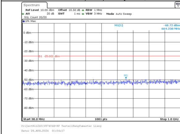
30.0MHz-1000.0MHz Band 7 20MHz/2510.0/Low 64QAM 1@99 Band 7 20MHz/2529.8/Low 64QAM 1@0
