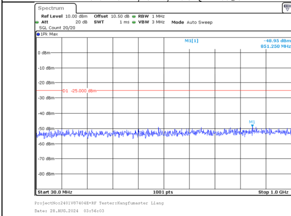
30.0MHz-1000.0MHz Band 7 20MHz/2525.1/Mid 256QAM 1@99 Band 7 20MHz/2544.9/Mid 256QAM 1@0
