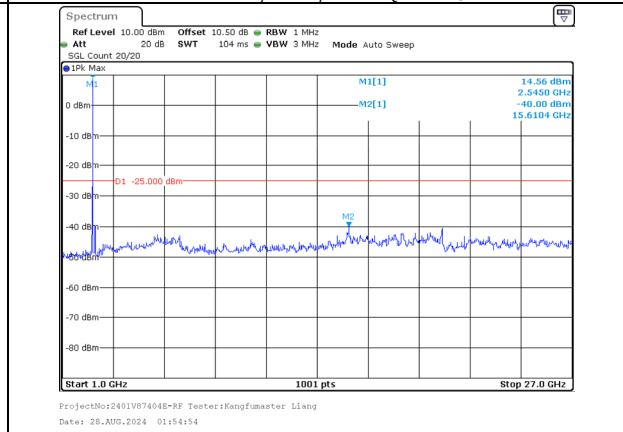
1000.0MHz-27000.0MHz Band 7 20MHz/2527.6/Mid QPSK 1@99 Band 7 15MHz/2544.7/Mid QPSK 1@0
