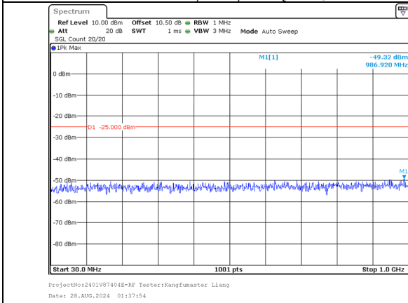
30.0MHz-1000.0MHz Band 7 15MHz/2527.5/Mid 64QAM 1@74 Band 7 15MHz/2542.5/Mid 64QAM 1@0
