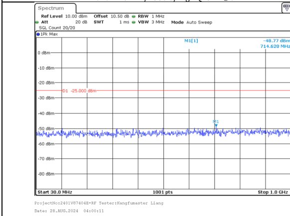
30.0MHz-1000.0MHz Band 7 10MHz/2545.6/High QPSK 50@0 Band 7 20MHz/2560.0/High QPSK 100@0
