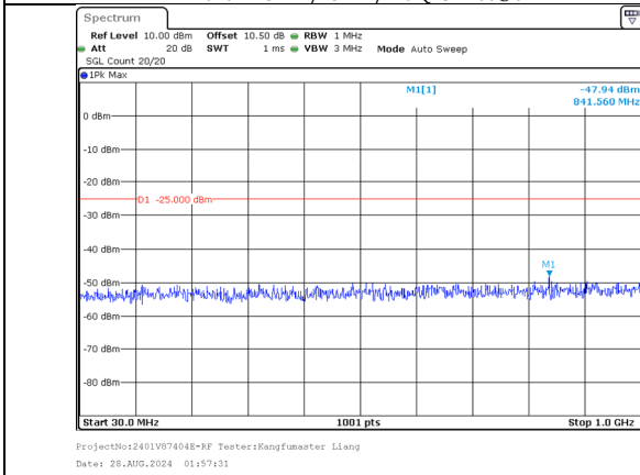
30.0MHz-1000.0MHz Band 7 20MHz/2527.6/Mid 16QAM 1@99 Band 7 15MHz/2544.7/Mid 16QAM 1@0
