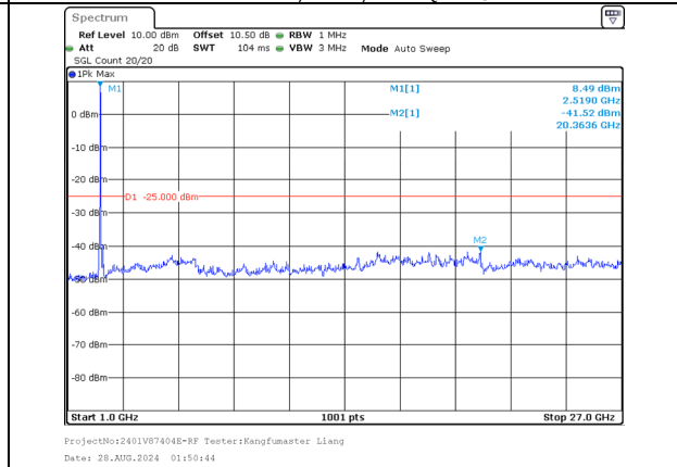
1000.0MHz-27000.0MHz Band 7 15MHz/2525.3/Mid 64QAM 75@0 Band 7 20MHz/2542.4/Mid 64QAM 100@0
