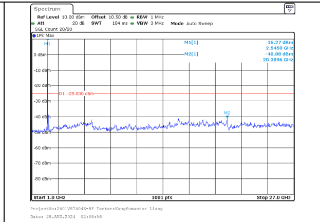
1000.0MHz-27000.0MHz Band 7 20MHz/2525.1/Mid 16QAM 1@99 Band 7 20MHz/2544.9/Mid 16QAM 1@0
