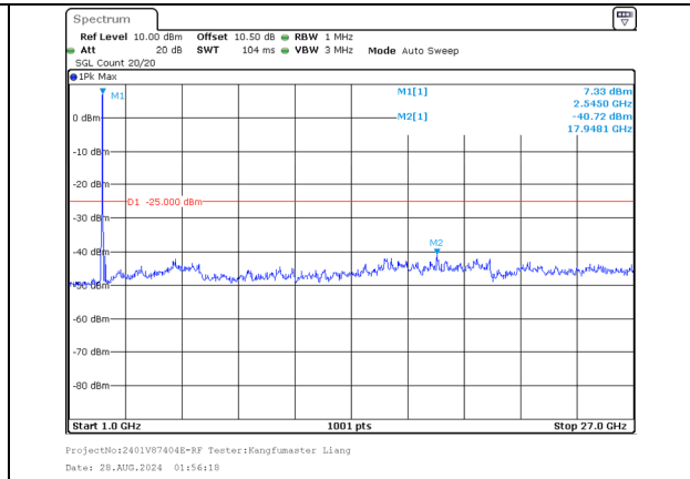
1000.0MHz-27000.0MHz Band 7 20MHz/2527.6/Mid QPSK 100@0 Band 7 15MHz/2544.7/Mid QPSK 100@0
