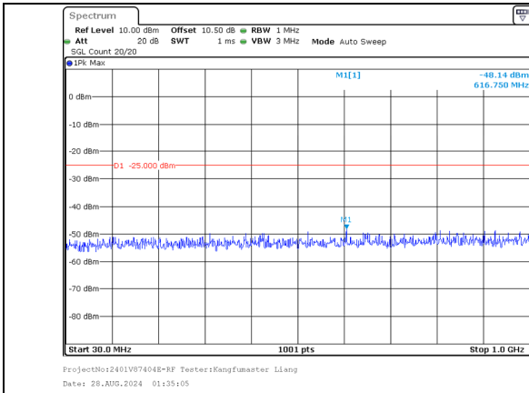
30.0MHz-1000.0MHz Band 7 15MHz/2527.5/Mid 16QAM 1@74 Band 7 15MHz/2542.5/Mid 16QAM 1@0
