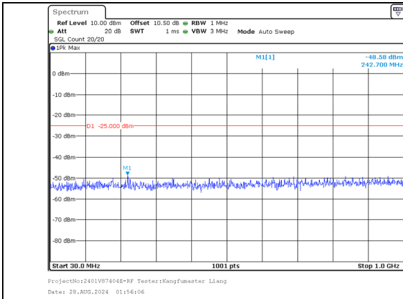
30.0MHz-1000.0MHz Band 7 20MHz/2527.6/Mid QPSK 100@0 Band 7 15MHz/2544.7/Mid QPSK 100@0
