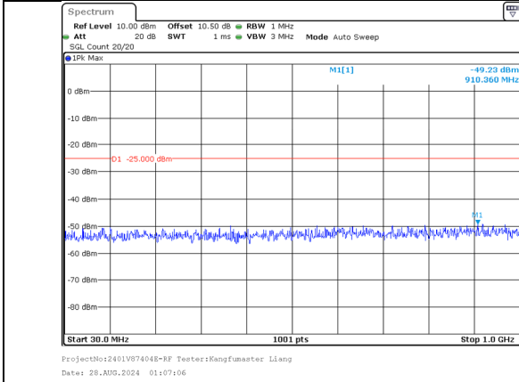
30.0MHz-1000.0MHz Band 7 20MHz/2510.0/Low 256QAM 1@99 Band 7 20MHz/2529.8/Low 256QAM 1@0
