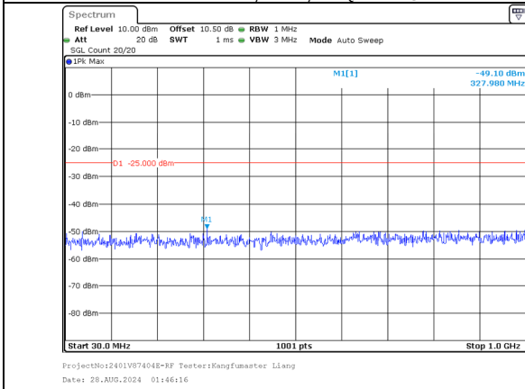
30.0MHz-1000.0MHz Band 7 15MHz/2525.3/Mid 16QAM 1@74 Band 7 20MHz/2542.4/Mid 16QAM 1@0
