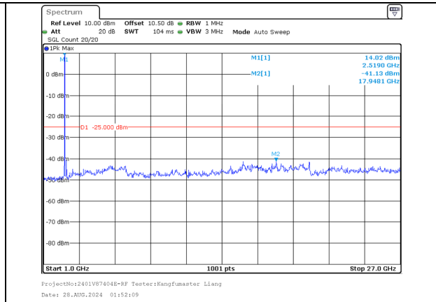
1000.0MHz-27000.0MHz Band 7 15MHz/2525.3/Mid 256QAM 1@74 Band 7 20MHz/2542.4/Mid 256QAM 1@0
