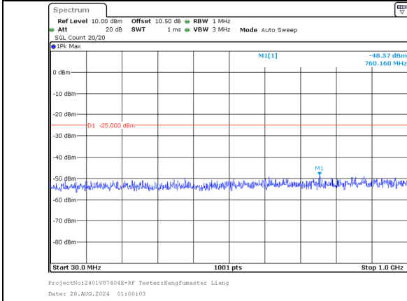
30.0MHz-1000.0MHz Band 7 20MHz/2510.0/Low QPSK 100@0 Band 7 20MHz/2529.8/Low QPSK 100@0
