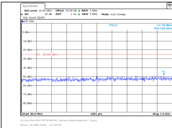
30.0MHz-1000.0MHz Band 7 10MHz/2525.6/Mid QPSK 1@49 Band 7 20MHz/2540.0/Mid QPSK 1@0
