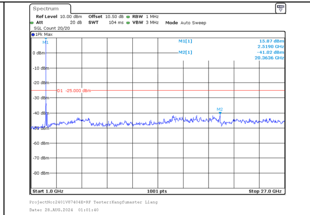
1000.0MHz-27000.0MHz Band 7 20MHz/2510.0/Low 16QAM 1@99 Band 7 20MHz/2529.8/Low 16QAM 1@0
