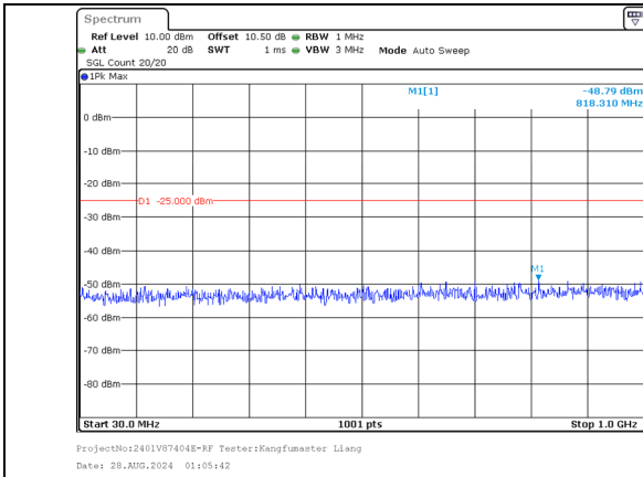
30.0MHz-1000.0MHz Band 7 20MHz/2510.0/Low 64QAM 100@0 Band 7 20MHz/2529.8/Low 64QAM 100@0
