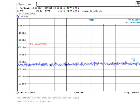
30.0MHz-1000.0MHz Band 7 20MHz/2527.6/Mid 256QAM 100@0 Band 7 15MHz/2544.7/Mid 256QAM 100@0
