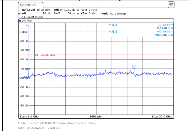
1000.0MHz-27000.0MHz Band 7 20MHz/2530.1/Mid QPSK 1@99 Band 7 10MHz/2544.5/Mid QPSK 1@0
