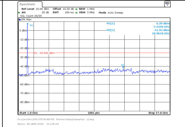
1000.0MHz-27000.0MHz Band 7 20MHz/2510.0/Low 256QAM 100@0 Band 7 20MHz/2529.8/Low 256QAM 100@0
