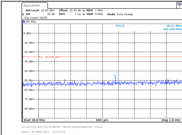
30.0MHz-1000.0MHz Band 7 15MHz/2525.3/Mid 256QAM 1@74 Band 7 20MHz/2542.4/Mid 256QAM 1@0
