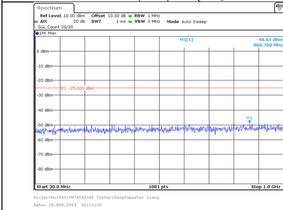
30.0MHz-1000.0MHz Band 7 20MHz/2525.1/Mid 16QAM 100@0 Band 7 20MHz/2544.9/Mid 16QAM 100@0
