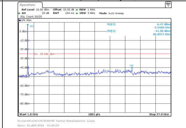
1000.0MHz-27000.0MHz Band 7 15MHz/2527.5/Mid 256QAM 75@0 Band 7 15MHz/2542.5/Mid 256QAM 75@0
