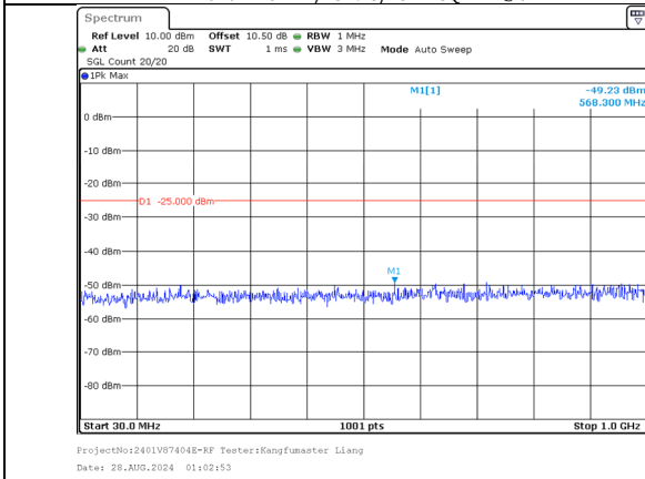
30.0MHz-1000.0MHz Band 7 20MHz/2510.0/Low 16QAM 100@0 Band 7 20MHz/2529.8/Low 16QAM 100@0
