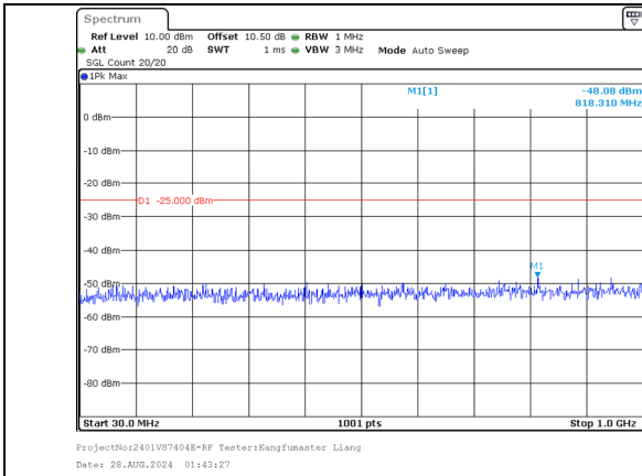
30.0MHz-1000.0MHz Band 7 15MHz/2525.3/Mid QPSK 1@74 Band 7 20MHz/2542.4/Mid QPSK 1@0
