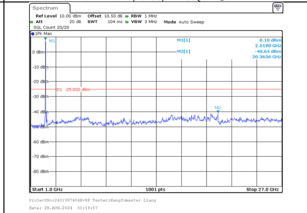
1000.0MHz-27000.0MHz Band 7 10MHz/2525.6/Mid 256QAM 50@0 Band 7 20MHz/2540.0/Mid 256QAM 100@0
