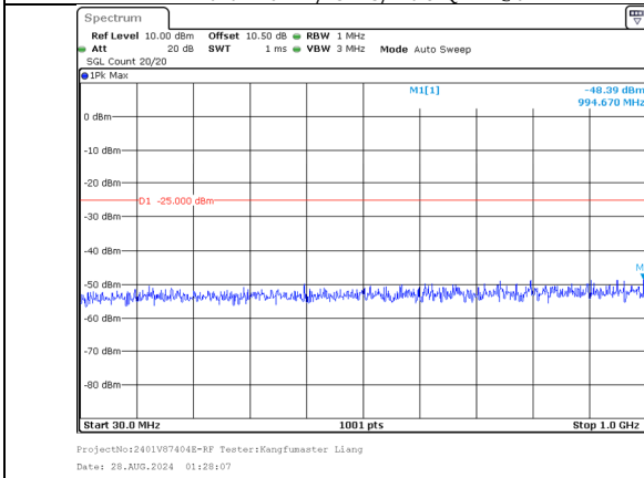
30.0MHz-1000.0MHz Band 7 20MHz/2530.1/Mid 64QAM 100@0 Band 7 10MHz/2544.5/Mid 64QAM 100@0
