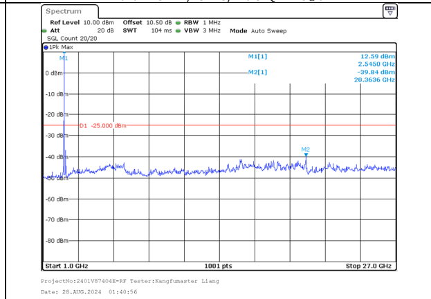
1000.0MHz-27000.0MHz Band 7 15MHz/2527.5/Mid 256QAM 1@74 Band 7 15MHz/2542.5/Mid 256QAM 1@0
