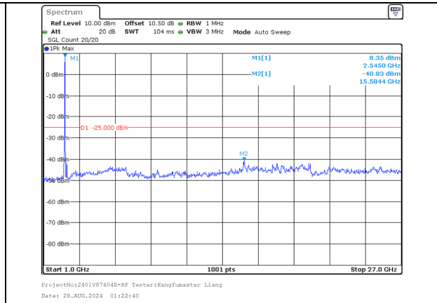
1000.0MHz-27000.0MHz Band 7 20MHz/2530.1/Mid QPSK 100@0 Band 7 10MHz/2544.5/Mid QPSK 100@0
