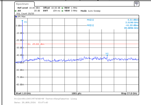
1000.0MHz-27000.0MHz Band 7 20MHz/2525.1/Mid 256QAM 100@0 Band 7 20MHz/2544.9/Mid 256QAM 100@0
