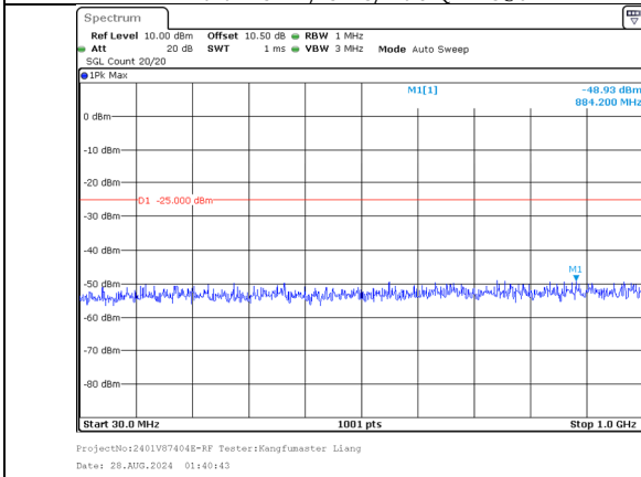
30.0MHz-1000.0MHz Band 7 15MHz/2527.5/Mid 256QAM 1@74 Band 7 15MHz/2542.5/Mid 256QAM 1@0
