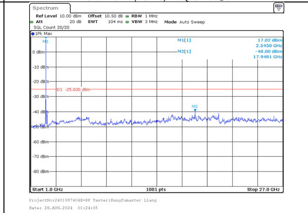
1000.0MHz-27000.0MHz Band 7 20MHz/2530.1/Mid 16QAM 1@99 Band 7 10MHz/2544.5/Mid 16QAM 1@0
