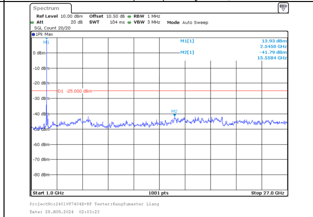
1000.0MHz-27000.0MHz Band 7 20MHz/2527.6/Mid 256QAM 1@99 Band 7 15MHz/2544.7/Mid 256QAM 1@0
