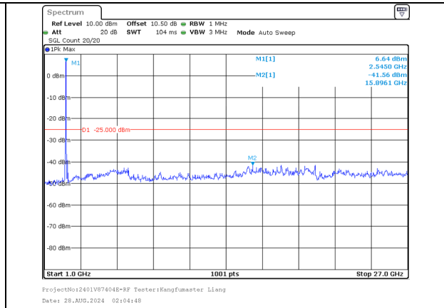
1000.0MHz-27000.0MHz Band 7 20MHz/2527.6/Mid 256QAM 100@0 Band 7 15MHz/2544.7/Mid 256QAM 100@0
