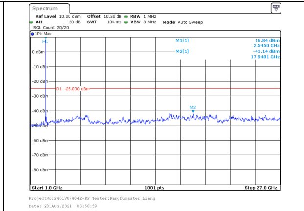
1000.0MHz-27000.0MHz Band 7 10MHz/2545.6/High QPSK 1@49 Band 7 20MHz/2560.0/High QPSK 1@0
