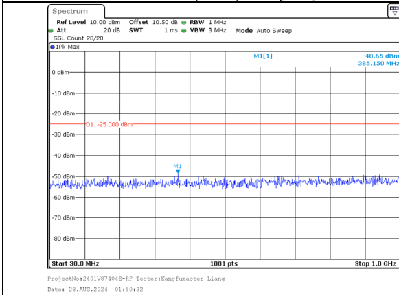
30.0MHz-1000.0MHz Band 7 15MHz/2525.3/Mid 64QAM 75@0 Band 7 20MHz/2542.4/Mid 64QAM 100@0
