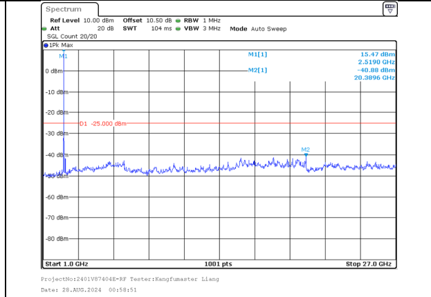
1000.0MHz-27000.0MHz Band 7 20MHz/2510.0/Low QPSK 1@99 Band 7 20MHz/2529.8/Low QPSK 1@0
