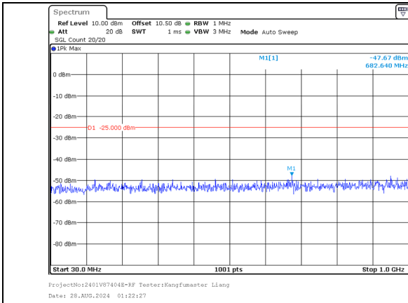
30.0MHz-1000.0MHz Band 7 20MHz/2530.1/Mid QPSK 100@0 Band 7 10MHz/2544.5/Mid QPSK 100@0
