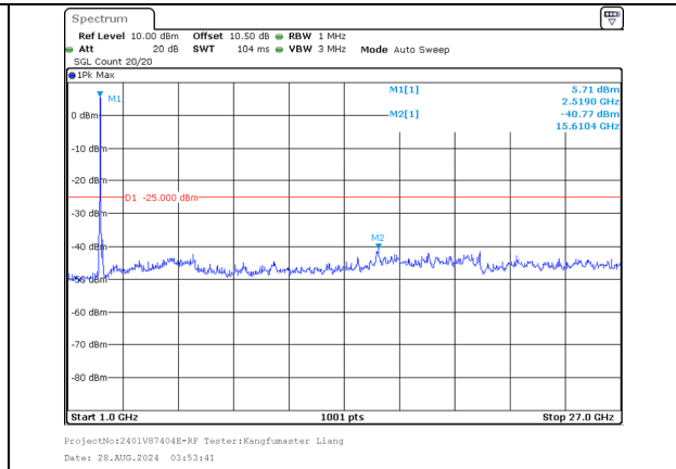
1000.0MHz-27000.0MHz Band 7 20MHz/2525.1/Mid 64QAM 100@0 Band 7 20MHz/2544.9/Mid 64QAM 100@0
