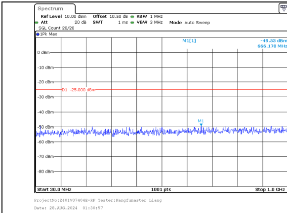
30.0MHz-1000.0MHz Band 7 20MHz/2530.1/Mid 256QAM 100@0 Band 7 10MHz/2544.5/Mid 256QAM 100@0
