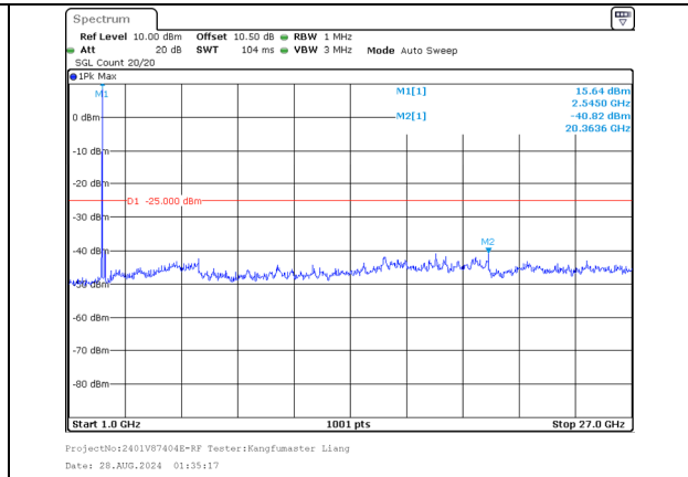
1000.0MHz-27000.0MHz Band 7 15MHz/2527.5/Mid 16QAM 1@74 Band 7 15MHz/2542.5/Mid 16QAM 1@0
