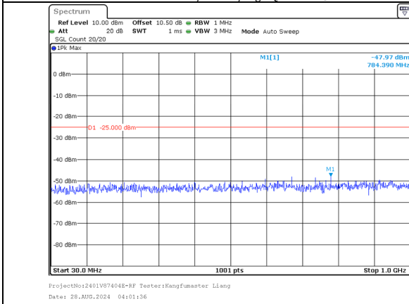
30.0MHz-1000.0MHz Band 7 10MHz/2545.6/High 16QAM 1@49 Band 7 20MHz/2560.0/High 16QAM 1@0
