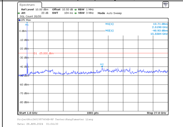
1000.0MHz-27000.0MHz Band 7 20MHz/2510.0/Low 64QAM 1@99 Band 7 20MHz/2529.8/Low 64QAM 1@0
