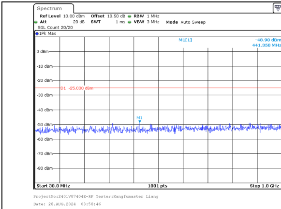
30.0MHz-1000.0MHz Band 7 10MHz/2545.6/High QPSK 1@49 Band 7 20MHz/2560.0/High QPSK 1@0
