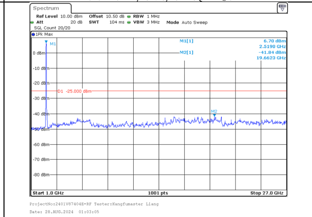
1000.0MHz-27000.0MHz Band 7 20MHz/2510.0/Low 16QAM 100@99 Band 7 20MHz/2529.8/Low 16QAM 100@0
