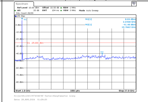
1000.0MHz-27000.0MHz Band 7 20MHz/2530.1/Mid 64QAM 100@0 Band 7 10MHz/2544.5/Mid 64QAM 100@0
