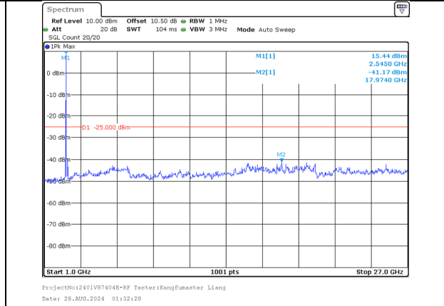
1000.0MHz-27000.0MHz Band 7 15MHz/2527.5/Mid QPSK 1@74 Band 7 15MHz/2542.5/Mid QPSK 1@0
