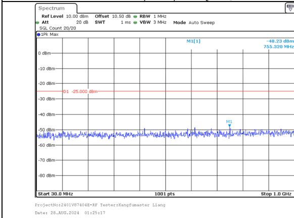
30.0MHz-1000.0MHz Band 7 20MHz/2530.1/Mid 16QAM 100@0 Band 7 10MHz/2544.5/Mid 16QAM 100@0
