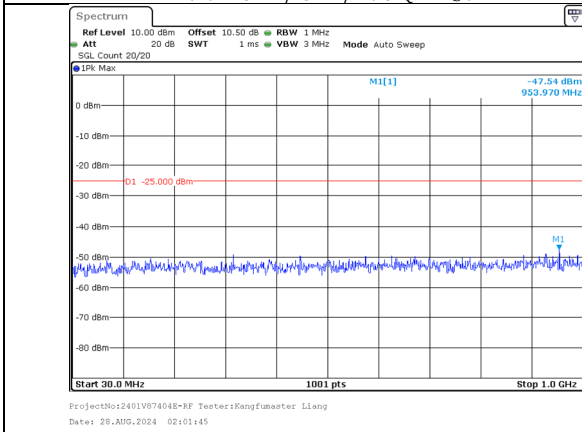
30.0MHz-1000.0MHz Band 7 20MHz/2527.6/Mid 64QAM 100@0 Band 7 15MHz/2544.7/Mid 64QAM 100@0
