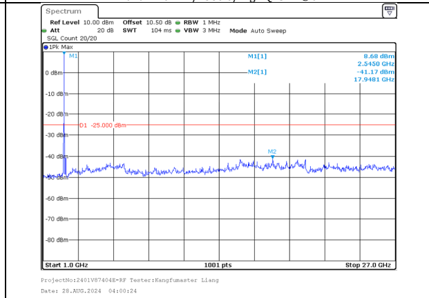
1000.0MHz-27000.0MHz Band 7 10MHz/2545.6/High QPSK 50@0 Band 7 20MHz/2560.0/High QPSK 100@0
