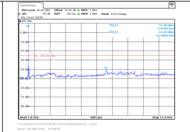
1000.0MHz-27000.0MHz Band 7 20MHz/2530.1/Mid 64QAM 1@99 Band 7 10MHz/2544.5/Mid 64QAM 1@0
