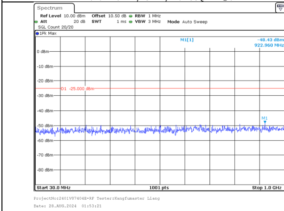
30.0MHz-1000.0MHz Band 7 15MHz/2525.3/Mid 256QAM 75@0 Band 7 20MHz/2542.4/Mid 256QAM 100@0
