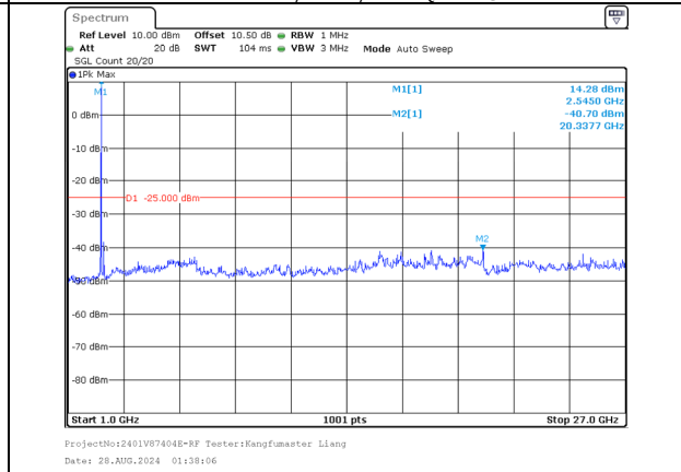
1000.0MHz-27000.0MHz Band 7 15MHz/2527.5/Mid 64QAM 1@74 Band 7 15MHz/2542.5/Mid 64QAM 1@0
