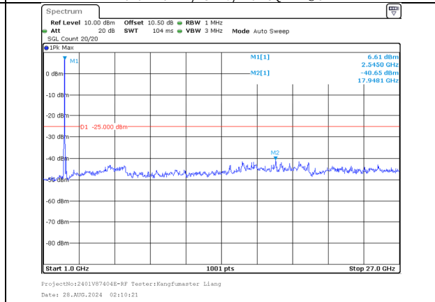
1000.0MHz-27000.0MHz Band 7 20MHz/2525.1/Mid 16QAM 100@0 Band 7 20MHz/2544.9/Mid 16QAM 100@0
