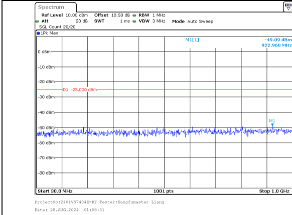
30.0MHz-1000.0MHz Band 7 20MHz/2510.0/Low 256QAM 100@0 Band 7 20MHz/2529.8/Low 256QAM 100@0
