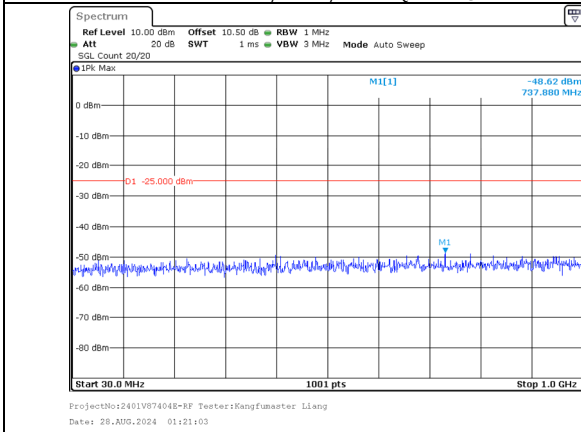
30.0MHz-1000.0MHz Band 7 20MHz/2530.1/Mid QPSK 1@99 Band 7 10MHz/2544.5/Mid QPSK 1@0
