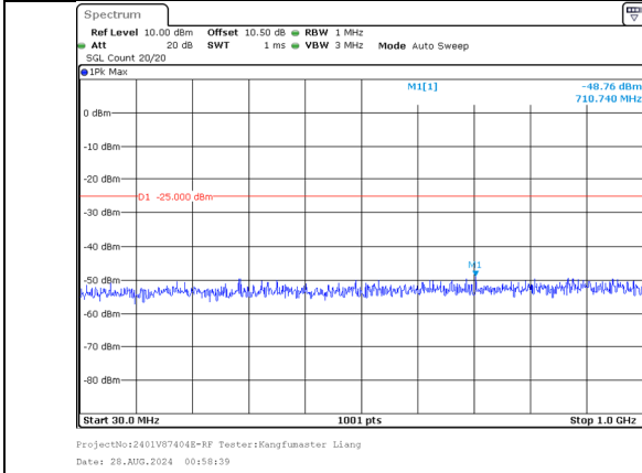
30.0MHz-1000.0MHz Band 7 20MHz/2510.0/Low QPSK 1@99 Band 7 20MHz/2529.8/Low QPSK 1@0
