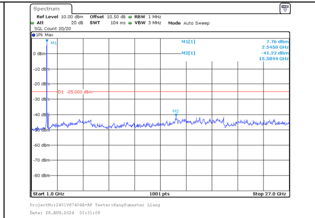
1000.0MHz-27000.0MHz Band 7 20MHz/2530.1/Mid 256QAM 100@0 Band 7 10MHz/2544.5/Mid 256QAM 100@0
