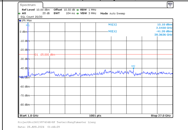
1000.0MHz-27000.0MHz Band 7 15MHz/2525.3/Mid 16QAM 1@74 Band 7 20MHz/2542.4/Mid 16QAM 1@0
