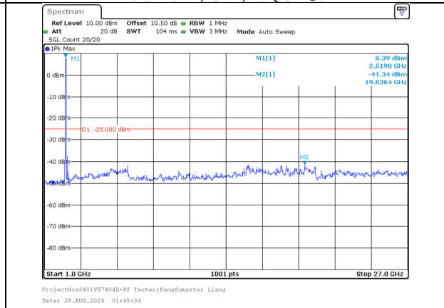
1000.0MHz-27000.0MHz Band 7 15MHz/2525.3/Mid QPSK 75@0 Band 7 20MHz/2542.4/Mid QPSK 100@0
