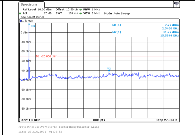
1000.0MHz-27000.0MHz Band 7 15MHz/2527.5/Mid QPSK 75@0 Band 7 15MHz/2542.5/Mid QPSK 75@0
