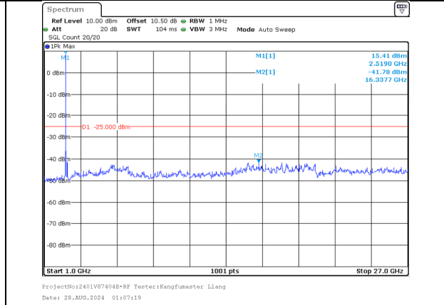
1000.0MHz-27000.0MHz Band 7 20MHz/2510.0/Low 256QAM 1@99 Band 7 20MHz/2529.8/Low 256QAM 1@0
