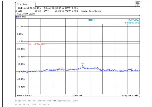
1000.0MHz-10000.0MHz Band 5 10MHz/839.0/High 64QAM 1@49 Band 5 5MHz/846.2/High 64QAM 1@0
