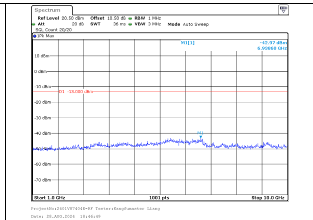
1000.0MHz-10000.0MHz Band 5 5MHz/835.0/Mid 256QAM 1@24 Band 5 3MHz/838.9/Mid 256QAM 1@0
