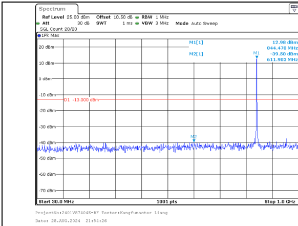
30.0MHz-1000.0MHz Band 5 10MHz/839.0/High 64QAM 1@49 Band 5 5MHz/846.2/High 64QAM 1@0
