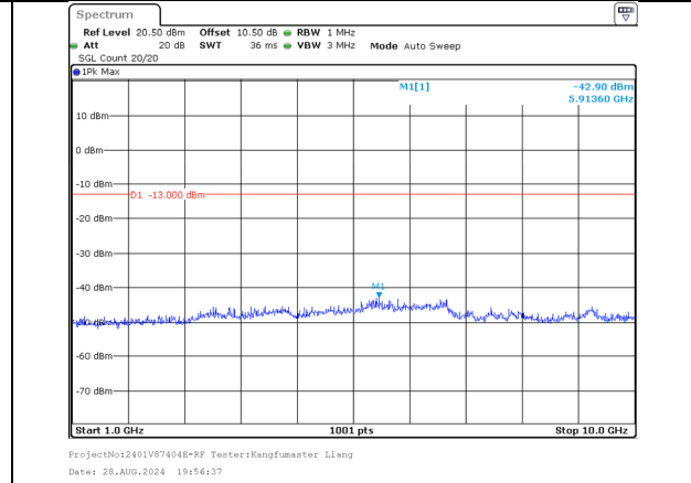
1000.0MHz-10000.0MHz Band 5 10MHz/834.0/Mid QPSK 1@49 Band 5 5MHz/841.2/Mid QPSK 1@0
