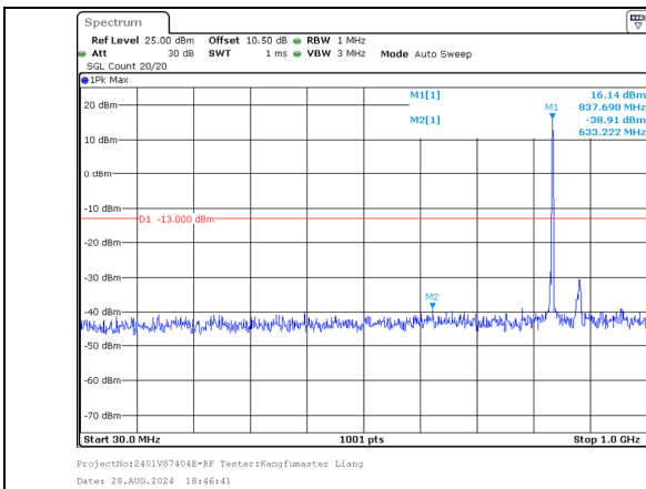
30.0MHz-1000.0MHz Band 5 5MHz/835.0/Mid 256QAM 1@24 Band 5 3MHz/838.9/Mid 256QAM 1@0
