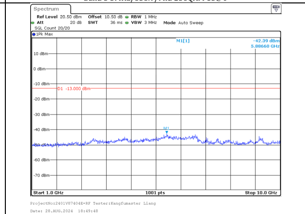
1000.0MHz-10000.0MHz Band 5 5MHz/831.8/Mid QPSK 1@24 Band 5 10MHz/839.0/Mid QPSK 1@0
