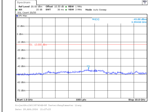
1000.0MHz-10000.0MHz Band 5 5MHz/843.5/High QPSK 1@24 Band 5 3MHz/847.4/High QPSK 1@0
