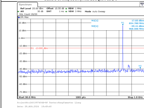
30.0MHz-1000.0MHz Band 5 5MHz/831.8/Mid QPSK 1@24 Band 5 10MHz/839.0/Mid QPSK 1@0
