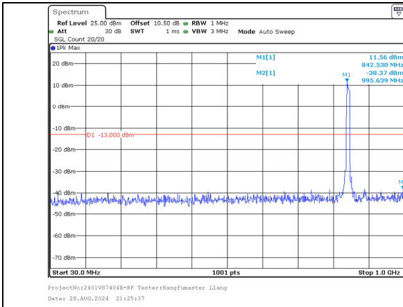
30.0MHz-1000.0MHz Band 5 3MHz/842.6/High 256QAM 15@0 Band 5 5MHz/846.5/High 256QAM 25@0
