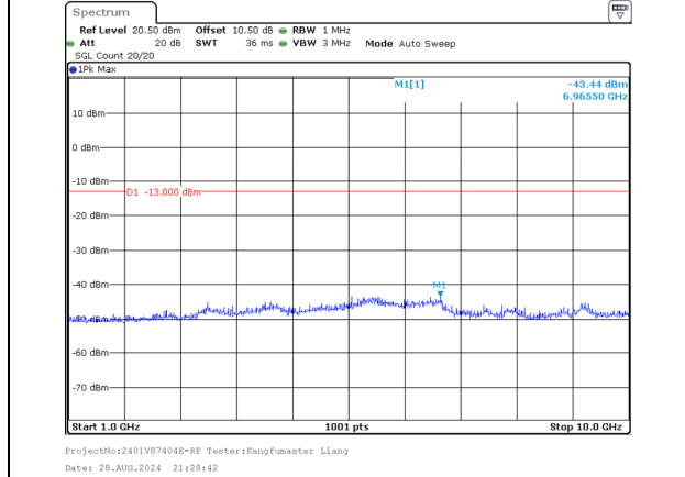
1000.0MHz-10000.0MHz Band 5 5MHz/843.5/High QPSK 25@0 Band 5 3MHz/847.4/High QPSK 15@0
