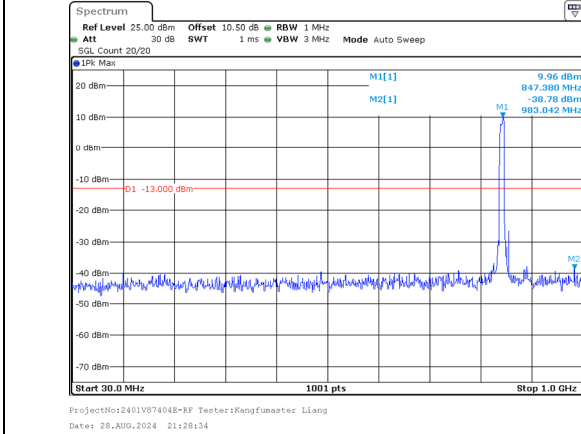
30.0MHz-1000.0MHz Band 5 5MHz/843.5/High QPSK 25@0 Band 5 3MHz/847.4/High QPSK 15@0
