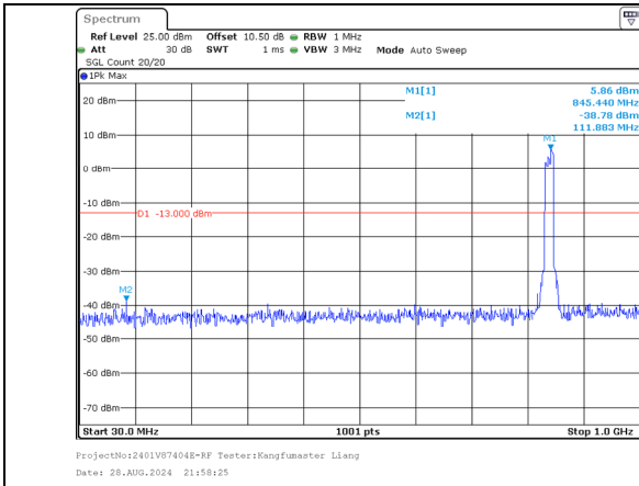
30.0MHz-1000.0MHz Band 5 10MHz/839.0/High 256QAM 50@0 Band 5 5MHz/846.2/High 256QAM 25@0
