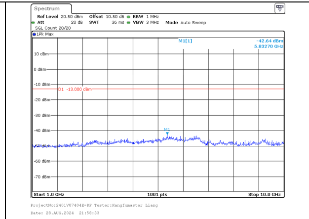
1000.0MHz-10000.0MHz Band 5 10MHz/839.0/High 256QAM 50@0 Band 5 5MHz/846.2/High 256QAM 25@0
