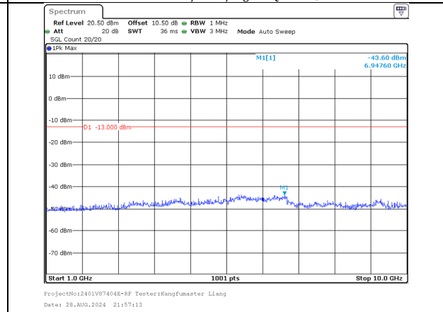
1000.0MHz-10000.0MHz Band 5 10MHz/839.0/High 256QAM 1@49 Band 5 5MHz/846.2/High 256QAM 1@0
