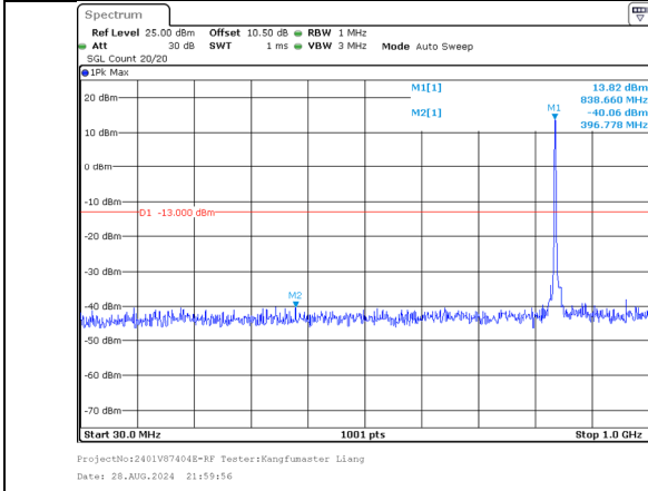
30.0MHz-1000.0MHz Band 5 10MHz/834.1/High QPSK 1@49 Band 5 10MHz/844.0/High QPSK 1@0
