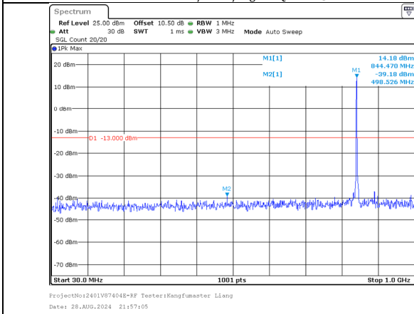
30.0MHz-1000.0MHz Band 5 10MHz/839.0/High 256QAM 1@49 Band 5 5MHz/846.2/High 256QAM 1@0
