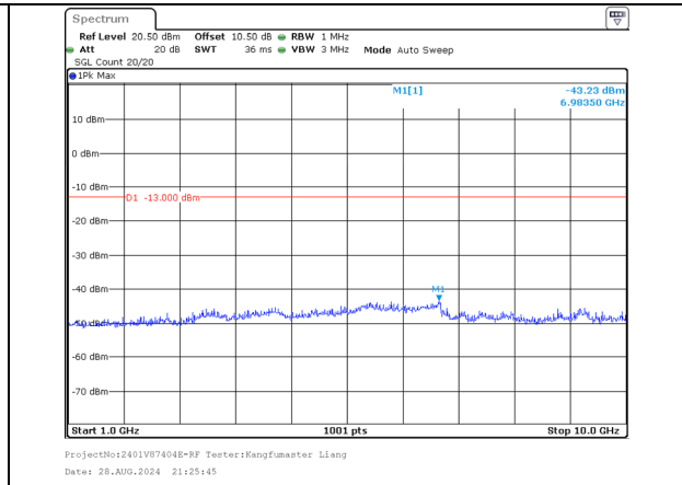
1000.0MHz-10000.0MHz Band 5 3MHz/842.6/High 256QAM 15@0 Band 5 5MHz/846.5/High 256QAM 25@0
