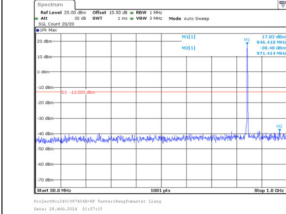
30.0MHz-1000.0MHz Band 5 5MHz/843.5/High QPSK 1@24 Band 5 3MHz/847.4/High QPSK 1@0
