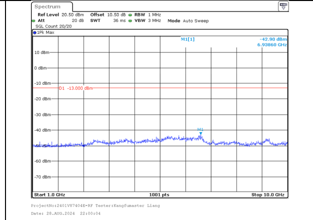
1000.0MHz-10000.0MHz Band 5 10MHz/834.1/High QPSK 1@49 Band 5 10MHz/844.0/High QPSK 1@0
