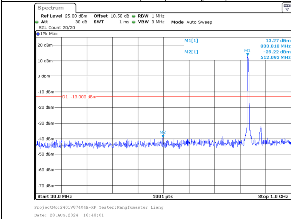
30.0MHz-1000.0MHz Band 5 5MHz/835.0/Mid 256QAM 25@0 Band 5 3MHz/838.9/Mid 256QAM 15@0
