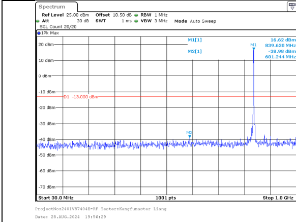
30.0MHz-1000.0MHz Band 5 10MHz/834.0/Mid QPSK 1@49 Band 5 5MHz/841.2/Mid QPSK 1@0
