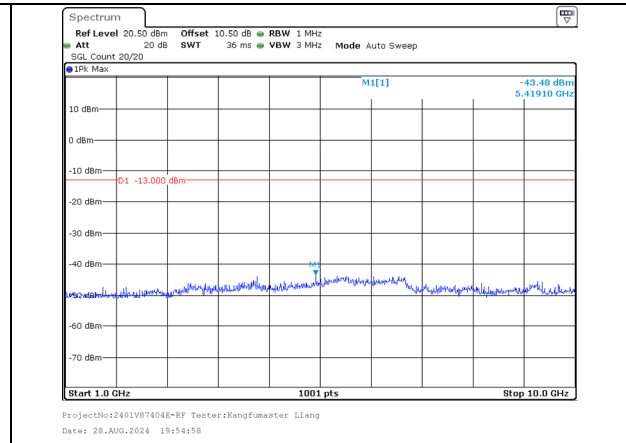
1000.0MHz-10000.0MHz Band 5 5MHz/831.8/Mid 256QAM 25@0 Band 5 10MHz/839.0/Mid 256QAM 50@0
