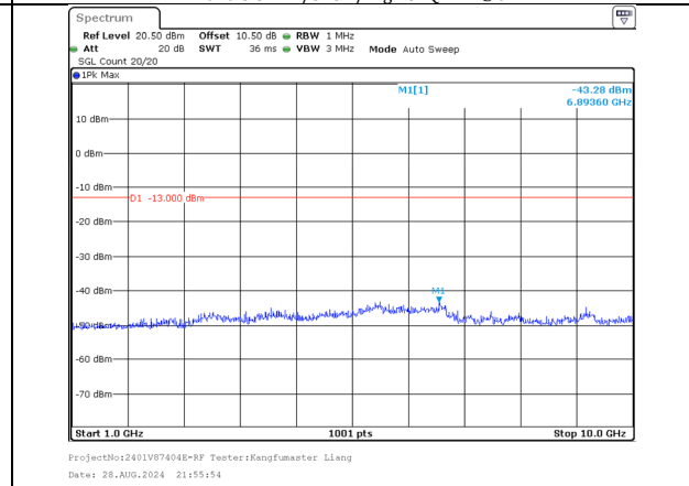
1000.0MHz-10000.0MHz Band 5 10MHz/839.0/High 64QAM 50@0 Band 5 5MHz/846.2/High 64QAM 25@0
