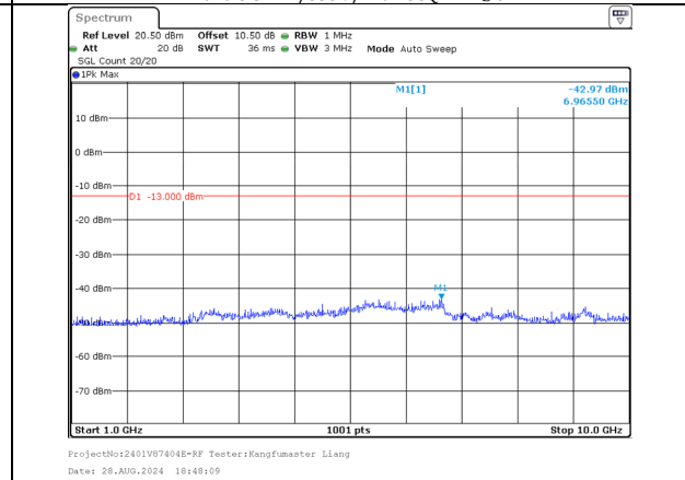
1000.0MHz-10000.0MHz Band 5 5MHz/835.0/Mid 256QAM 25@0 Band 5 3MHz/838.9/Mid 256QAM 15@0
