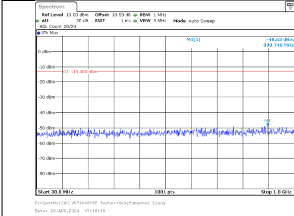
30.0MHz-1000.0MHz Band 66 15MHz/1745.3/Mid 256QAM 1@74 Band 66 20MHz/1762.4/Mid 256QAM 1@0
