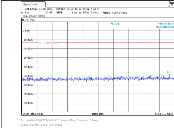
30.0MHz-1000.0MHz Band 66 15MHz/1747.5/Mid QPSK 1@74 Band 66 15MHz/1762.5/Mid QPSK 1@0
