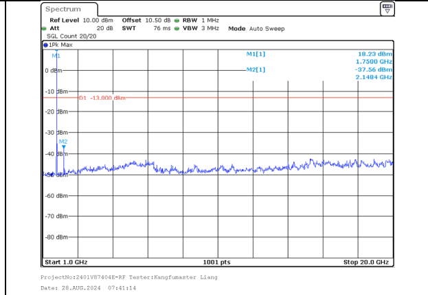
1000.0MHz-20000.0MHz Band 66 5MHz/1745.8/Mid QPSK 1@24 Band 66 20MHz/1757.5/Mid QPSK 1@0
