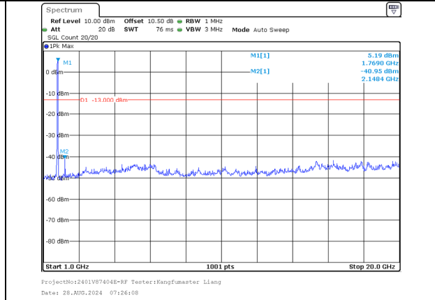
1000.0MHz-20000.0MHz Band 66 20MHz/1747.6/Mid 64QAM 100@0 Band 66 15MHz/1764.7/Mid 64QAM 100@0
