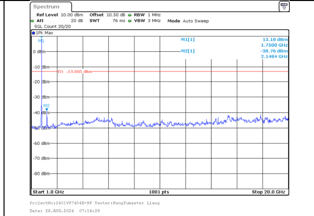
1000.0MHz-20000.0MHz Band 66 15MHz/1745.3/Mid 256QAM 1@74 Band 66 20MHz/1762.4/Mid 256QAM 1@0
