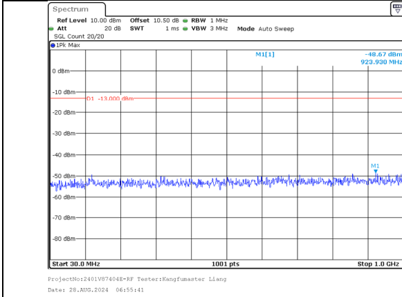
30.0MHz-1000.0MHz Band 66 20MHz/1750.1/Mid 256QAM 100@0 Band 66 10MHz/1764.5/Mid 256QAM 100@0
