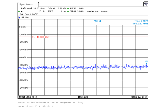
30.0MHz-1000.0MHz Band 66 20MHz/1747.6/Mid 16QAM 100@0 Band 66 15MHz/1764.7/Mid 16QAM 100@0
