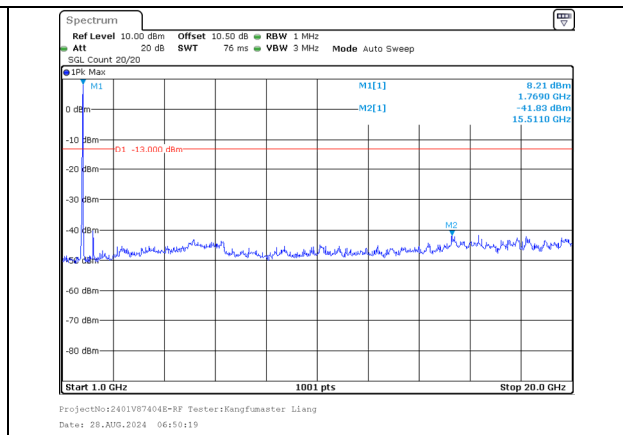
1000.0MHz-20000.0MHz Band 66 20MHz/1750.1/Mid 16QAM 100@0 Band 66 10MHz/1764.5/Mid 16QAM 100@0
