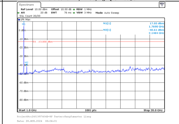
1000.0MHz-20000.0MHz Band 66 10MHz/1755.6/High 16QAM 1@49 Band 66 20MHz/1770.0/High 16QAM 1@0
