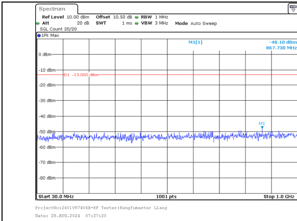
30.0MHz-1000.0MHz Band 66 20MHz/1747.6/Mid 256QAM 1@99 Band 66 15MHz/1764.7/Mid 256QAM 1@0
