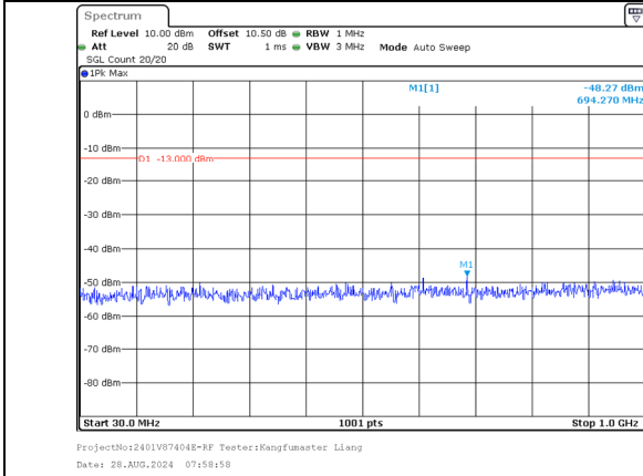
30.0MHz-1000.0MHz Band 66 20MHz/1745.1/Mid 64QAM 100@0 Band 66 20MHz/1764.9/Mid 64QAM 100@0
