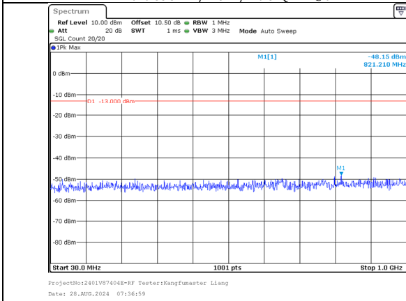
30.0MHz-1000.0MHz Band 66 20MHz/1752.5/Mid 64QAM 100@0 Band 66 5MHz/1764.2/Mid 64QAM 25@0
