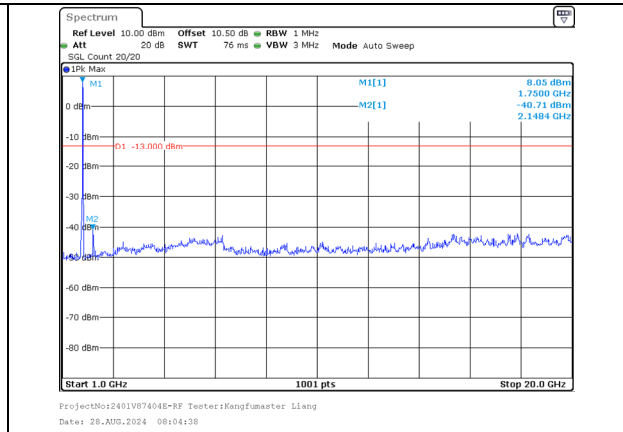
1000.0MHz-20000.0MHz Band 66 10MHz/1755.6/High QPSK 50@0 Band 66 20MHz/1770.0/High QPSK 100@0
