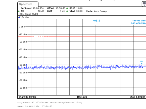
30.0MHz-1000.0MHz Band 66 20MHz/1747.6/Mid QPSK 100@0 Band 66 15MHz/1764.7/Mid QPSK 100@0
