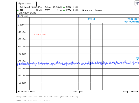
30.0MHz-1000.0MHz Band 66 20MHz/1752.5/Mid QPSK 1@99 Band 66 5MHz/1764.2/Mid QPSK 1@0
