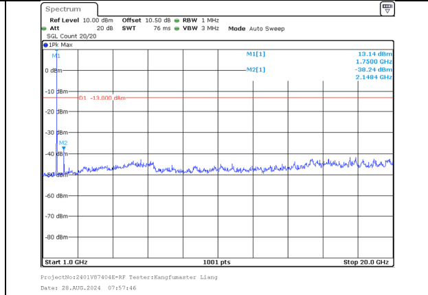
1000.0MHz-20000.0MHz Band 66 20MHz/1745.1/Mid 64QAM 1@99 Band 66 20MHz/1764.9/Mid 64QAM 1@0
