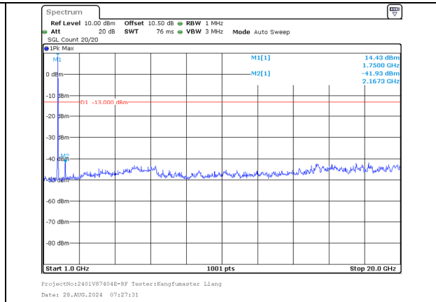
1000.0MHz-20000.0MHz Band 66 20MHz/1747.6/Mid 256QAM 1@99 Band 66 15MHz/1764.7/Mid 256QAM 1@0
