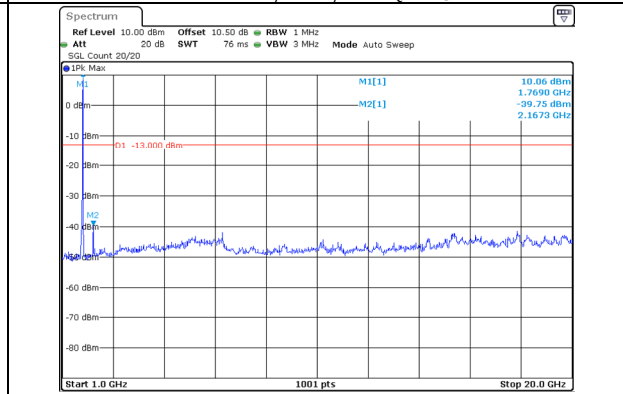
1000.0MHz-20000.0MHz Band 66 20MHz/1752.5/Mid 16QAM 1@99 Band 66 5MHz/1764.2/Mid 16QAM 1@0
