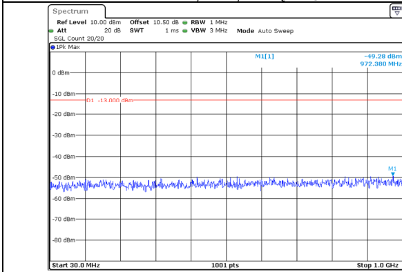
30.0MHz-1000.0MHz Band 66 20MHz/1752.5/Mid 16QAM 1@99 Band 66 5MHz/1764.2/Mid 16QAM 1@0
