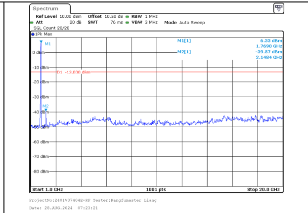
1000.0MHz-20000.0MHz Band 66 20MHz/1747.6/Mid 16QAM 100@0 Band 66 15MHz/1764.7/Mid 16QAM 100@0
