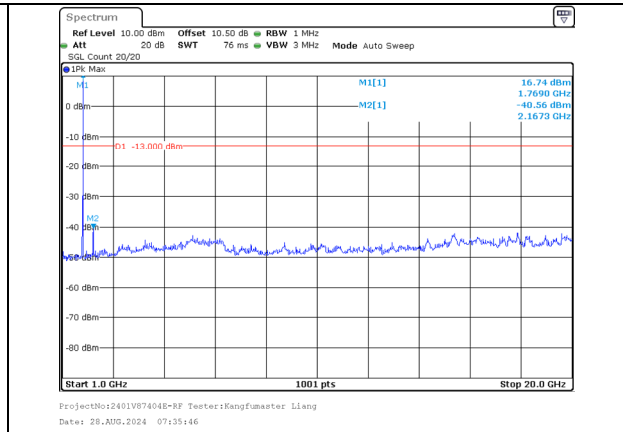
1000.0MHz-20000.0MHz Band 66 20MHz/1752.5/Mid 64QAM 1@99 Band 66 5MHz/1764.2/Mid 64QAM 1@0
