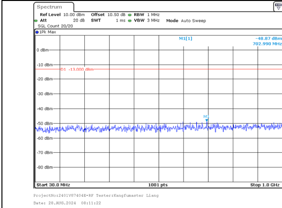
30.0MHz-1000.0MHz Band 66 10MHz/1755.6/High 256QAM 1@49 Band 66 20MHz/1770.0/High 256QAM 1@0
