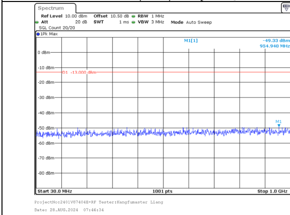
30.0MHz-1000.0MHz Band 66 5MHz/1745.8/Mid 64QAM 1@24 Band 66 20MHz/1757.5/Mid 64QAM 1@0
