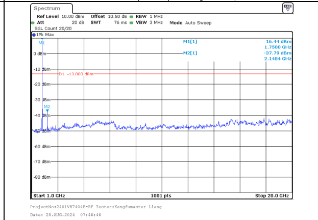
1000.0MHz-20000.0MHz Band 66 5MHz/1745.8/Mid 64QAM 1@24 Band 66 20MHz/1757.5/Mid 64QAM 1@0
