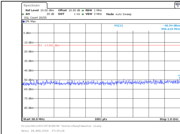
30.0MHz-1000.0MHz Band 66 20MHz/1752.5/Mid 64QAM 1@99 Band 66 5MHz/1764.2/Mid 64QAM 1@0
