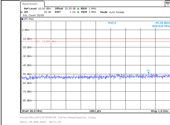
30.0MHz-1000.0MHz Band 66 20MHz/1750.1/Mid 64QAM 1@99 Band 66 10MHz/1764.5/Mid 64QAM 1@0
