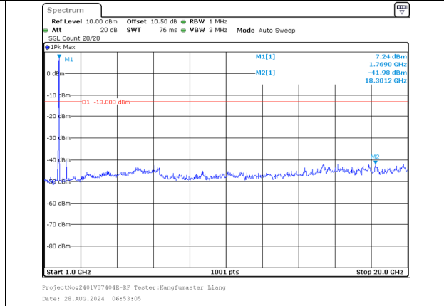
1000.0MHz-20000.0MHz Band 66 20MHz/1750.1/Mid 64QAM 100@0 Band 66 10MHz/1764.5/Mid 64QAM 100@0
