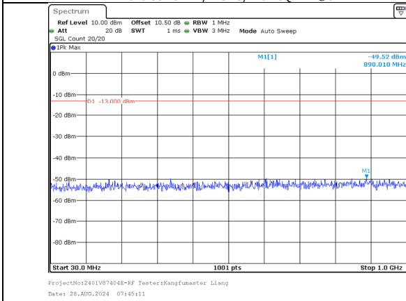
30.0MHz-1000.0MHz Band 66 5MHz/1745.8/Mid 16QAM 25@0 Band 66 20MHz/1757.5/Mid 16QAM 100@0
