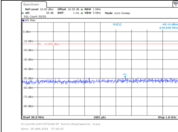
30.0MHz-1000.0MHz Band 66 5MHz/1745.8/Mid QPSK 25@0 Band 66 20MHz/1757.5/Mid QPSK 100@0
