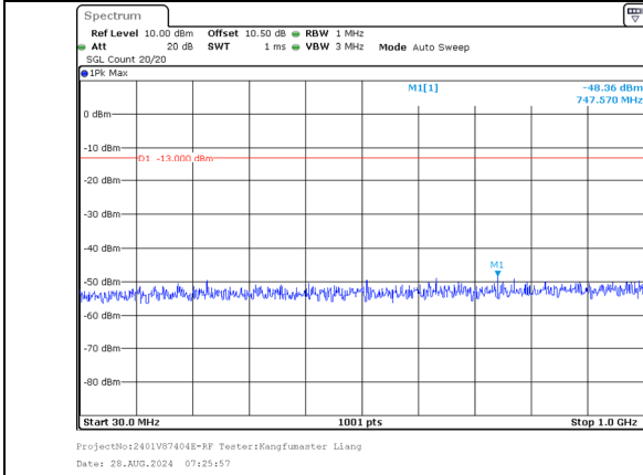
30.0MHz-1000.0MHz Band 66 20MHz/1747.6/Mid 64QAM 100@0 Band 66 15MHz/1764.7/Mid 64QAM 100@0
