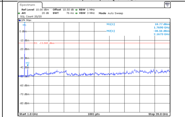
1000.0MHz-20000.0MHz Band 66 20MHz/1752.5/Mid QPSK 100@0 Band 66 5MHz/1764.2/Mid QPSK 25@0
