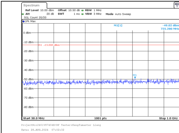
30.0MHz-1000.0MHz Band 66 15MHz/1747.5/Mid 64QAM 1@74 Band 66 15MHz/1762.5/Mid 64QAM 1@0
