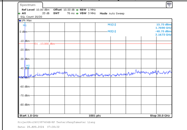
1000.0MHz-20000.0MHz Band 66 20MHz/1752.5/Mid 256QAM 1@99 Band 66 5MHz/1764.2/Mid 256QAM 1@0
