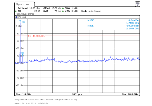
1000.0MHz-20000.0MHz Band 66 20MHz/1745.1/Mid 16QAM 100@0 Band 66 20MHz/1764.9/Mid 16QAM 100@0
