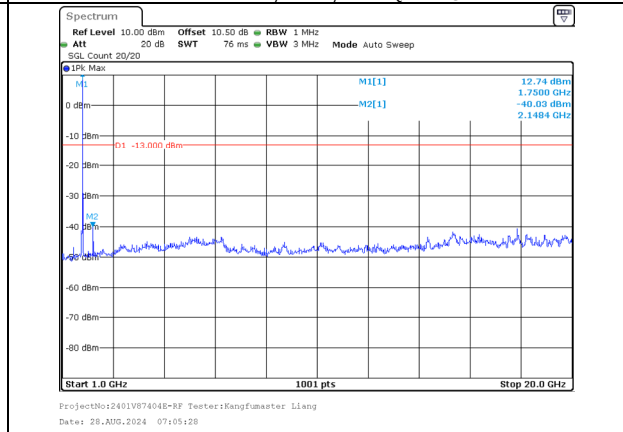
1000.0MHz-20000.0MHz Band 66 15MHz/1747.5/Mid 256QAM 1@74 Band 66 15MHz/1762.5/Mid 256QAM 1@0
