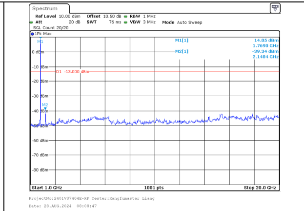
1000.0MHz-20000.0MHz Band 66 10MHz/1755.6/High 64QAM 1@49 Band 66 20MHz/1770.0/High 64QAM 1@0
