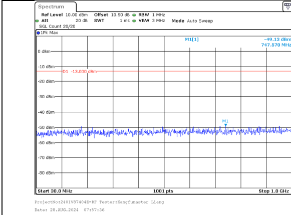
30.0MHz-1000.0MHz Band 66 20MHz/1745.1/Mid 64QAM 1@99 Band 66 20MHz/1764.9/Mid 64QAM 1@0
