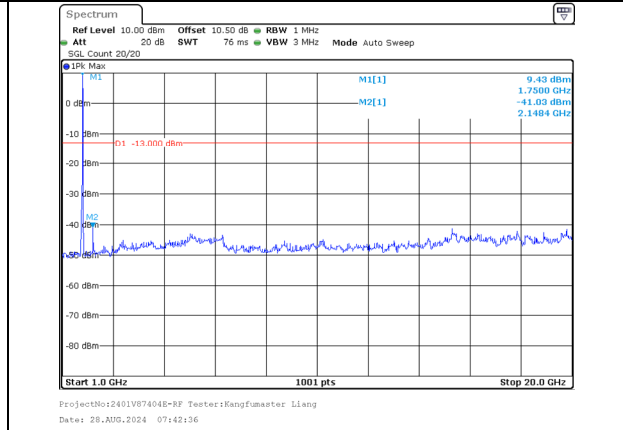
1000.0MHz-20000.0MHz Band 66 5MHz/1745.8/Mid QPSK 25@0 Band 66 20MHz/1757.5/Mid QPSK 100@0
