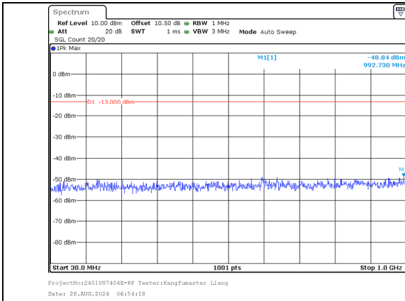
30.0MHz-1000.0MHz Band 66 20MHz/1750.1/Mid 256QAM 1@99 Band 66 10MHz/1764.5/Mid 256QAM 1@0
