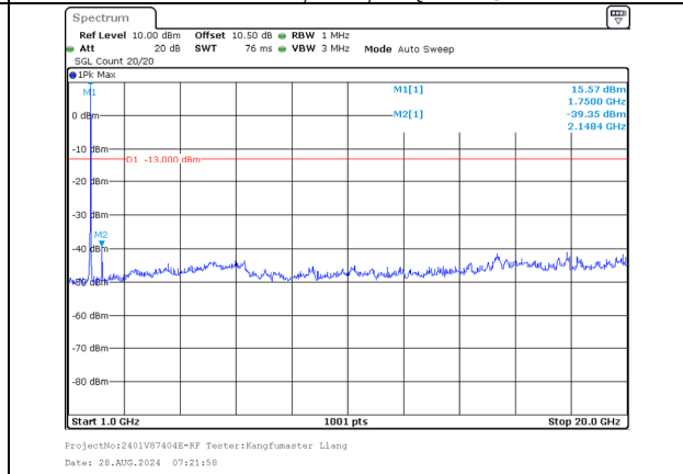
1000.0MHz-20000.0MHz Band 66 20MHz/1747.6/Mid 16QAM 1@99 Band 66 15MHz/1764.7/Mid 16QAM 1@0
