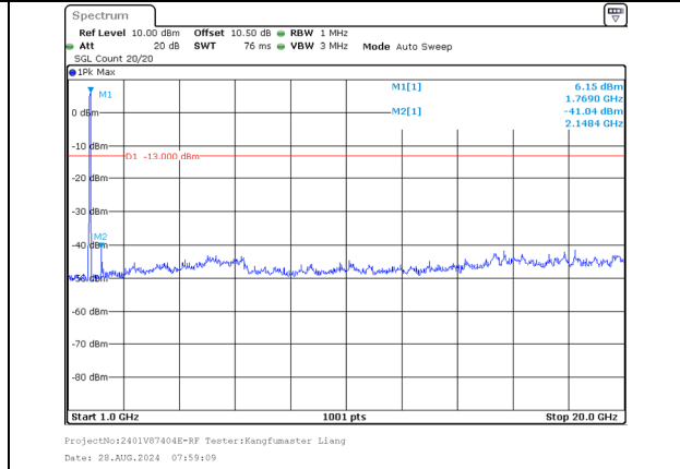
1000.0MHz-20000.0MHz Band 66 20MHz/1745.1/Mid 64QAM 100@0 Band 66 20MHz/1764.9/Mid 64QAM 100@0
