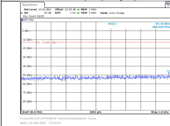
30.0MHz-1000.0MHz Band 66 15MHz/1747.5/Mid 64QAM 75@0 Band 66 15MHz/1762.5/Mid 64QAM 75@0
