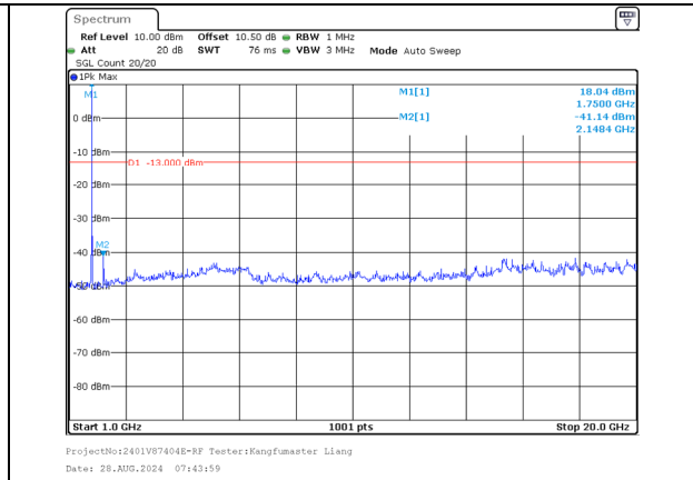
1000.0MHz-20000.0MHz Band 66 5MHz/1745.8/Mid 16QAM 1@24 Band 66 20MHz/1757.5/Mid 16QAM 1@0
