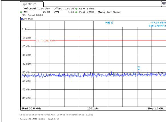
30.0MHz-1000.0MHz Band 66 20MHz/1750.1/Mid 64QAM 100@0 Band 66 10MHz/1764.5/Mid 64QAM 100@0
