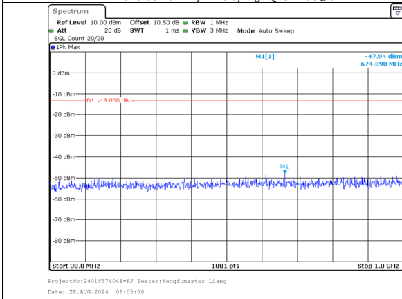
30.0MHz-1000.0MHz Band 66 10MHz/1755.6/High 16QAM 1@49 Band 66 20MHz/1770.0/High 16QAM 1@0
