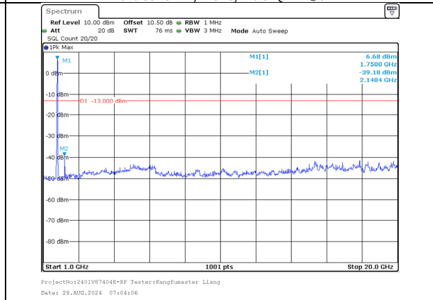
1000.0MHz-20000.0MHz Band 66 15MHz/1747.5/Mid 64QAM 75@0 Band 66 15MHz/1762.5/Mid 64QAM 75@0
