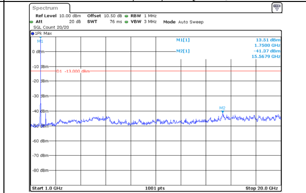
1000.0MHz-20000.0MHz Band 66 15MHz/1745.3/Mid 16QAM 75@0 Band 66 20MHz/1762.4/Mid 16QAM 100@0
