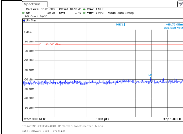
30.0MHz-1000.0MHz Band 66 20MHz/1747.6/Mid 64QAM 1@99 Band 66 15MHz/1764.7/Mid 64QAM 1@0
