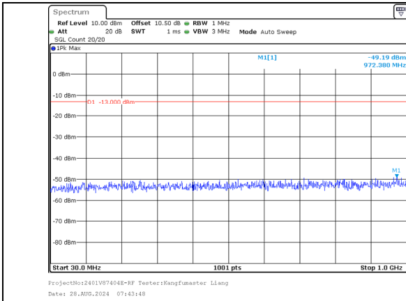
30.0MHz-1000.0MHz Band 66 5MHz/1745.8/Mid 16QAM 1@24 Band 66 20MHz/1757.5/Mid 16QAM 1@0
