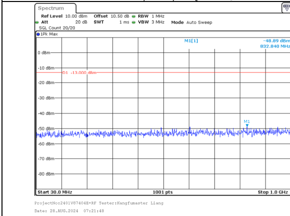
30.0MHz-1000.0MHz Band 66 20MHz/1747.6/Mid 16QAM 1@99 Band 66 15MHz/1764.7/Mid 16QAM 1@0
