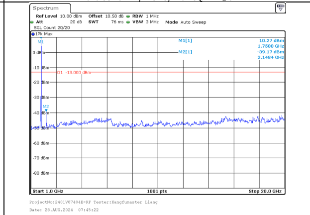
1000.0MHz-20000.0MHz Band 66 5MHz/1745.8/Mid 16QAM 25@0 Band 66 20MHz/1757.5/Mid 16QAM 100@0
