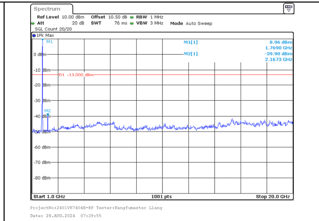
1000.0MHz-20000.0MHz Band 66 20MHz/1752.5/Mid 256QAM 100@0 Band 66 5MHz/1764.2/Mid 256QAM 25@0
