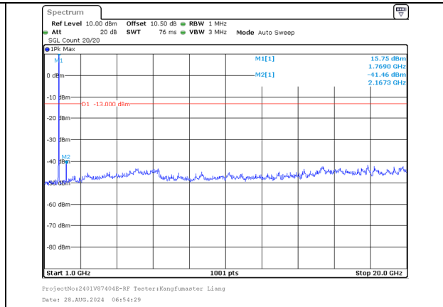
1000.0MHz-20000.0MHz Band 66 20MHz/1750.1/Mid 256QAM 1@99 Band 66 10MHz/1764.5/Mid 256QAM 1@0
