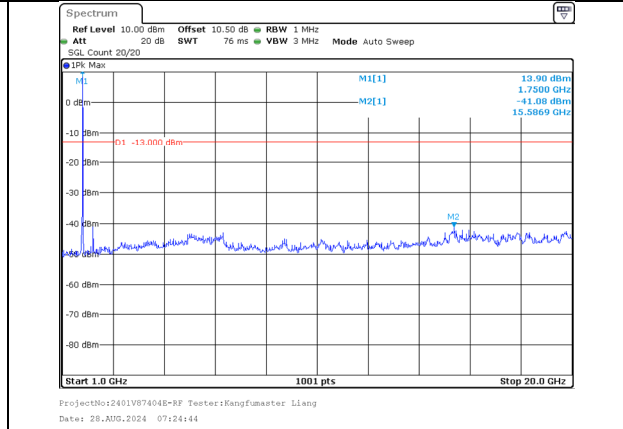
1000.0MHz-20000.0MHz Band 66 20MHz/1747.6/Mid 64QAM 1@99 Band 66 15MHz/1764.7/Mid 64QAM 1@0
