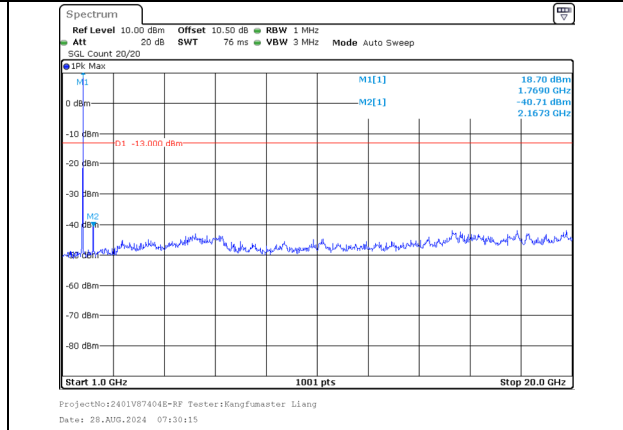
1000.0MHz-20000.0MHz Band 66 20MHz/1752.5/Mid QPSK 1@99 Band 66 5MHz/1764.2/Mid QPSK 1@0
