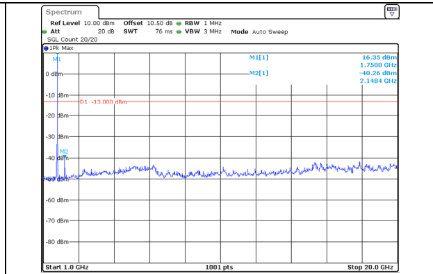
1000.0MHz-20000.0MHz Band 66 15MHz/1745.3/Mid 16QAM 1@74 Band 66 20MHz/1762.4/Mid 16QAM 1@0
