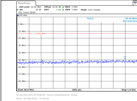
30.0MHz-1000.0MHz Band 66 20MHz/1747.6/Mid 256QAM 100@0 Band 66 15MHz/1764.7/Mid 256QAM 100@0
