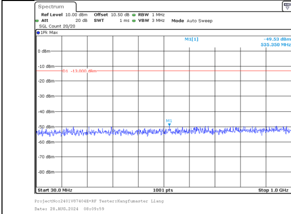
30.0MHz-1000.0MHz Band 66 10MHz/1755.6/High 64QAM 50@0 Band 66 20MHz/1770.0/High 64QAM 100@0
