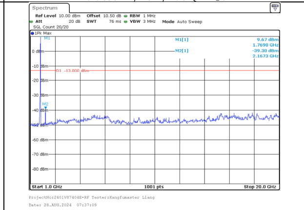
1000.0MHz-20000.0MHz Band 66 20MHz/1752.5/Mid 64QAM 100@0 Band 66 5MHz/1764.2/Mid 64QAM 25@0
