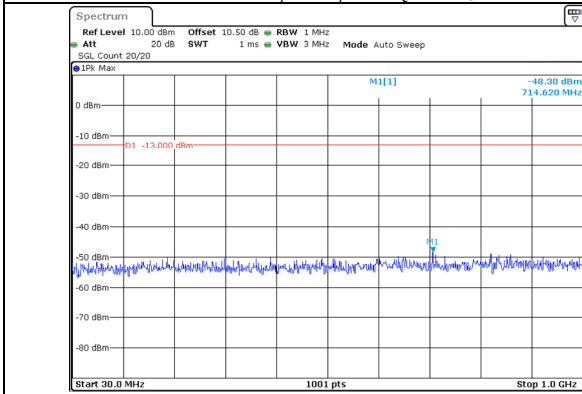
30.0MHz-1000.0MHz Band 66 15MHz/1745.3/Mid 16QAM 75@0 Band 66 20MHz/1762.4/Mid 16QAM 100@0
