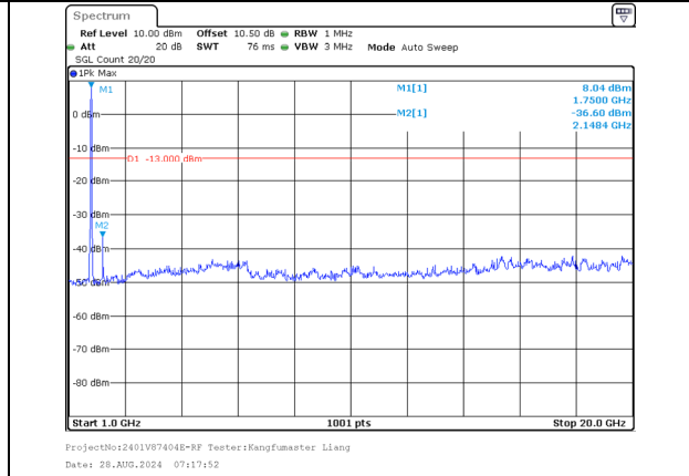
1000.0MHz-20000.0MHz Band 66 15MHz/1745.3/Mid 256QAM 75@0 Band 66 20MHz/1762.4/Mid 256QAM 100@0
