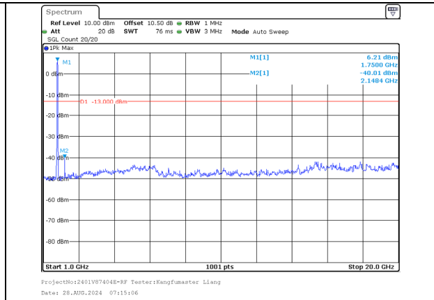
1000.0MHz-20000.0MHz Band 66 15MHz/1745.3/Mid 64QAM 75@0 Band 66 20MHz/1762.4/Mid 64QAM 100@0
