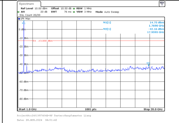
1000.0MHz-20000.0MHz Band 66 20MHz/1750.1/Mid 64QAM 1@99 Band 66 10MHz/1764.5/Mid 64QAM 1@0
