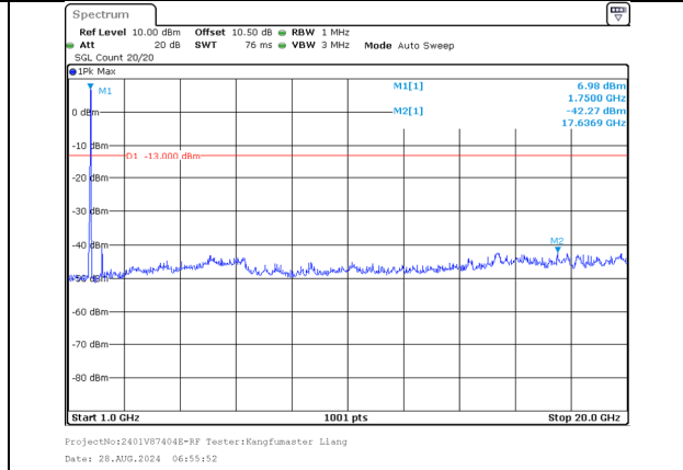
1000.0MHz-20000.0MHz Band 66 20MHz/1750.1/Mid 256QAM 100@0 Band 66 10MHz/1764.5/Mid 256QAM 100@0
