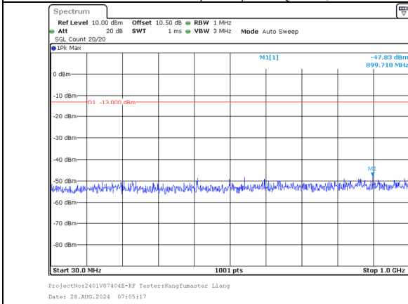
30.0MHz-1000.0MHz Band 66 15MHz/1747.5/Mid 256QAM 1@74 Band 66 15MHz/1762.5/Mid 256QAM 1@0
