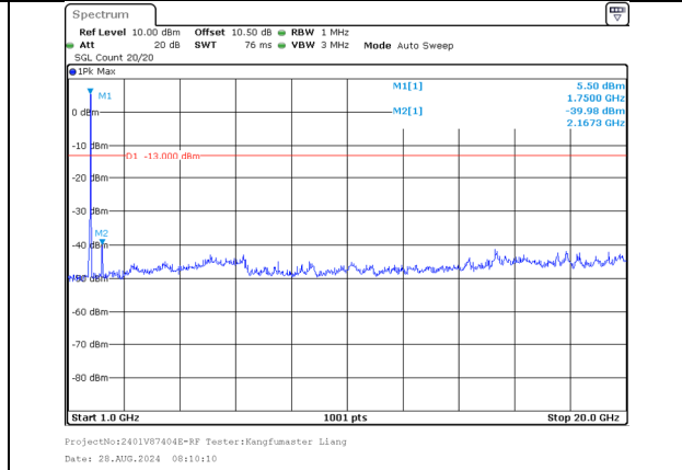
1000.0MHz-20000.0MHz Band 66 10MHz/1755.6/High 64QAM 50@0 Band 66 20MHz/1770.0/High 64QAM 100@0
