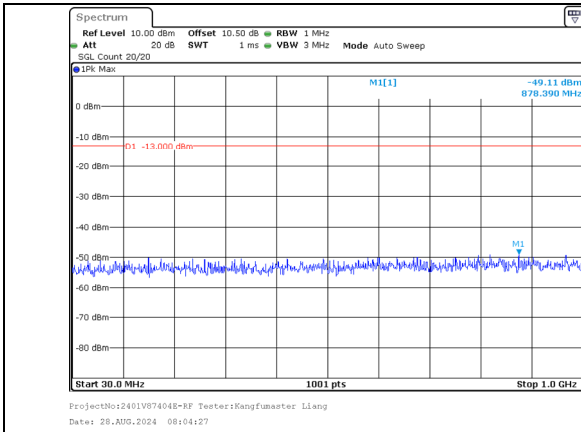
30.0MHz-1000.0MHz Band 66 10MHz/1755.6/High QPSK 50@0 Band 66 20MHz/1770.0/High QPSK 100@0
