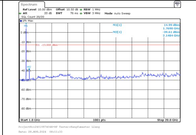
1000.0MHz-20000.0MHz Band 66 10MHz/1755.6/High 256QAM 1@49 Band 66 20MHz/1770.0/High 256QAM 1@0
