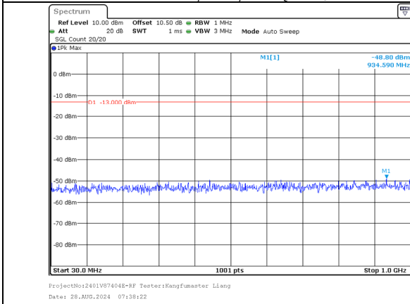
30.0MHz-1000.0MHz Band 66 20MHz/1752.5/Mid 256QAM 1@99 Band 66 5MHz/1764.2/Mid 256QAM 1@0
