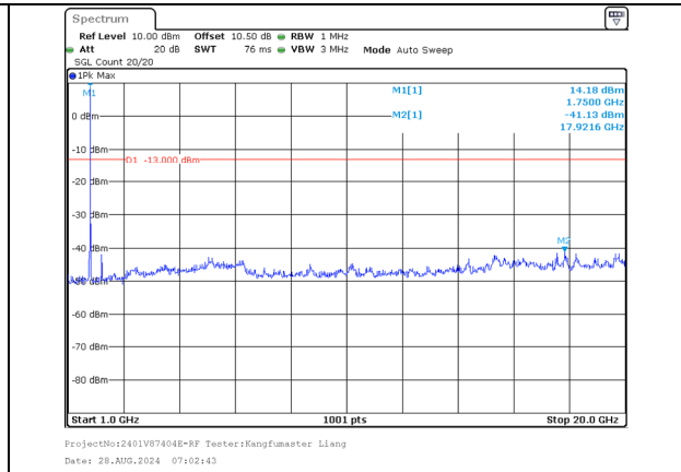
1000.0MHz-20000.0MHz Band 66 15MHz/1747.5/Mid 64QAM 1@74 Band 66 15MHz/1762.5/Mid 64QAM 1@0
