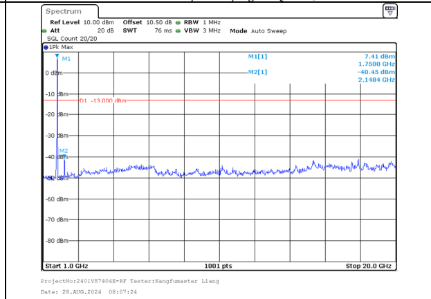
1000.0MHz-20000.0MHz Band 66 10MHz/1755.6/High 16QAM 50@0 Band 66 20MHz/1770.0/High 16QAM 100@0
