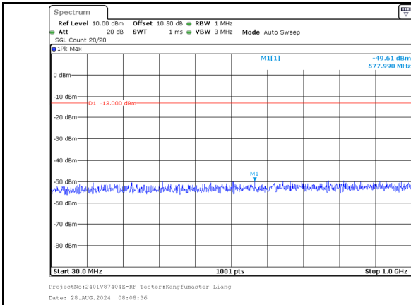
30.0MHz-1000.0MHz Band 66 10MHz/1755.6/High 64QAM 1@49 Band 66 20MHz/1770.0/High 64QAM 1@0
