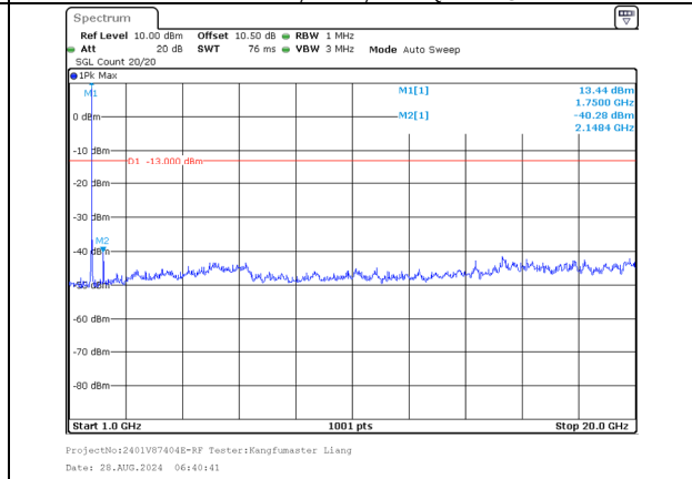
1000.0MHz-20000.0MHz Band 66 10MHz/1745.6/Mid 64QAM 1@49 Band 66 20MHz/1760.0/Mid 64QAM 1@0
