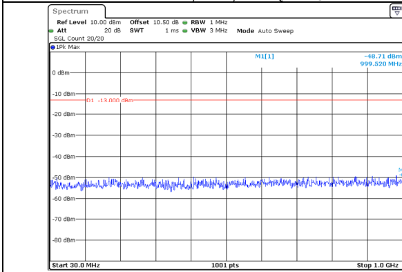
30.0MHz-1000.0MHz Band 66 20MHz/1720.0/Low 16QAM 100@0 Band 66 5MHz/1731.7/Low 16QAM 25@0
