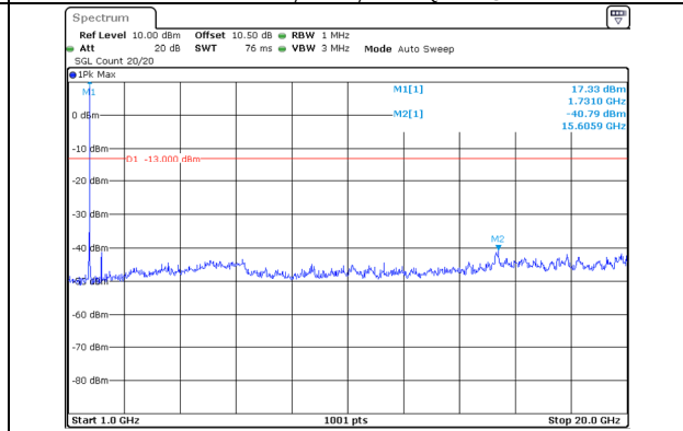
1000.0MHz-20000.0MHz Band 66 20MHz/1720.0/Low 16QAM 100@0 Band 66 5MHz/1731.7/Low 16QAM 25@0
