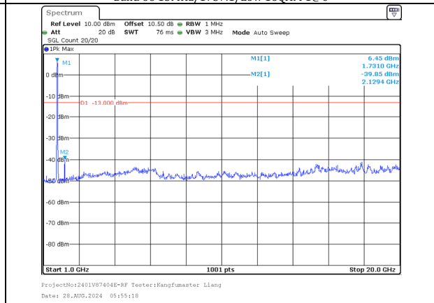
1000.0MHz-20000.0MHz Band 66 20MHz/1720.0/Low 16QAM 100@0 Band 66 15MHz/1737.1/Low 16QAM 100@0
