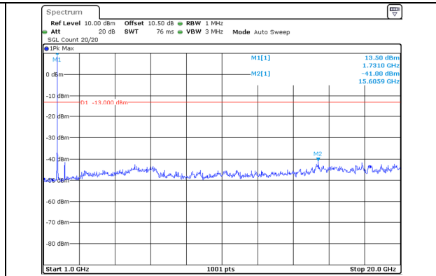
1000.0MHz-20000.0MHz Band 66 20MHz/1720.0/Low 64QAM 1@99 Band 66 20MHz/1739.8/Low 64QAM 1@0
