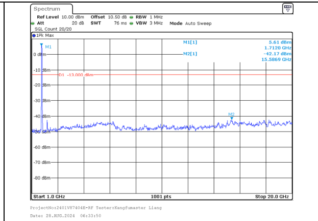
1000.0MHz-20000.0MHz Band 66 20MHz/1720.0/Low 256QAM 100@0 Band 66 20MHz/1739.8/Low 256QAM 100@0
