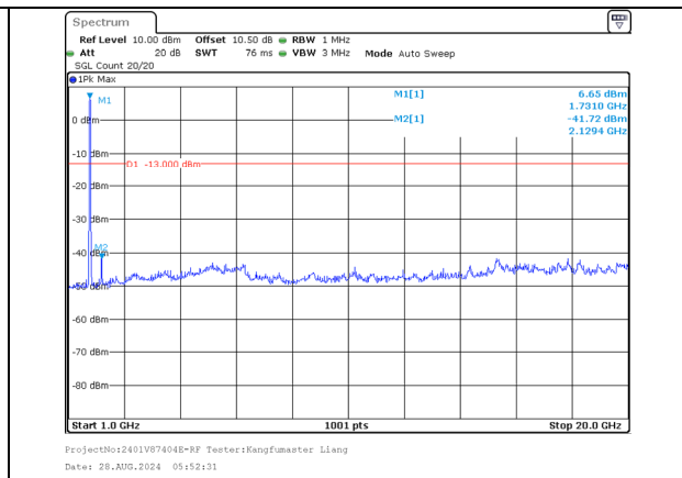
1000.0MHz-20000.0MHz Band 66 20MHz/1720.0/Low QPSK 100@0 Band 66 15MHz/1737.1/Low QPSK 100@0
