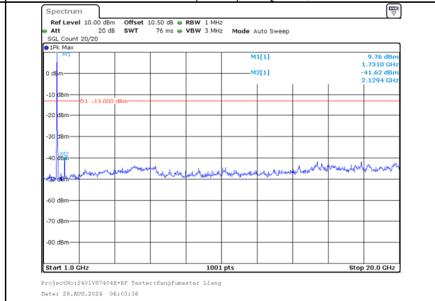
1000.0MHz-20000.0MHz Band 66 20MHz/1720.0/Low QPSK 100@0 Band 66 5MHz/1731.7/Low QPSK 25@0
