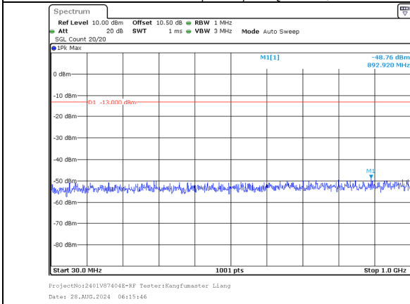
30.0MHz-1000.0MHz Band 66 5MHz/1713.3/Low 16QAM 1@24 Band 66 20MHz/1725.0/Low 16QAM 1@0
