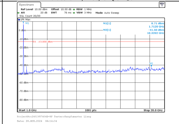
1000.0MHz-20000.0MHz Band 66 5MHz/1713.3/Low QPSK 25@0 Band 66 20MHz/1725.0/Low QPSK 100@0
