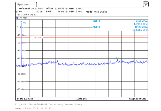
1000.0MHz-20000.0MHz Band 66 20MHz/1720.0/Low 256QAM 100@0 Band 66 15MHz/1737.1/Low 256QAM 100@0
