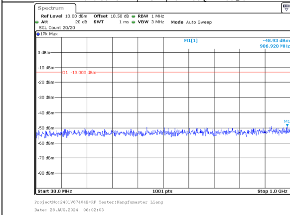
30.0MHz-1000.0MHz Band 66 20MHz/1720.0/Low QPSK 1@99 Band 66 5MHz/1731.7/Low QPSK 1@0
