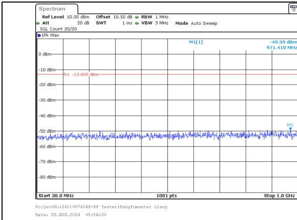
30.0MHz-1000.0MHz Band 66 20MHz/1720.0/Low 64QAM 1@99 Band 66 15MHz/1737.1/Low 64QAM 1@0
