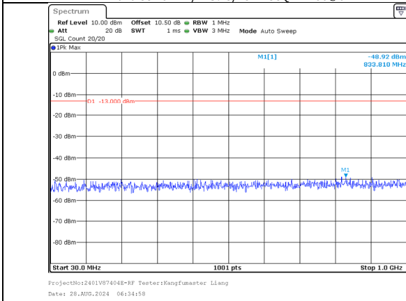
30.0MHz-1000.0MHz Band 66 10MHz/1745.6/Mid QPSK 1@49 Band 66 20MHz/1760.0/Mid QPSK 1@0
