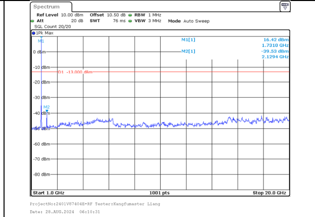
1000.0MHz-20000.0MHz Band 66 20MHz/1720.0/Low 256QAM 1@99 Band 66 5MHz/1731.7/Low 256QAM 1@0
