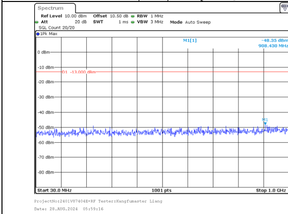
30.0MHz-1000.0MHz Band 66 20MHz/1720.0/Low 256QAM 1@99 Band 66 15MHz/1737.1/Low 256QAM 1@0
