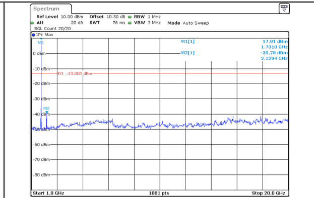
1000.0MHz-20000.0MHz Band 66 20MHz/1720.0/Low 16QAM 1@99 Band 66 5MHz/1731.7/Low 16QAM 1@0
