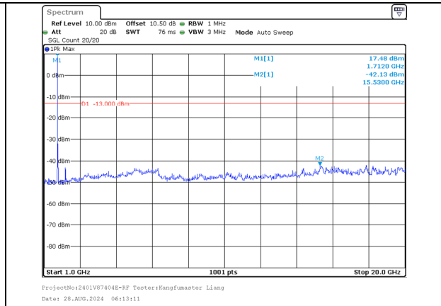
1000.0MHz-20000.0MHz Band 66 5MHz/1713.3/Low QPSK 1@24 Band 66 20MHz/1725.0/Low QPSK 1@0
