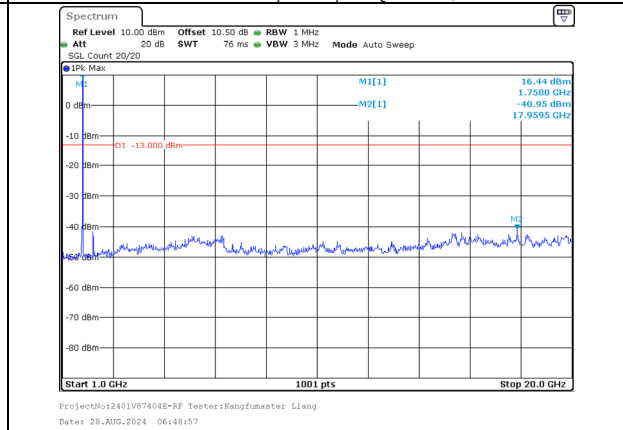
1000.0MHz-20000.0MHz Band 66 20MHz/1750.1/Mid 16QAM 1@99 Band 66 10MHz/1764.5/Mid 16QAM 1@0
