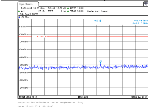
30.0MHz-1000.0MHz Band 66 20MHz/1720.0/Low QPSK 1@99 Band 66 20MHz/1739.8/Low QPSK 1@0
