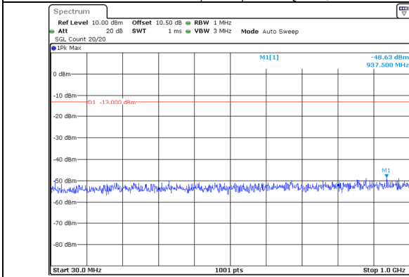
30.0MHz-1000.0MHz Band 66 10MHz/1745.6/Mid 256QAM 1@49 Band 66 20MHz/1760.0/Mid 256QAM 1@0
