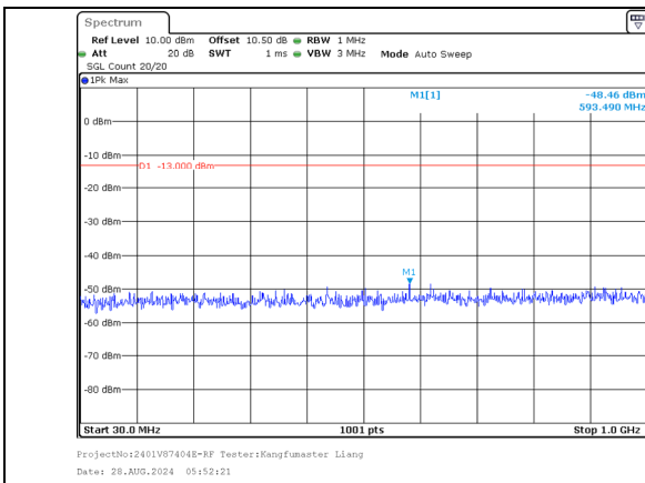
30.0MHz-1000.0MHz Band 66 20MHz/1720.0/Low QPSK 100@0 Band 66 15MHz/1737.1/Low QPSK 100@0
