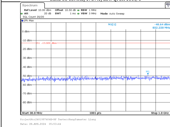
30.0MHz-1000.0MHz Band 66 20MHz/1720.0/Low 16QAM 1@99 Band 66 15MHz/1737.1/Low 16QAM 1@0
