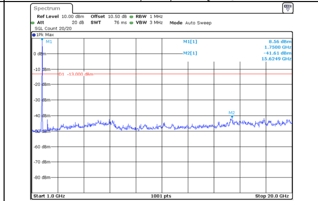
1000.0MHz-20000.0MHz Band 66 10MHz/1745.6/Mid 256QAM 1@49 Band 66 20MHz/1760.0/Mid 256QAM 1@0
