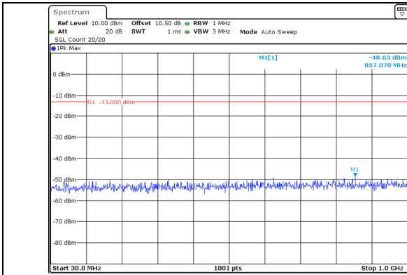
30.0MHz-1000.0MHz Band 66 20MHz/1720.0/Low 64QAM 1@99 Band 66 20MHz/1739.8/Low 64QAM 1@0
