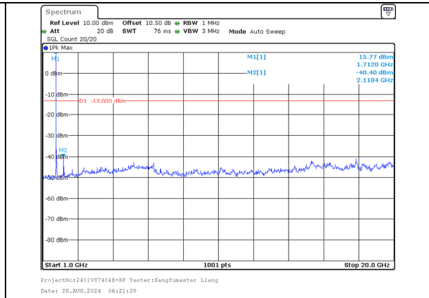
1000.0MHz-20000.0MHz Band 66 5MHz/1713.3/Low 256QAM 1@24 Band 66 20MHz/1725.0/Low 256QAM 1@0
