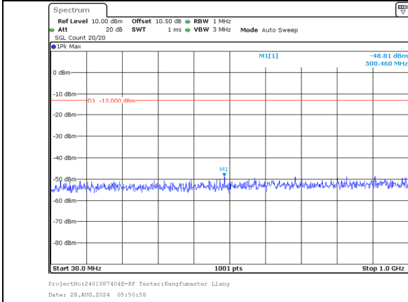
30.0MHz-1000.0MHz Band 66 20MHz/1720.0/Low QPSK 1@99 Band 66 15MHz/1737.1/Low QPSK 1@0
