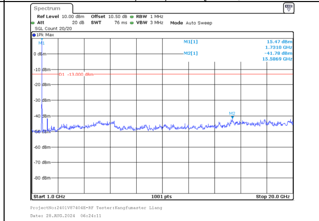
1000.0MHz-20000.0MHz Band 66 20MHz/1720.0/Low QPSK 1@99 Band 66 20MHz/1739.8/Low QPSK 1@0
