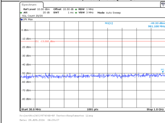
30.0MHz-1000.0MHz Band 66 10MHz/1745.6/Mid 16QAM 50@0 Band 66 20MHz/1760.0/Mid 16QAM 100@0
