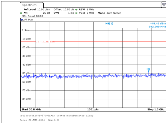
30.0MHz-1000.0MHz Band 66 20MHz/1750.1/Mid QPSK 1@99 Band 66 10MHz/1764.5/Mid QPSK 1@0
