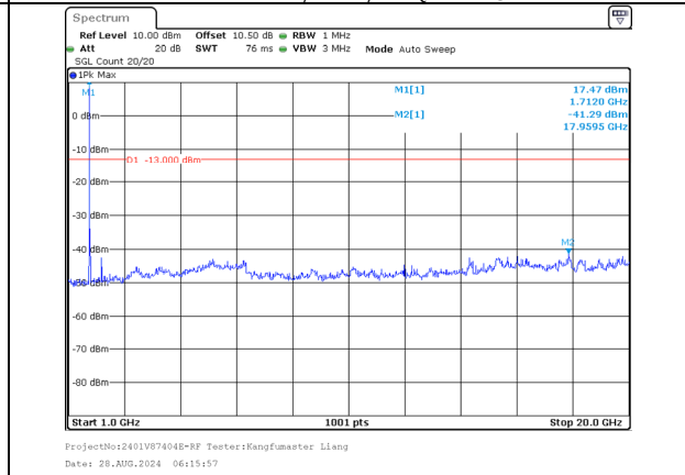
1000.0MHz-20000.0MHz Band 66 5MHz/1713.3/Low 16QAM 1@24 Band 66 20MHz/1725.0/Low 16QAM 1@0
