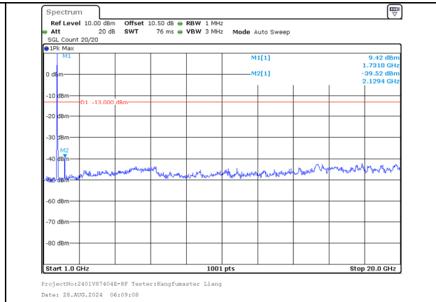
1000.0MHz-20000.0MHz Band 66 20MHz/1720.0/Low 64QAM 100@0 Band 66 5MHz/1731.7/Low 64QAM 25@0
