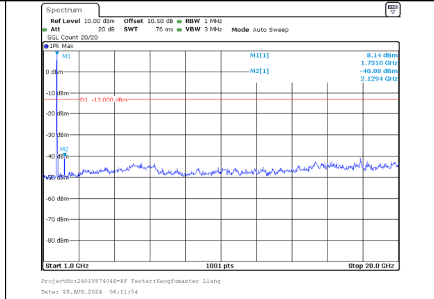
1000.0MHz-20000.0MHz Band 66 20MHz/1720.0/Low 256QAM 100@0 Band 66 5MHz/1731.7/Low 256QAM 25@0
