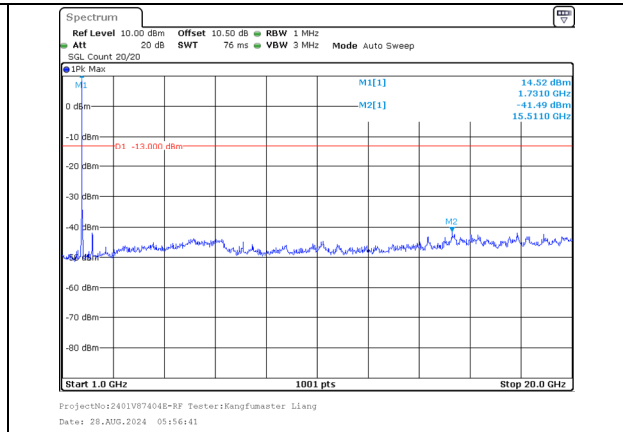
1000.0MHz-20000.0MHz Band 66 20MHz/1720.0/Low 64QAM 1@99 Band 66 15MHz/1737.1/Low 64QAM 1@0
