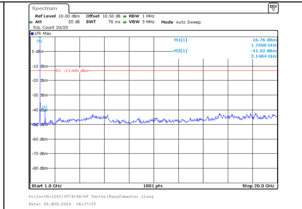
1000.0MHz-20000.0MHz Band 66 10MHz/1745.6/Mid 16QAM 1@49 Band 66 20MHz/1760.0/Mid 16QAM 1@0
