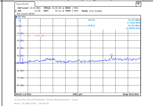
1000.0MHz-20000.0MHz Band 66 20MHz/1720.0/Low 16QAM 1@99 Band 66 20MHz/1739.8/Low 16QAM 1@0
