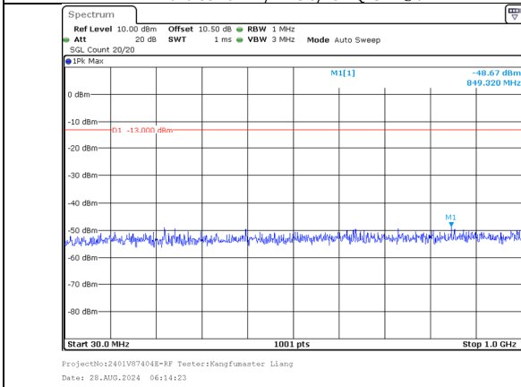
30.0MHz-1000.0MHz Band 66 5MHz/1713.3/Low QPSK 25@0 Band 66 20MHz/1725.0/Low QPSK 100@0
