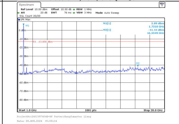
1000.0MHz-20000.0MHz Band 66 20MHz/1720.0/Low 64QAM 100@0 Band 66 15MHz/1737.1/Low 64QAM 100@0
