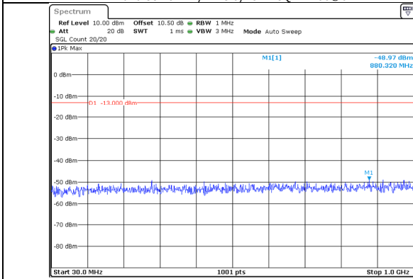
30.0MHz-1000.0MHz Band 66 5MHz/1713.3/Low 16QAM 25@0 Band 66 20MHz/1725.0/Low 16QAM 100@0
