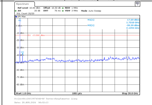
1000.0MHz-20000.0MHz Band 66 20MHz/1720.0/Low QPSK 1@99 Band 66 5MHz/1731.7/Low QPSK 1@0
