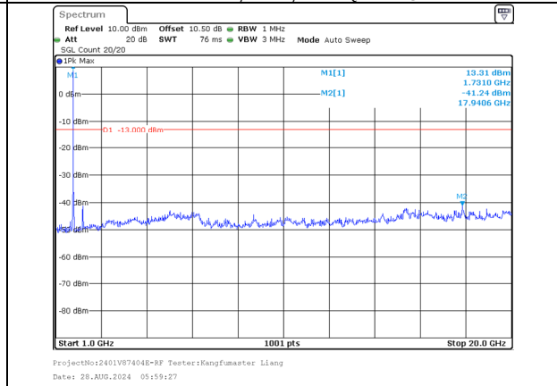
1000.0MHz-20000.0MHz Band 66 20MHz/1720.0/Low 256QAM 1@99 Band 66 15MHz/1737.1/Low 256QAM 1@0
