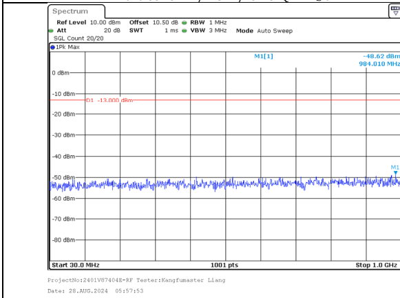
30.0MHz-1000.0MHz Band 66 20MHz/1720.0/Low 64QAM 100@0 Band 66 15MHz/1737.1/Low 64QAM 100@0
