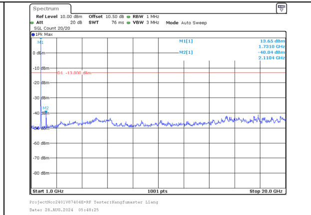
1000.0MHz-20000.0MHz Band 66 15MHz/1717.8/Low 256QAM 1@74 Band 66 20MHz/1734.9/Low 256QAM 1@0
