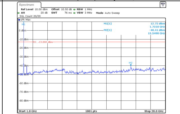
1000.0MHz-20000.0MHz Band 66 20MHz/1720.0/Low 64QAM 100@0 Band 66 20MHz/1739.8/Low 64QAM 100@0
