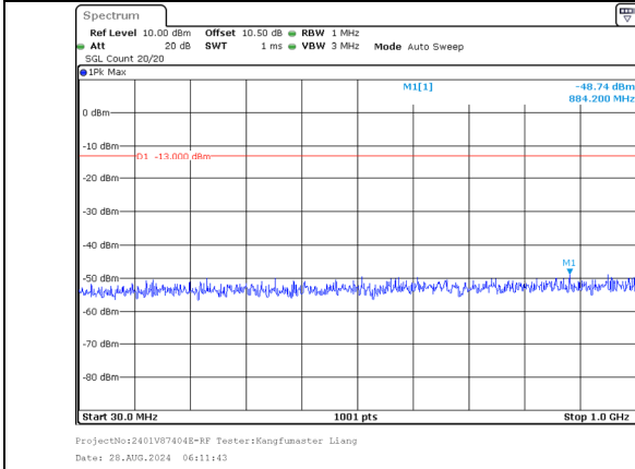
30.0MHz-1000.0MHz Band 66 20MHz/1720.0/Low 256QAM 100@0 Band 66 5MHz/1731.7/Low 256QAM 25@0
