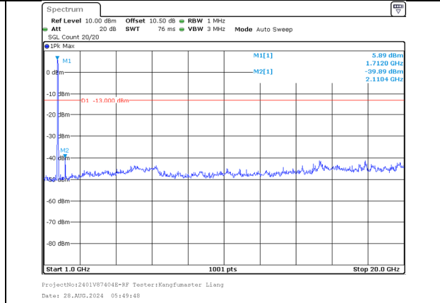
1000.0MHz-20000.0MHz Band 66 15MHz/1717.8/Low 256QAM 75@0 Band 66 20MHz/1734.9/Low 256QAM 100@0
