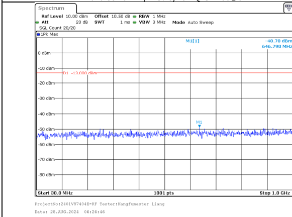
30.0MHz-1000.0MHz Band 66 20MHz/1720.0/Low 16QAM 1@99 Band 66 20MHz/1739.8/Low 16QAM 1@0
