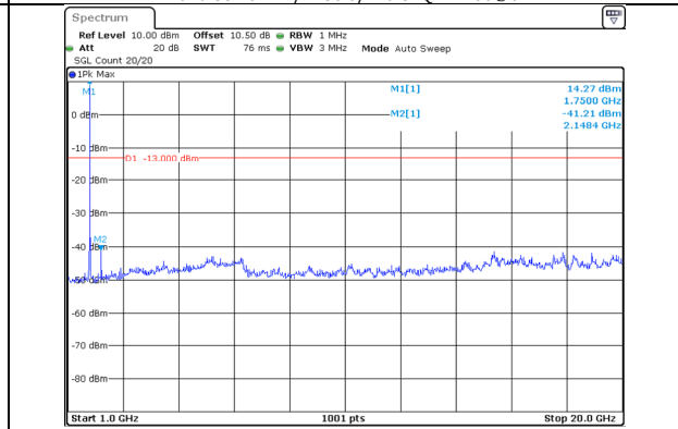
1000.0MHz-20000.0MHz Band 66 10MHz/1745.6/Mid 64QAM 50@0 Band 66 20MHz/1760.0/Mid 64QAM 100@0
