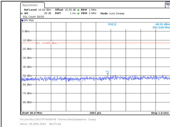
30.0MHz-1000.0MHz Band 66 10MHz/1745.6/Mid 16QAM 1@49 Band 66 20MHz/1760.0/Mid 16QAM 1@0
