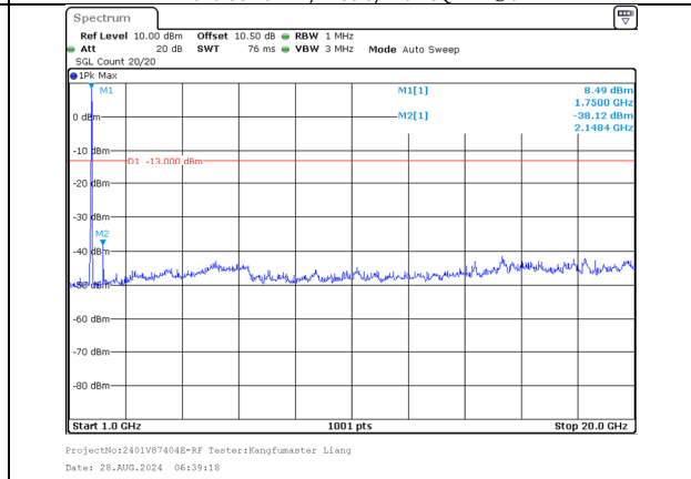
1000.0MHz-20000.0MHz Band 66 10MHz/1745.6/Mid 16QAM 50@0 Band 66 20MHz/1760.0/Mid 16QAM 100@0
