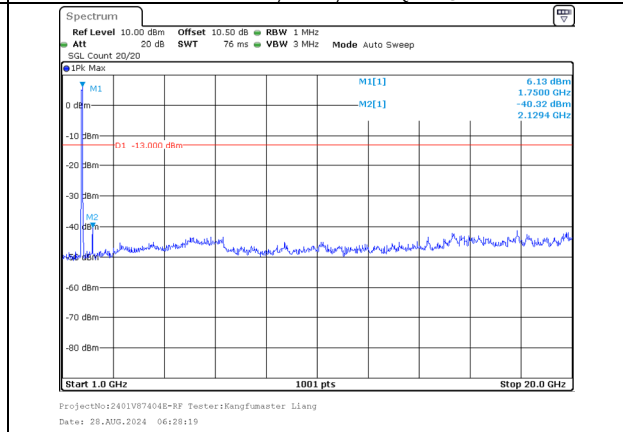
1000.0MHz-20000.0MHz Band 66 20MHz/1720.0/Low 16QAM 100@0 Band 66 20MHz/1739.8/Low 16QAM 100@0
