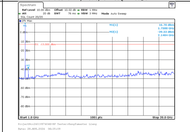
1000.0MHz-20000.0MHz Band 66 10MHz/1745.6/Mid QPSK 1@49 Band 66 20MHz/1760.0/Mid QPSK 1@0
