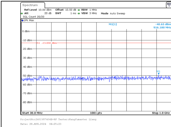
30.0MHz-1000.0MHz Band 66 20MHz/1720.0/Low QPSK 100@0 Band 66 20MHz/1739.8/Low QPSK 100@0
