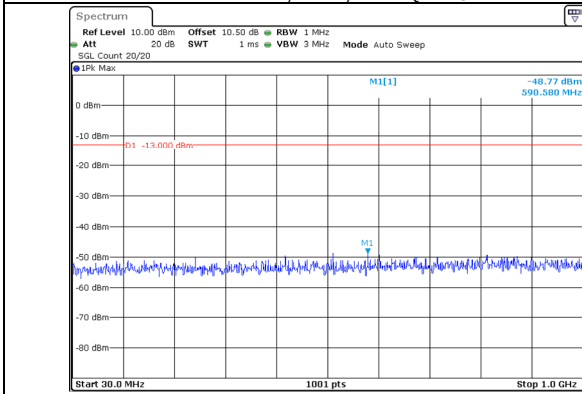
30.0MHz-1000.0MHz Band 66 5MHz/1713.3/Low 64QAM 1@24 Band 66 20MHz/1725.0/Low 64QAM 1@0
