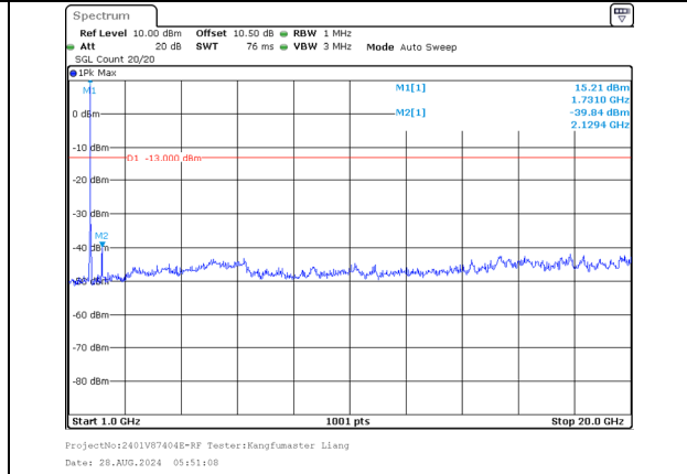
1000.0MHz-20000.0MHz Band 66 20MHz/1720.0/Low QPSK 1@99 Band 66 15MHz/1737.1/Low QPSK 1@0
