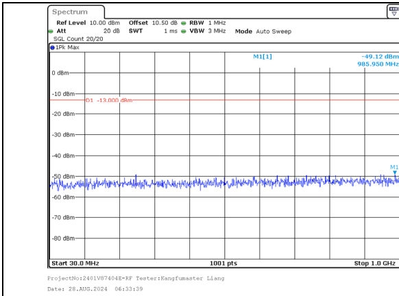
30.0MHz-1000.0MHz Band 66 20MHz/1720.0/Low 256QAM 100@0 Band 66 20MHz/1739.8/Low 256QAM 100@0
