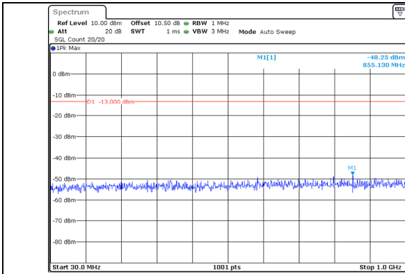
30.0MHz-1000.0MHz Band 66 20MHz/1720.0/Low 16QAM 1@99 Band 66 5MHz/1731.7/Low 16QAM 1@0
