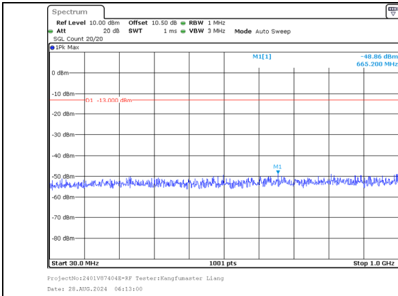
30.0MHz-1000.0MHz Band 66 5MHz/1713.3/Low QPSK 1@24 Band 66 20MHz/1725.0/Low QPSK 1@0
