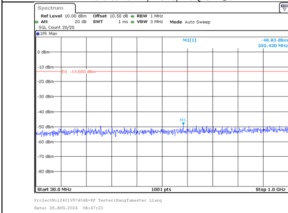
30.0MHz-1000.0MHz Band 66 20MHz/1750.1/Mid QPSK 100@0 Band 66 10MHz/1764.5/Mid QPSK 100@0
