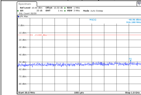
30.0MHz-1000.0MHz Band 66 20MHz/1720.0/Low 64QAM 100@0 Band 66 20MHz/1739.8/Low 64QAM 100@0
