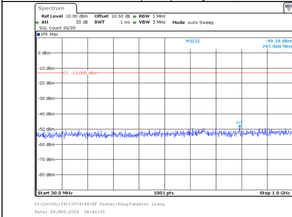
30.0MHz-1000.0MHz Band 66 10MHz/1745.6/Mid 64QAM 1@49 Band 66 20MHz/1760.0/Mid 64QAM 1@0
