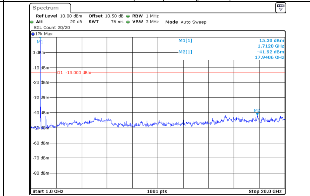
1000.0MHz-20000.0MHz Band 66 5MHz/1713.3/Low 16QAM 25@0 Band 66 20MHz/1725.0/Low 16QAM 100@0
