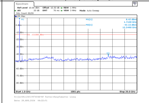
1000.0MHz-20000.0MHz Band 66 5MHz/1713.3/Low 256QAM 25@0 Band 66 20MHz/1725.0/Low 256QAM 100@0
