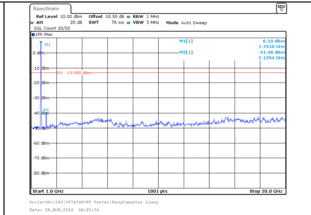
1000.0MHz-20000.0MHz Band 66 20MHz/1720.0/Low QPSK 100@0 Band 66 20MHz/1739.8/Low QPSK 100@0
