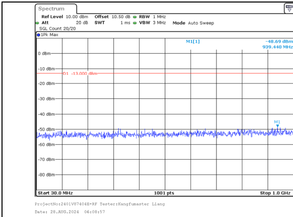
30.0MHz-1000.0MHz Band 66 20MHz/1720.0/Low 64QAM 100@0 Band 66 5MHz/1731.7/Low 64QAM 25@0
