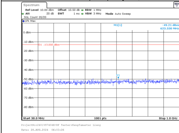
30.0MHz-1000.0MHz Band 66 20MHz/1720.0/Low QPSK 100@0 Band 66 5MHz/1731.7/Low QPSK 25@0
