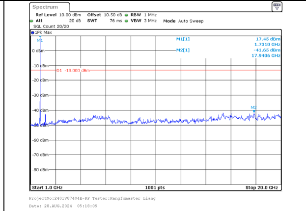
1000.0MHz-20000.0MHz Band 66 20MHz/1720.0/Low QPSK 1@99 Band 66 10MHz/1734.4/Low QPSK 1@0
