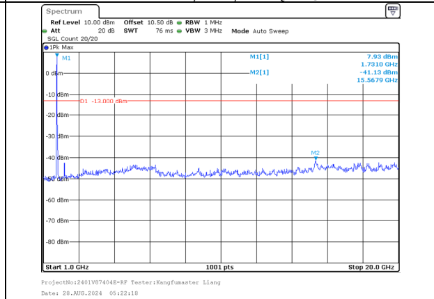
1000.0MHz-20000.0MHz Band 66 20MHz/1720.0/Low 16QAM 100@0 Band 66 10MHz/1734.4/Low 16QAM 100@0
