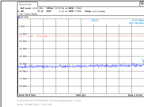
30.0MHz-1000.0MHz Band 66 10MHz/1715.5/Low 16QAM 50@0 Band 66 20MHz/1729.9/Low 16QAM 100@0
