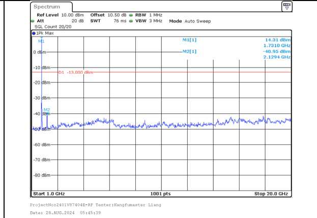
1000.0MHz-20000.0MHz Band 66 15MHz/1717.8/Low 64QAM 1@74 Band 66 20MHz/1734.9/Low 64QAM 1@0
