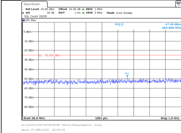
30.0MHz-1000.0MHz Band 41 20MHz/2660.2/High 16QAM 100@0 Band 41 20MHz/2680.0/High 16QAM 100@0
