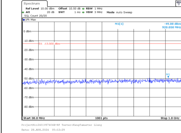
30.0MHz-1000.0MHz Band 66 10MHz/1715.5/Low 64QAM 1@49 Band 66 20MHz/1729.9/Low 64QAM 1@0
