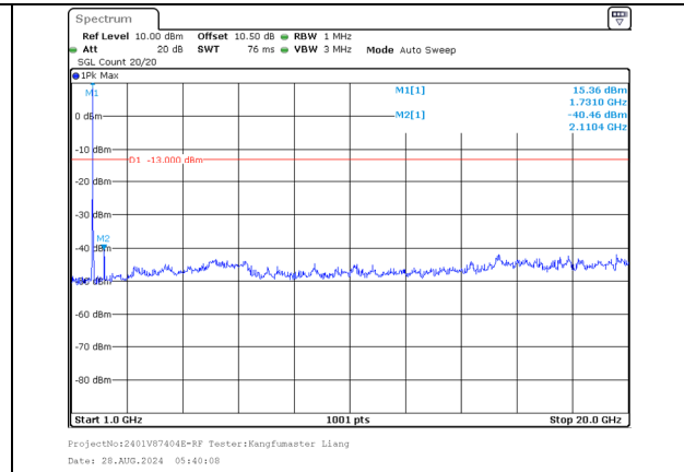
1000.0MHz-20000.0MHz Band 66 15MHz/1717.8/Low QPSK 1@74 Band 66 20MHz/1734.9/Low QPSK 1@0
