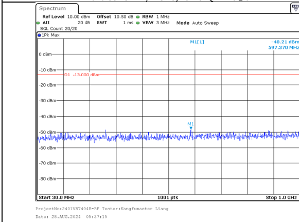
30.0MHz-1000.0MHz Band 66 15MHz/1717.5/Low 256QAM 1@74 Band 66 15MHz/1732.5/Low 256QAM 1@0
