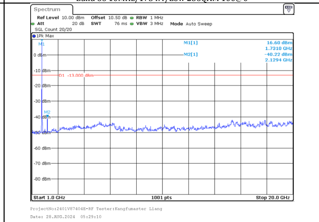
1000.0MHz-20000.0MHz Band 66 15MHz/1717.5/Low QPSK 1@74 Band 66 15MHz/1732.5/Low QPSK 1@0
