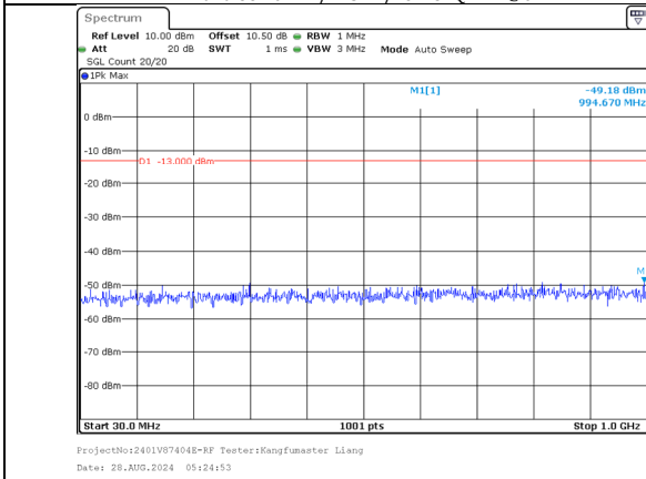
30.0MHz-1000.0MHz Band 66 20MHz/1720.0/Low 64QAM 100@0 Band 66 10MHz/1734.4/Low 64QAM 100@0
