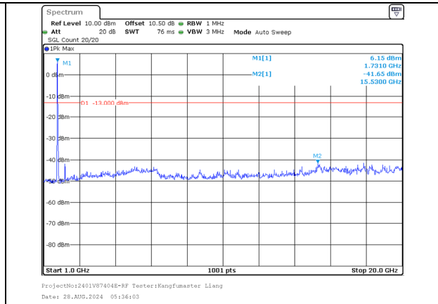
1000.0MHz-20000.0MHz Band 66 15MHz/1717.5/Low 64QAM 75@0 Band 66 15MHz/1732.5/Low 64QAM 75@0
