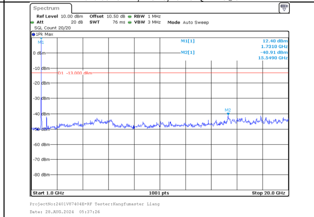
1000.0MHz-20000.0MHz Band 66 15MHz/1717.5/Low 256QAM 1@74 Band 66 15MHz/1732.5/Low 256QAM 1@0
