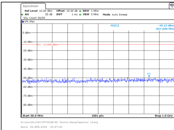
30.0MHz-1000.0MHz Band 66 20MHz/1720.0/Low 256QAM 100@0 Band 66 10MHz/1734.4/Low 256QAM 100@0
