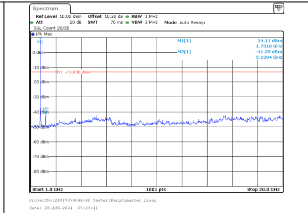
1000.0MHz-20000.0MHz Band 66 20MHz/1720.0/Low 64QAM 1@99 Band 66 10MHz/1734.4/Low 64QAM 1@0
