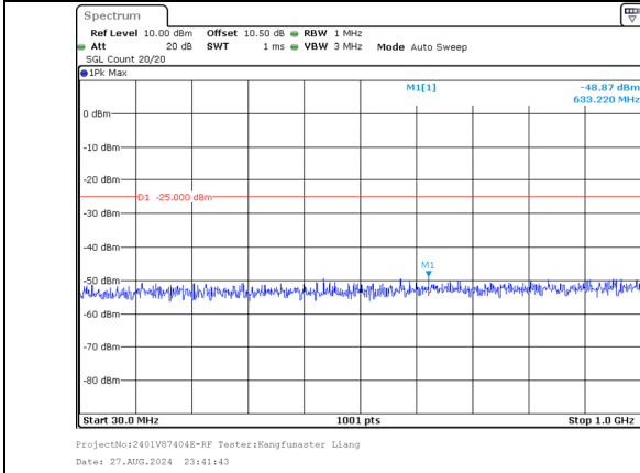
30.0MHz-1000.0MHz Band 41 20MHz/2660.2/High 256QAM 100@0 Band 41 20MHz/2680.0/High 256QAM 100@0
