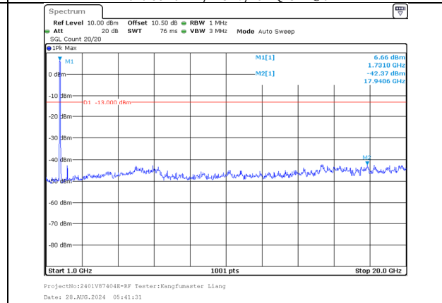
1000.0MHz-20000.0MHz Band 66 15MHz/1717.8/Low QPSK 75@0 Band 66 20MHz/1734.9/Low QPSK 100@0
