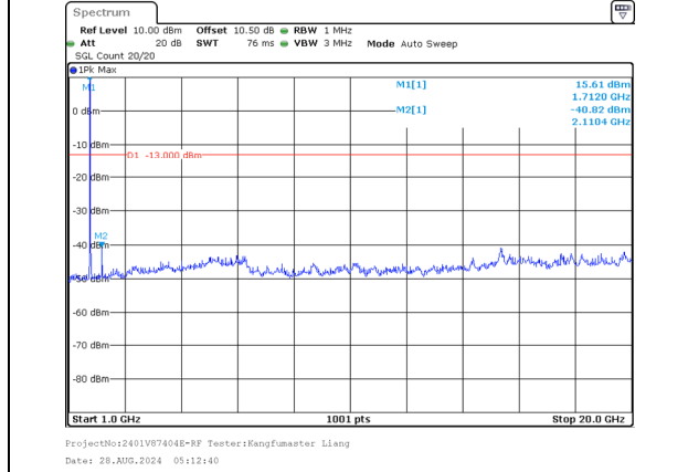
1000.0MHz-20000.0MHz Band 66 10MHz/1715.5/Low 64QAM 1@49 Band 66 20MHz/1729.9/Low 64QAM 1@0
