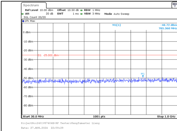
30.0MHz-1000.0MHz Band 41 15MHz/2667.5/High 16QAM 1@74 Band 41 15MHz/2682.5/High 16QAM 1@0
