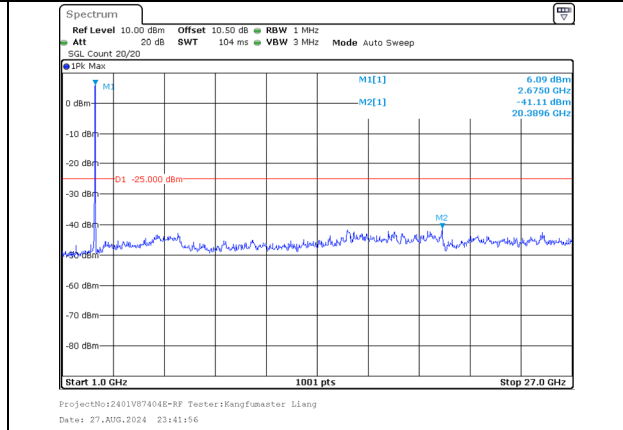
1000.0MHz-27000.0MHz Band 41 20MHz/2660.2/High 256QAM 100@0 Band 41 20MHz/2680.0/High 256QAM 100@0
