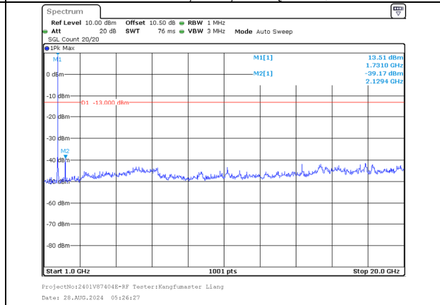
1000.0MHz-20000.0MHz Band 66 20MHz/1720.0/Low 256QAM 1@99 Band 66 10MHz/1734.4/Low 256QAM 1@0
