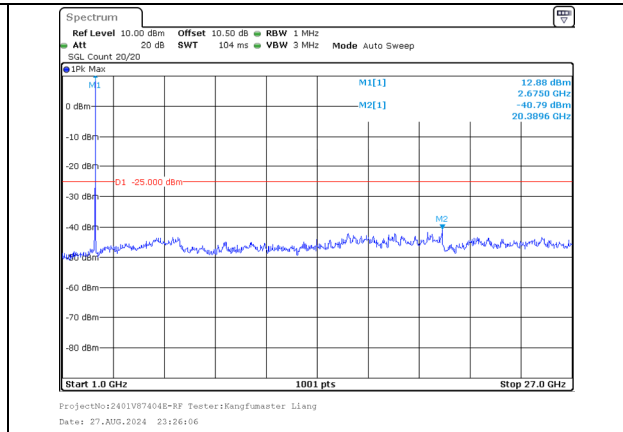
1000.0MHz-27000.0MHz Band 41 20MHz/2665.1/High 64QAM 1@99 Band 41 15MHz/2682.2/High 64QAM 1@0
