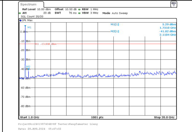
1000.0MHz-20000.0MHz Band 66 15MHz/1717.8/Low 64QAM 75@0 Band 66 20MHz/1734.9/Low 64QAM 100@0
