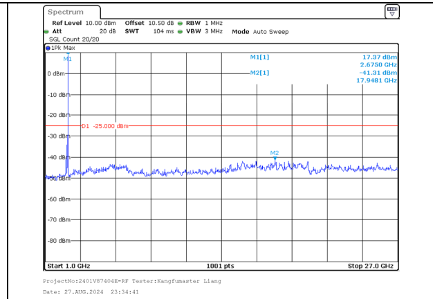
1000.0MHz-27000.0MHz Band 41 20MHz/2660.2/High 16QAM 1@99 Band 41 20MHz/2680.0/High 16QAM 1@0
