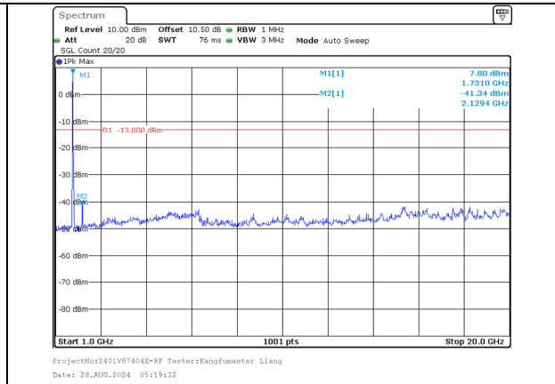
1000.0MHz-20000.0MHz Band 66 20MHz/1720.0/Low QPSK 100@0 Band 66 10MHz/1734.4/Low QPSK 100@0
