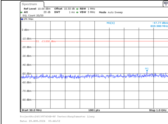
30.0MHz-1000.0MHz Band 66 15MHz/1717.8/Low 64QAM 75@0 Band 66 20MHz/1734.9/Low 64QAM 100@0
