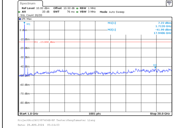
1000.0MHz-20000.0MHz Band 66 10MHz/1715.5/Low 64QAM 50@0 Band 66 20MHz/1729.9/Low 64QAM 100@0
