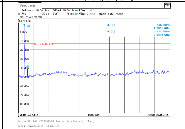
1000.0MHz-20000.0MHz Band 66 15MHz/1717.5/Low QPSK 75@0 Band 66 15MHz/1732.5/Low QPSK 75@0
