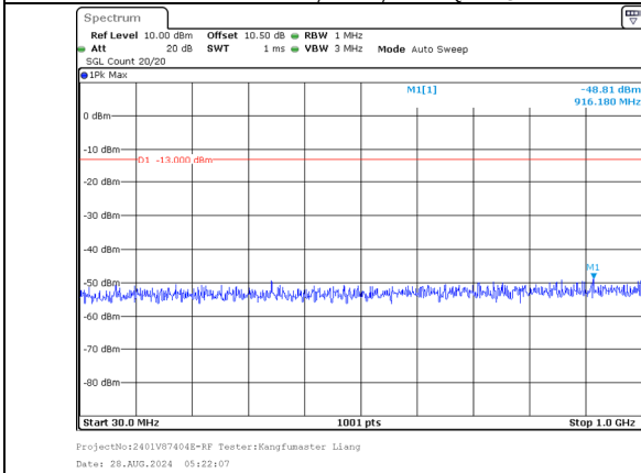
30.0MHz-1000.0MHz Band 66 20MHz/1720.0/Low 16QAM 100@0 Band 66 10MHz/1734.4/Low 16QAM 100@0
