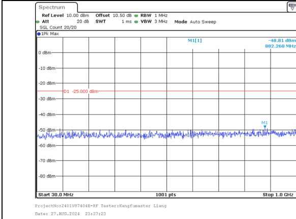
30.0MHz-1000.0MHz Band 41 20MHz/2660.2/High 64QAM 1@99 Band 41 20MHz/2680.0/High 64QAM 1@0
