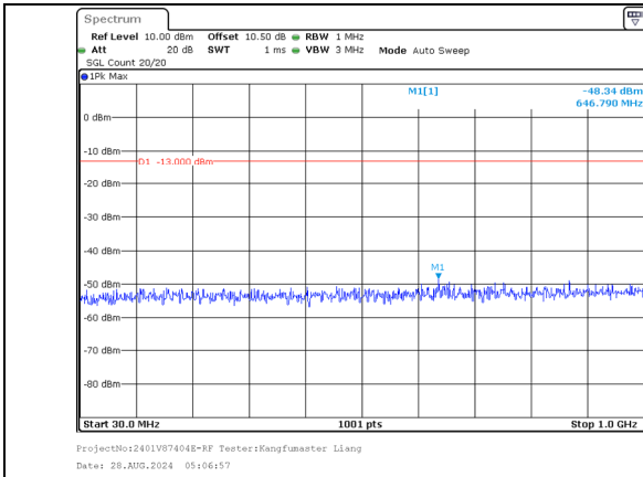
30.0MHz-1000.0MHz Band 66 10MHz/1715.5/Low QPSK 1@49 Band 66 20MHz/1729.9/Low QPSK 1@0
