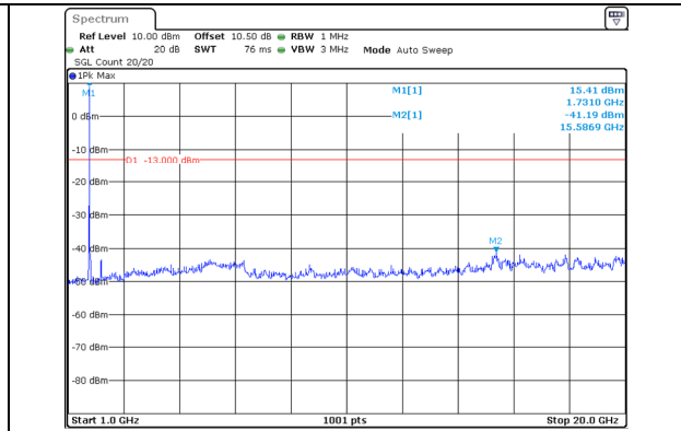
1000.0MHz-20000.0MHz Band 66 15MHz/1717.5/Low 16QAM 1@74 Band 66 15MHz/1732.5/Low 16QAM 1@0
