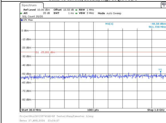
30.0MHz-1000.0MHz Band 41 20MHz/2665.1/High 16QAM 100@0 Band 41 15MHz/2682.2/High 16QAM 100@0
