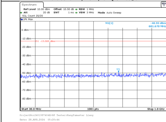
30.0MHz-1000.0MHz Band 66 20MHz/1720.0/Low 16QAM 1@99 Band 66 10MHz/1734.4/Low 16QAM 1@0
