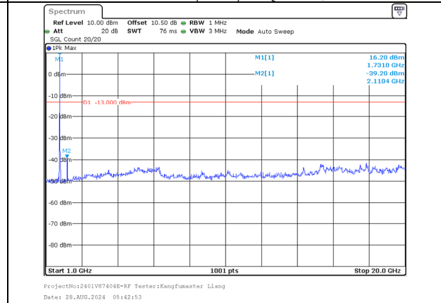
1000.0MHz-20000.0MHz Band 66 15MHz/1717.8/Low 16QAM 1@74 Band 66 20MHz/1734.9/Low 16QAM 1@0
