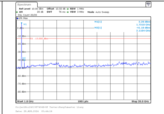
1000.0MHz-20000.0MHz Band 66 15MHz/1717.8/Low 16QAM 75@0 Band 66 20MHz/1734.9/Low 16QAM 100@0
