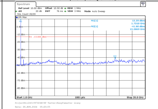
1000.0MHz-20000.0MHz Band 66 20MHz/1720.0/Low 16QAM 1@99 Band 66 10MHz/1734.4/Low 16QAM 1@0
