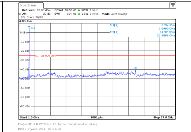
1000.0MHz-27000.0MHz Band 41 20MHz/2660.2/High 64QAM 100@0 Band 41 20MHz/2680.0/High 64QAM 100@0
