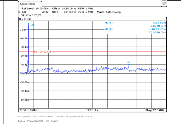
1000.0MHz-27000.0MHz Band 41 20MHz/2660.2/High 16QAM 100@0 Band 41 20MHz/2680.0/High 16QAM 100@0
