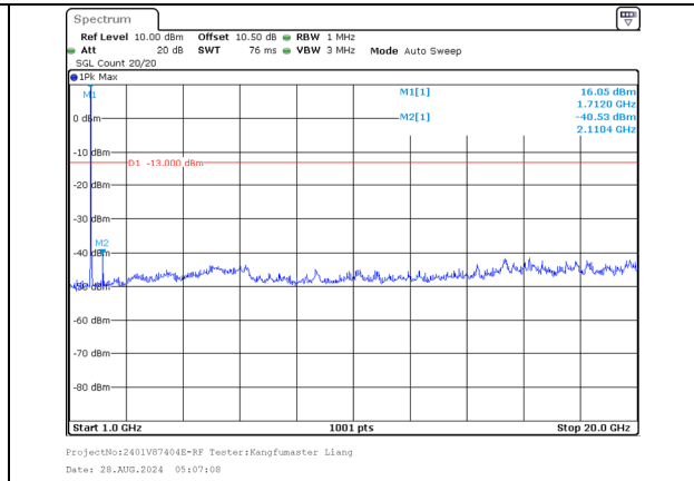
1000.0MHz-20000.0MHz Band 66 10MHz/1715.5/Low QPSK 1@49 Band 66 20MHz/1729.9/Low QPSK 1@0
