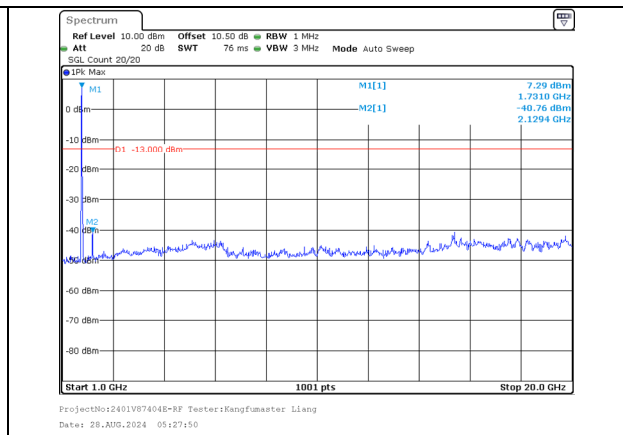
1000.0MHz-20000.0MHz Band 66 20MHz/1720.0/Low 256QAM 100@0 Band 66 10MHz/1734.4/Low 256QAM 100@0
