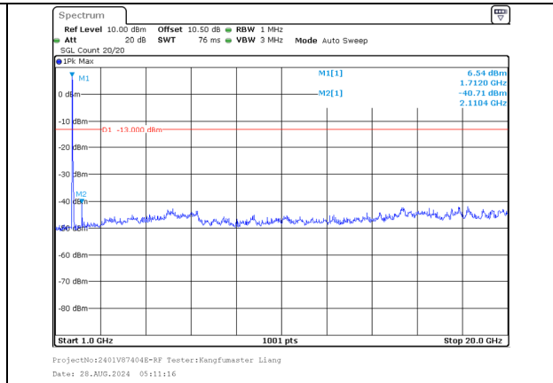
1000.0MHz-20000.0MHz Band 66 10MHz/1715.5/Low 16QAM 50@0 Band 66 20MHz/1729.9/Low 16QAM 100@0
