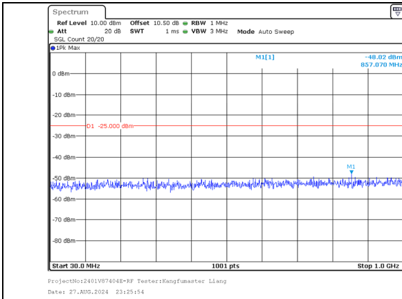
30.0MHz-1000.0MHz Band 41 20MHz/2665.1/High 64QAM 1@99 Band 41 15MHz/2682.2/High 64QAM 1@0
