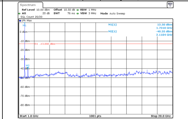
1000.0MHz-20000.0MHz Band 66 15MHz/1717.5/Low 16QAM 75@0 Band 66 15MHz/1732.5/Low 16QAM 75@0
