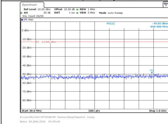
30.0MHz-1000.0MHz Band 66 10MHz/1715.5/Low 16QAM 1@49 Band 66 20MHz/1729.9/Low 16QAM 1@0
