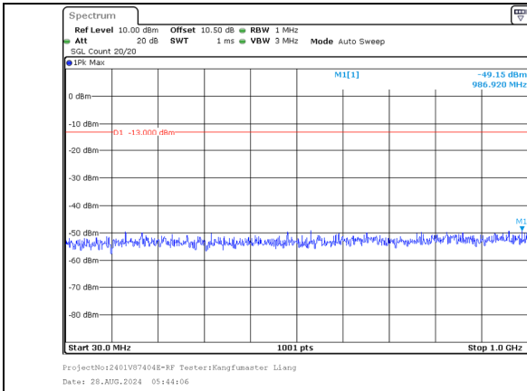
30.0MHz-1000.0MHz Band 66 15MHz/1717.8/Low 16QAM 75@0 Band 66 20MHz/1734.9/Low 16QAM 100@0
