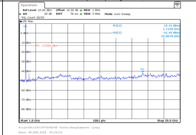
1000.0MHz-20000.0MHz Band 66 10MHz/1715.5/Low 16QAM 1@49 Band 66 20MHz/1729.9/Low 16QAM 1@0
