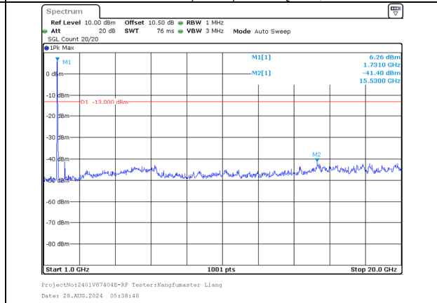
1000.0MHz-20000.0MHz Band 66 15MHz/1717.5/Low 256QAM 75@0 Band 66 15MHz/1732.5/Low 256QAM 75@0
