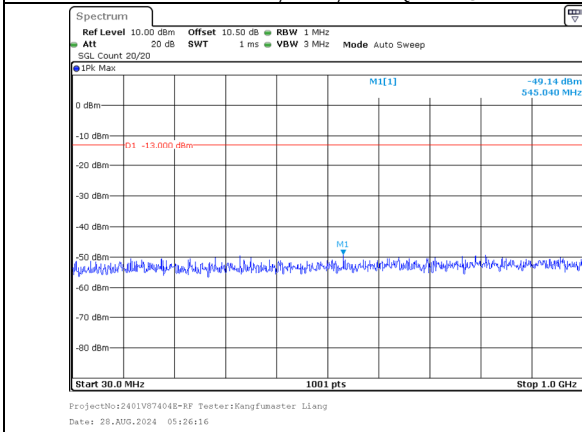
30.0MHz-1000.0MHz Band 66 20MHz/1720.0/Low 256QAM 1@99 Band 66 10MHz/1734.4/Low 256QAM 1@0
