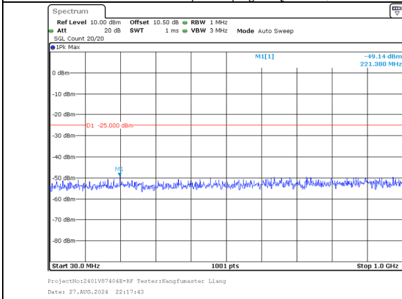
30.0MHz-1000.0MHz Band 41 5MHz/2668.3/High 256QAM 1@24 Band 41 20MHz/2680.0/High 256QAM 1@0
