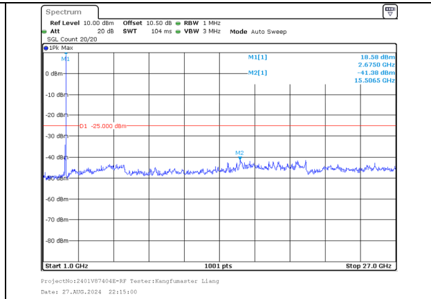
1000.0MHz-27000.0MHz Band 41 5MHz/2668.3/High 64QAM 1@24 Band 41 20MHz/2680.0/High 64QAM 1@0
