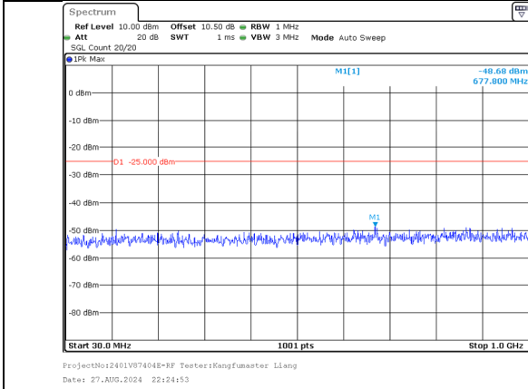
30.0MHz-1000.0MHz Band 41 20MHz/2675.0/High 16QAM 100@0 Band 41 5MHz/2686.7/High 16QAM 25@0
