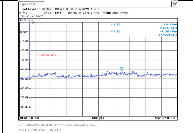
1000.0MHz-27000.0MHz Band 41 20MHz/2675.0/High 16QAM 100@0 Band 41 5MHz/2686.7/High 16QAM 25@0
