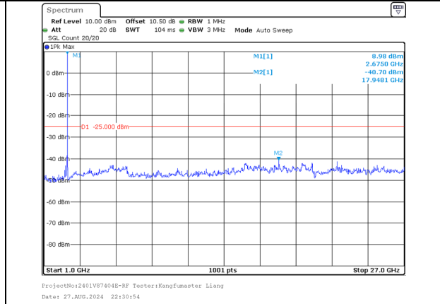
1000.0MHz-27000.0MHz Band 41 20MHz/2675.0/High 256QAM 100@0 Band 41 5MHz/2686.7/High 256QAM 25@0
