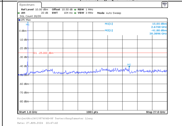
1000.0MHz-27000.0MHz Band 41 20MHz/2670.1/High 16QAM 1@99 Band 41 10MHz/2684.5/High 16QAM 1@0
