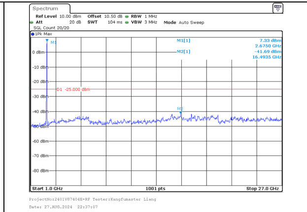
1000.0MHz-27000.0MHz Band 41 10MHz/2665.6/High 16QAM 50@0 Band 41 20MHz/2680.0/High 16QAM 100@0
