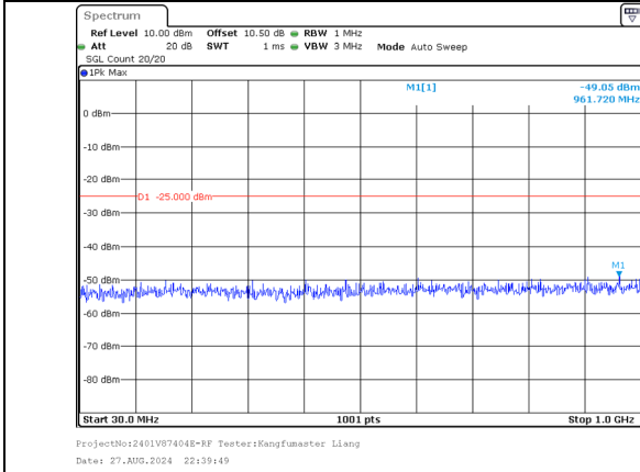
30.0MHz-1000.0MHz Band 41 10MHz/2665.6/High 64QAM 50@0 Band 41 20MHz/2680.0/High 64QAM 100@0
