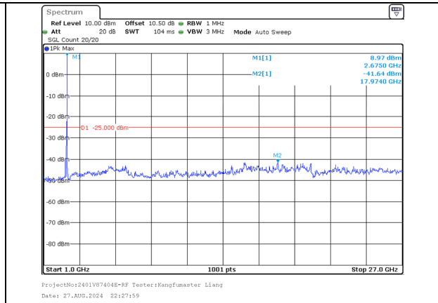
1000.0MHz-27000.0MHz Band 41 20MHz/2675.0/High 64QAM 100@0 Band 41 5MHz/2686.7/High 64QAM 25@0
