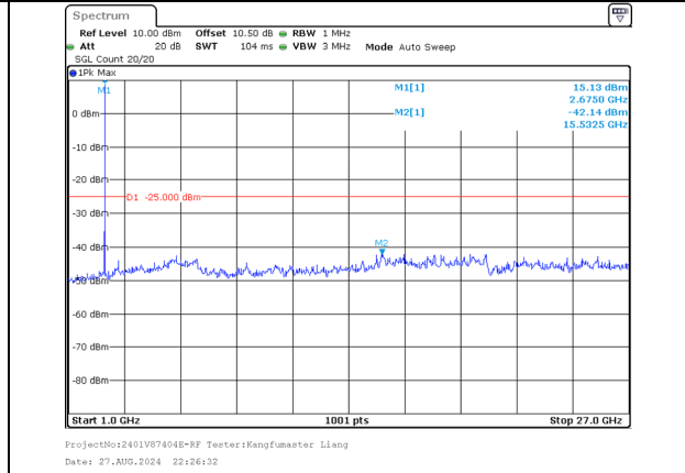
1000.0MHz-27000.0MHz Band 41 20MHz/2675.0/High 64QAM 1@99 Band 41 5MHz/2686.7/High 64QAM 1@0
