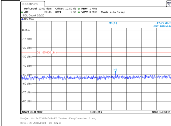
30.0MHz-1000.0MHz Band 41 10MHz/2665.6/High 256QAM 50@0 Band 41 20MHz/2680.0/High 256QAM 100@0
