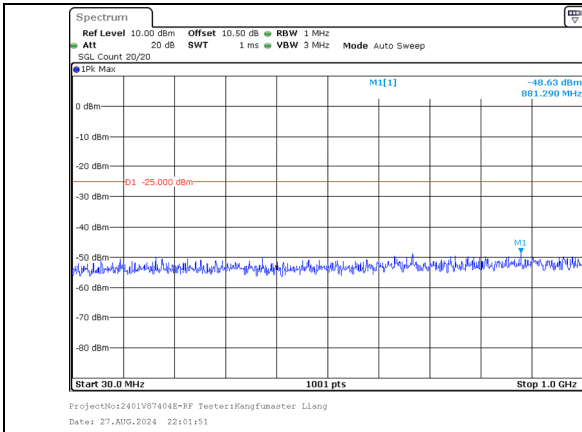
30.0MHz-1000.0MHz Band 41 20MHz/2583.1/Mid 16QAM 100@0 Band 41 20MHz/2602.9/Mid 16QAM 100@0
