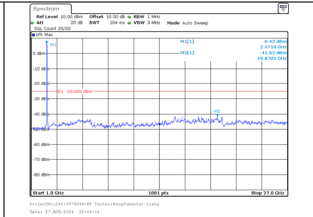
1000.0MHz-27000.0MHz Band 41 20MHz/2583.1/Mid 16QAM 100@0 Band 41 20MHz/2602.9/Mid 16QAM 100@0
