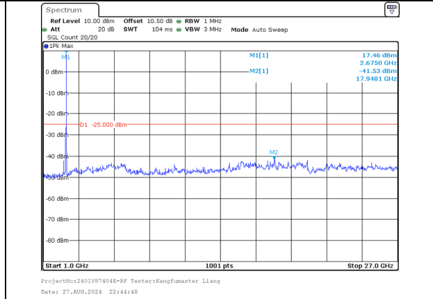
1000.0MHz-27000.0MHz Band 41 20MHz/2670.1/High QPSK 1@99 Band 41 10MHz/2684.5/High QPSK 1@0
