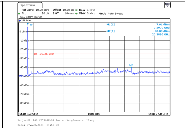
1000.0MHz-27000.0MHz Band 41 20MHz/2585.6/Mid 64QAM 100@0 Band 41 15MHz/2602.7/Mid 64QAM 100@0
