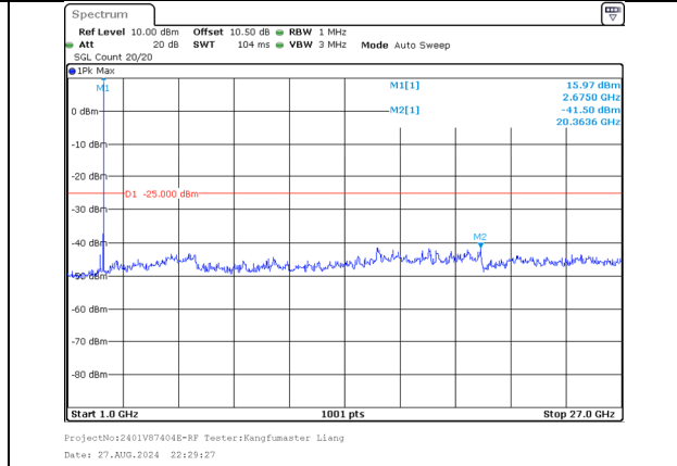
1000.0MHz-27000.0MHz Band 41 20MHz/2675.0/High 256QAM 1@99 Band 41 5MHz/2686.7/High 256QAM 1@0
