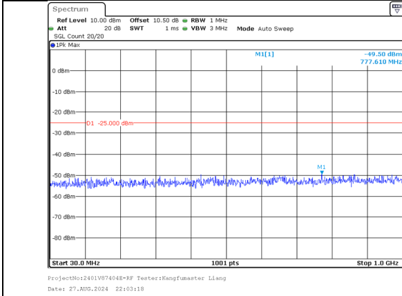
30.0MHz-1000.0MHz Band 41 20MHz/2583.1/Mid 64QAM 1@99 Band 41 20MHz/2602.9/Mid 64QAM 1@0
