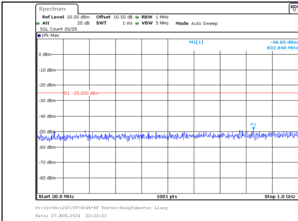
30.0MHz-1000.0MHz Band 41 10MHz/2665.6/High QPSK 1@49 Band 41 20MHz/2680.0/High QPSK 1@0
