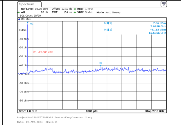
1000.0MHz-27000.0MHz Band 41 10MHz/2665.6/High 64QAM 50@0 Band 41 20MHz/2680.0/High 64QAM 100@0
