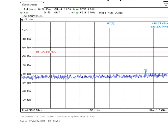
30.0MHz-1000.0MHz Band 41 20MHz/2670.1/High 16QAM 100@0 Band 41 10MHz/2684.5/High 16QAM 100@0
