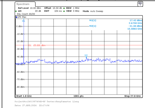
1000.0MHz-27000.0MHz Band 41 5MHz/2668.3/High 256QAM 1@24 Band 41 20MHz/2680.0/High 256QAM 1@0
