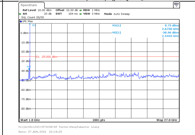
1000.0MHz-27000.0MHz Band 41 5MHz/2668.3/High 64QAM 25@0 Band 41 20MHz/2680.0/High 64QAM 100@0
