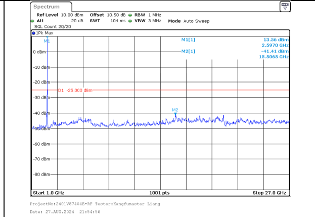
1000.0MHz-27000.0MHz Band 41 20MHz/2585.6/Mid 256QAM 1@99 Band 41 15MHz/2602.7/Mid 256QAM 1@0
