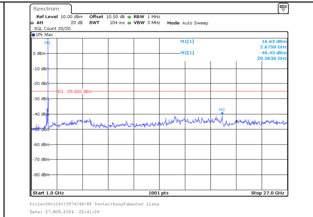
1000.0MHz-27000.0MHz Band 41 10MHz/2665.6/High 256QAM 1@49 Band 41 20MHz/2680.0/High 256QAM 1@0
