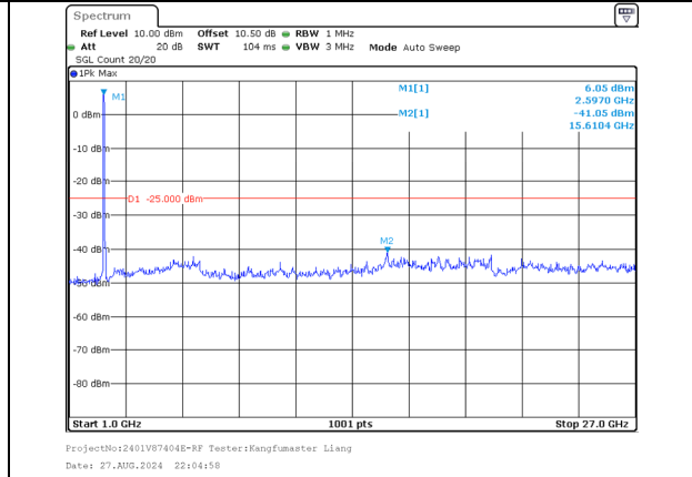
1000.0MHz-27000.0MHz Band 41 20MHz/2583.1/Mid 64QAM 100@0 Band 41 20MHz/2602.9/Mid 64QAM 100@0
