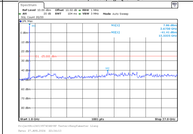
1000.0MHz-27000.0MHz Band 41 10MHz/2665.6/High QPSK 50@0 Band 41 20MHz/2680.0/High QPSK 100@0
