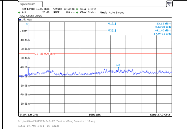
1000.0MHz-27000.0MHz Band 41 20MHz/2583.1/Mid 64QAM 1@99 Band 41 20MHz/2602.9/Mid 64QAM 1@0
