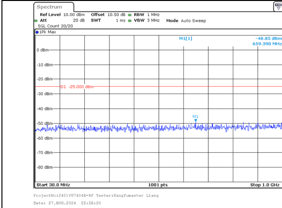
30.0MHz-1000.0MHz Band 41 20MHz/2675.0/High 64QAM 1@99 Band 41 5MHz/2686.7/High 64QAM 1@0
