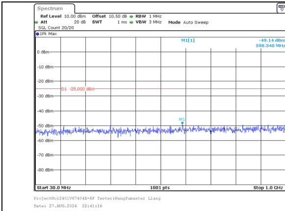
30.0MHz-1000.0MHz Band 41 10MHz/2665.6/High 256QAM 1@49 Band 41 20MHz/2680.0/High 256QAM 1@0
