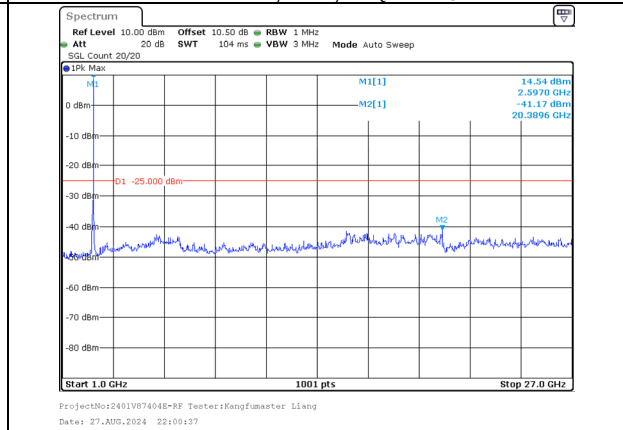
1000.0MHz-27000.0MHz Band 41 20MHz/2583.1/Mid 16QAM 1@99 Band 41 20MHz/2602.9/Mid 16QAM 1@0
