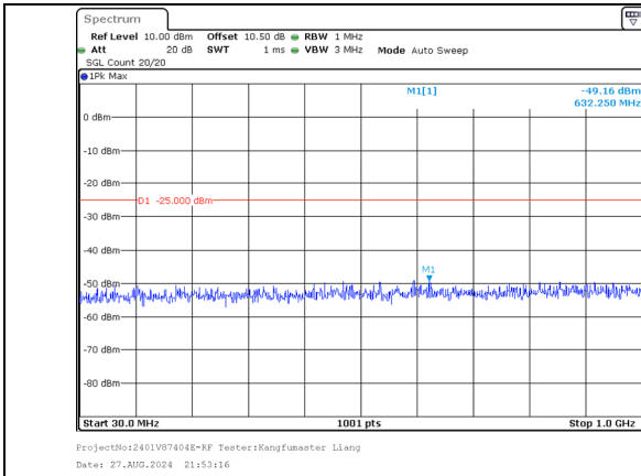
30.0MHz-1000.0MHz Band 41 20MHz/2585.6/Mid 64QAM 100@0 Band 41 15MHz/2602.7/Mid 64QAM 100@0
