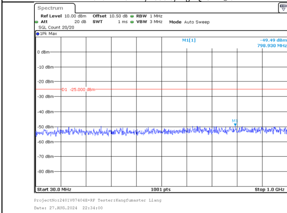
30.0MHz-1000.0MHz Band 41 10MHz/2665.6/High QPSK 50@0 Band 41 20MHz/2680.0/High QPSK 100@0
