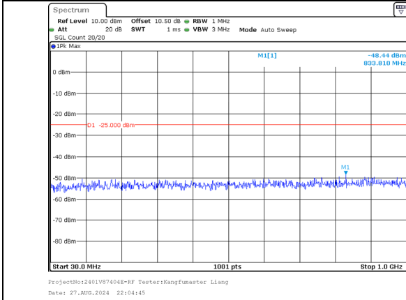
30.0MHz-1000.0MHz Band 41 20MHz/2583.1/Mid 64QAM 100@0 Band 41 20MHz/2602.9/Mid 64QAM 100@0
