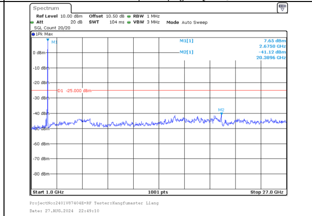
1000.0MHz-27000.0MHz Band 41 20MHz/2670.1/High 16QAM 100@0 Band 41 10MHz/2684.5/High 16QAM 100@0
