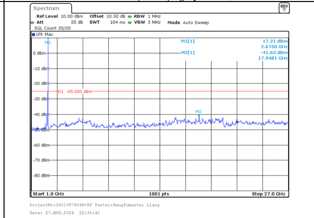
1000.0MHz-27000.0MHz Band 41 10MHz/2665.6/High 16QAM 1@49 Band 41 20MHz/2680.0/High 16QAM 1@0
