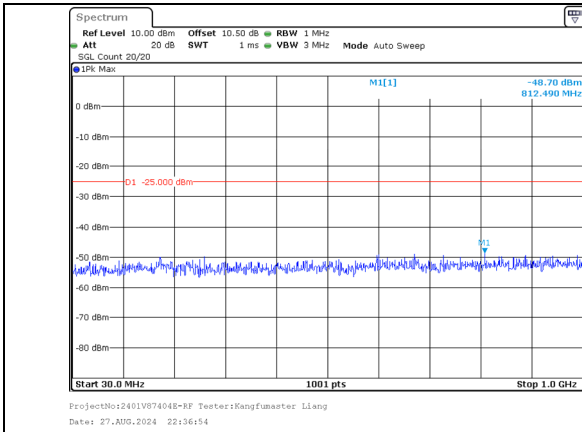
30.0MHz-1000.0MHz Band 41 10MHz/2665.6/High 16QAM 50@0 Band 41 20MHz/2680.0/High 16QAM 100@0
