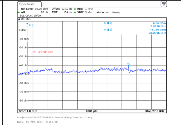
1000.0MHz-27000.0MHz Band 41 20MHz/2585.6/Mid 256QAM 100@0 Band 41 15MHz/2602.7/Mid 256QAM 100@0
