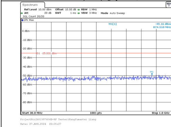
30.0MHz-1000.0MHz Band 41 10MHz/2665.6/High 16QAM 1@49 Band 41 20MHz/2680.0/High 16QAM 1@0
