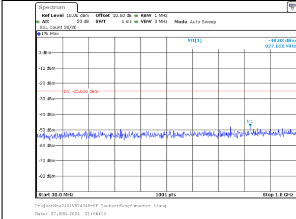
30.0MHz-1000.0MHz Band 41 20MHz/2585.6/Mid 256QAM 100@0 Band 41 15MHz/2602.7/Mid 256QAM 100@0
