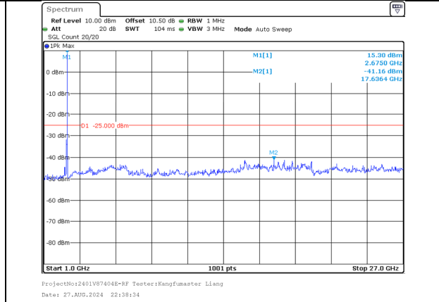
1000.0MHz-27000.0MHz Band 41 10MHz/2665.6/High 64QAM 1@49 Band 41 20MHz/2680.0/High 64QAM 1@0
