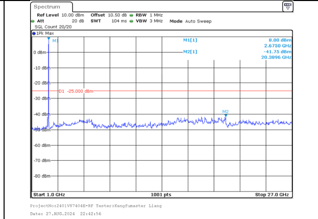
1000.0MHz-27000.0MHz Band 41 10MHz/2665.6/High 256QAM 50@0 Band 41 20MHz/2680.0/High 256QAM 100@0
