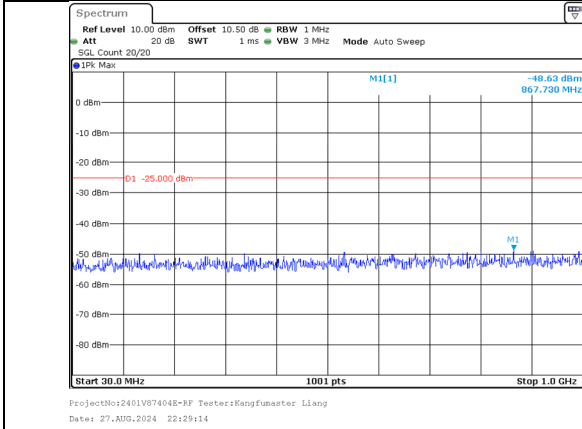
30.0MHz-1000.0MHz Band 41 20MHz/2675.0/High 256QAM 1@99 Band 41 5MHz/2686.7/High 256QAM 1@0
