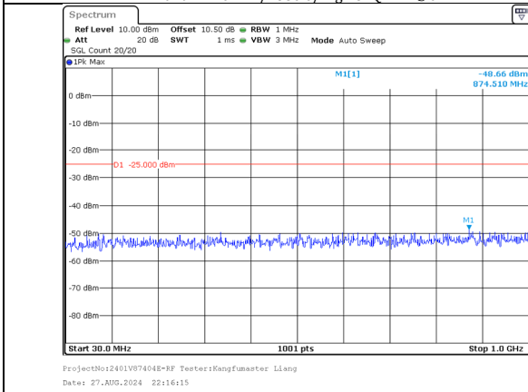
30.0MHz-1000.0MHz Band 41 5MHz/2668.3/High 64QAM 25@0 Band 41 20MHz/2680.0/High 64QAM 100@0
