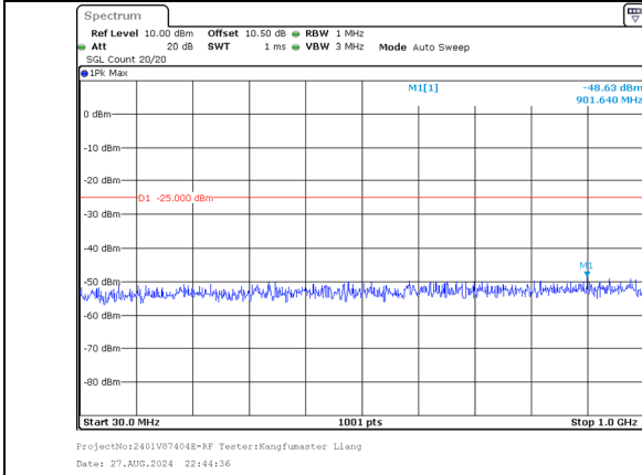
30.0MHz-1000.0MHz Band 41 20MHz/2670.1/High QPSK 1@99 Band 41 10MHz/2684.5/High QPSK 1@0
