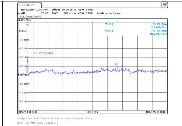
1000.0MHz-27000.0MHz Band 41 10MHz/2665.6/High QPSK 1@49 Band 41 20MHz/2680.0/High QPSK 1@0
