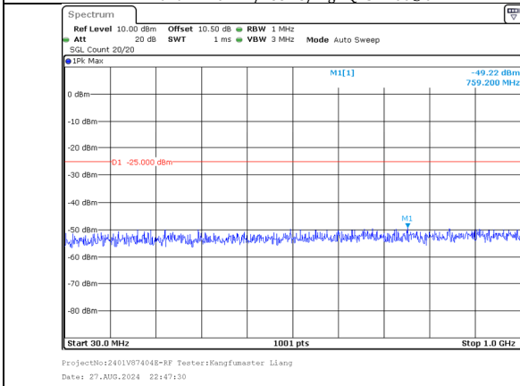
30.0MHz-1000.0MHz Band 41 20MHz/2670.1/High 16QAM 1@99 Band 41 10MHz/2684.5/High 16QAM 1@0
