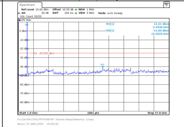
1000.0MHz-27000.0MHz Band 41 10MHz/2501.5/Low 64QAM 1@49 Band 41 20MHz/2515.9/Low 64QAM 1@0
