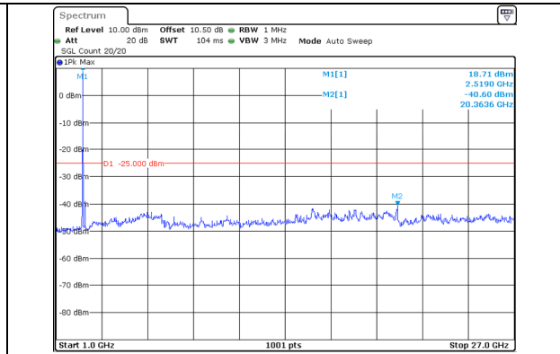
1000.0MHz-27000.0MHz Band 41 20MHz/2506.0/Low QPSK 1@99 Band 41 10MHz/2520.4/Low QPSK 1@0
