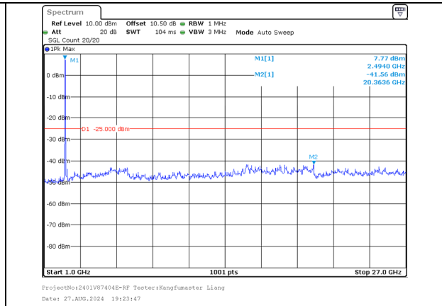
1000.0MHz-27000.0MHz Band 41 10MHz/2501.5/Low 64QAM 50@0 Band 41 20MHz/2515.9/Low 64QAM 100@0
