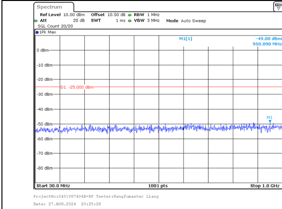
30.0MHz-1000.0MHz Band 41 20MHz/2506.0/Low QPSK 1@99 Band 41 20MHz/2525.8/Low QPSK 1@0
