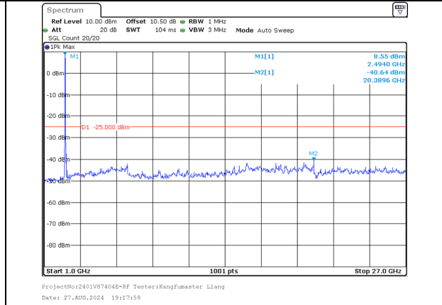
1000.0MHz-27000.0MHz Band 41 10MHz/2501.5/Low QPSK 50@0 Band 41 20MHz/2515.9/Low QPSK 100@0
