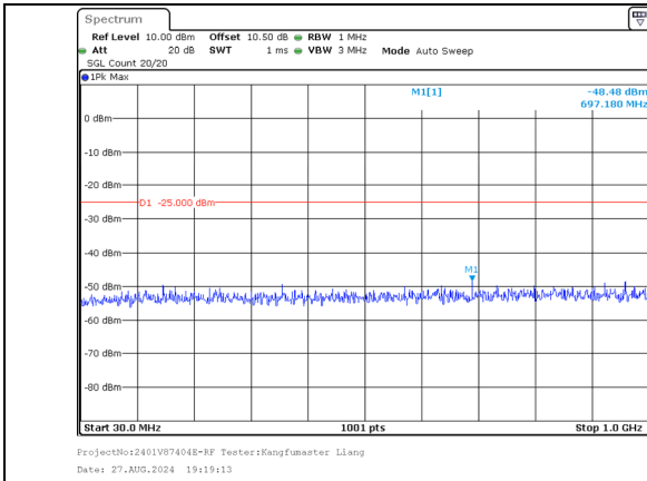
30.0MHz-1000.0MHz Band 41 10MHz/2501.5/Low 16QAM 1@49 Band 41 20MHz/2515.9/Low 16QAM 1@0
