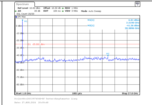
1000.0MHz-27000.0MHz Band 41 15MHz/2503.8/Low 64QAM 75@0 Band 41 20MHz/2520.9/Low 64QAM 100@0
