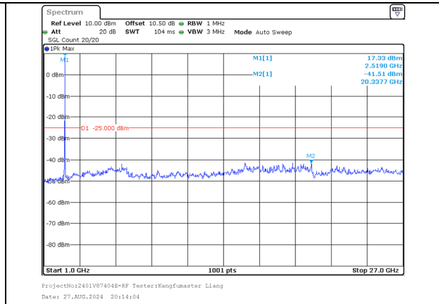
1000.0MHz-27000.0MHz Band 41 20MHz/2506.0/Low QPSK 1@99 Band 41 15MHz/2523.1/Low QPSK 1@0
