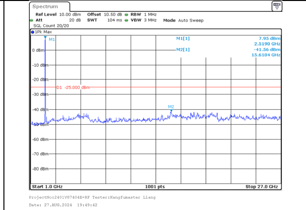
1000.0MHz-27000.0MHz Band 41 20MHz/2506.0/Low 256QAM 100@0 Band 41 10MHz/2520.4/Low 256QAM 100@0
