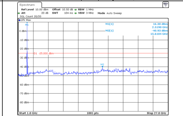
1000.0MHz-27000.0MHz Band 41 20MHz/2506.0/Low QPSK 100@0 Band 41 10MHz/2520.4/Low QPSK 100@0
