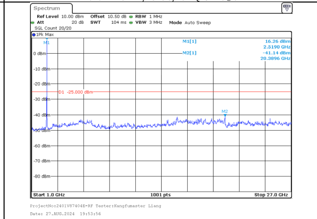
1000.0MHz-27000.0MHz Band 41 15MHz/2503.5/Low 16QAM 1@74 Band 41 15MHz/2518.5/Low 16QAM 1@0
