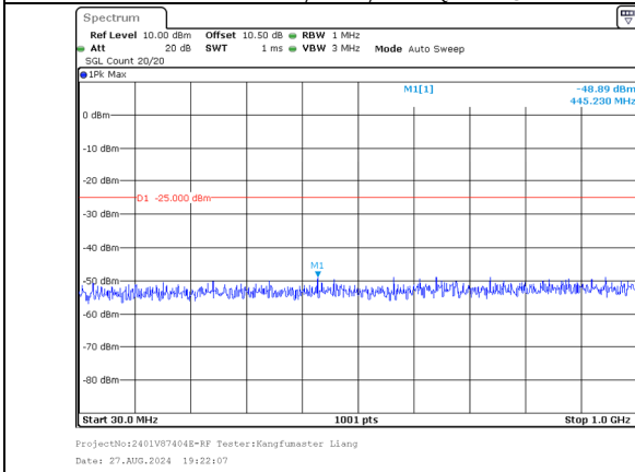
30.0MHz-1000.0MHz Band 41 10MHz/2501.5/Low 64QAM 1@49 Band 41 20MHz/2515.9/Low 64QAM 1@0
