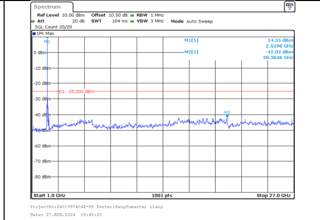
1000.0MHz-27000.0MHz Band 41 20MHz/2506.0/Low 64QAM 1@99 Band 41 10MHz/2520.4/Low 64QAM 1@0
