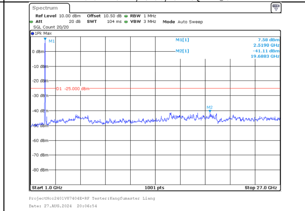
1000.0MHz-27000.0MHz Band 41 15MHz/2503.8/Low 16QAM 75@0 Band 41 20MHz/2520.9/Low 16QAM 100@0
