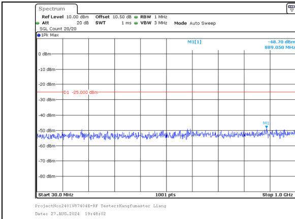
30.0MHz-1000.0MHz Band 41 20MHz/2506.0/Low 256QAM 1@99 Band 41 10MHz/2520.4/Low 256QAM 1@0
