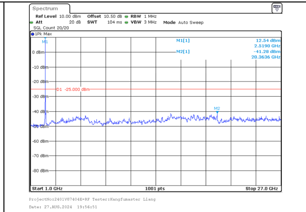
1000.0MHz-27000.0MHz Band 41 15MHz/2503.5/Low 64QAM 1@74 Band 41 15MHz/2518.5/Low 64QAM 1@0
