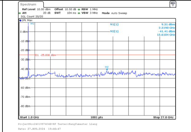
1000.0MHz-27000.0MHz Band 41 20MHz/2506.0/Low 64QAM 100@0 Band 41 10MHz/2520.4/Low 64QAM 100@0
