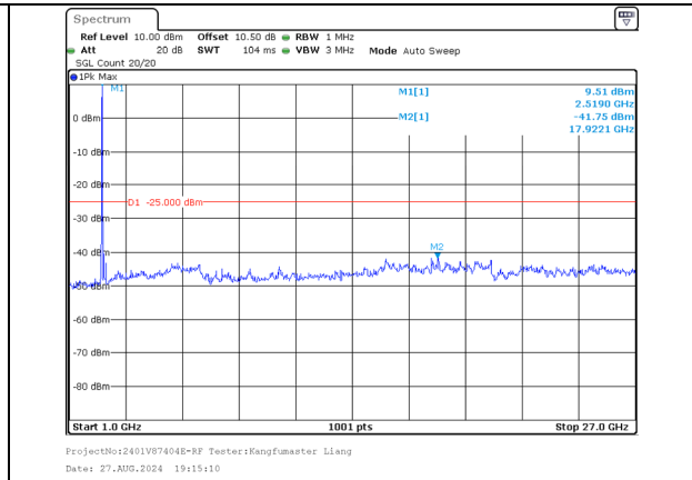
1000.0MHz-27000.0MHz Band 41 20MHz/2506.0/Low 256QAM 100@0 Band 41 5MHz/2517.7/Low 256QAM 25@0
