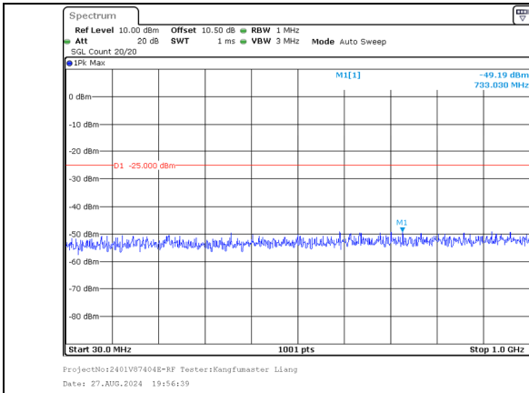
30.0MHz-1000.0MHz Band 41 15MHz/2503.5/Low 64QAM 1@74 Band 41 15MHz/2518.5/Low 64QAM 1@0
