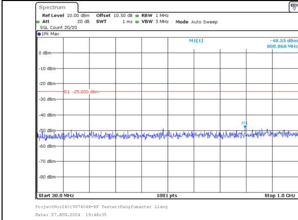
30.0MHz-1000.0MHz Band 41 20MHz/2506.0/Low 64QAM 100@0 Band 41 10MHz/2520.4/Low 64QAM 100@0
