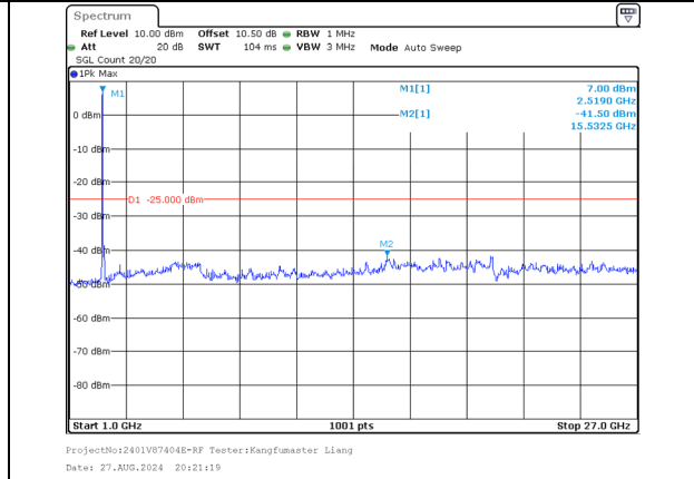
1000.0MHz-27000.0MHz Band 41 20MHz/2506.0/Low 64QAM 100@0 Band 41 15MHz/2523.1/Low 64QAM 100@0
