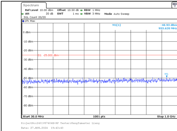
30.0MHz-1000.0MHz Band 41 20MHz/2506.0/Low 16QAM 100@0 Band 41 10MHz/2520.4/Low 16QAM 100@0
