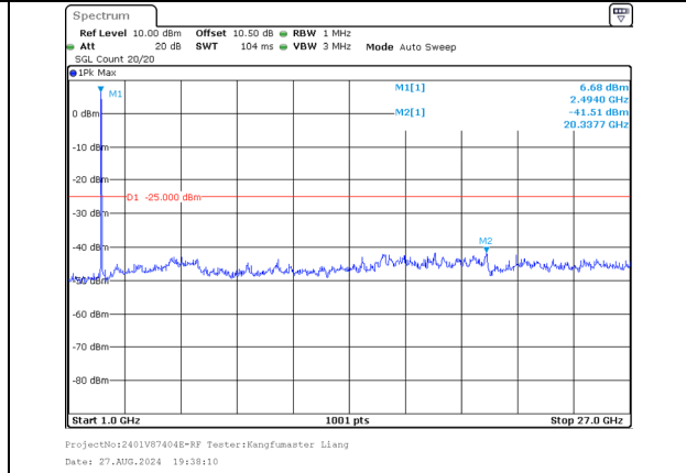
1000.0MHz-27000.0MHz Band 41 10MHz/2501.5/Low 256QAM 50@0 Band 41 20MHz/2515.9/Low 256QAM 100@0
