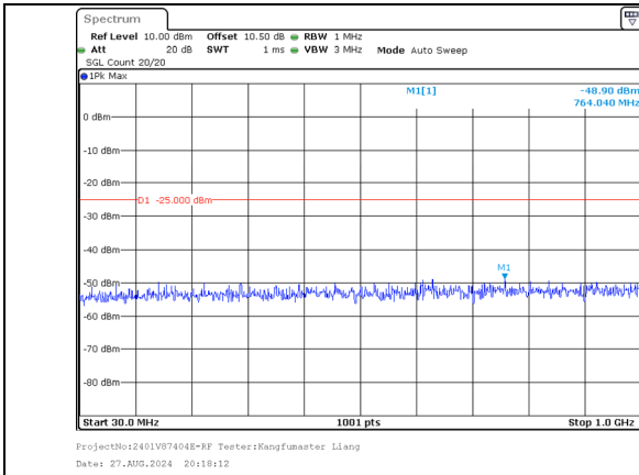
30.0MHz-1000.0MHz Band 41 20MHz/2506.0/Low 16QAM 100@0 Band 41 15MHz/2523.1/Low 16QAM 100@0
