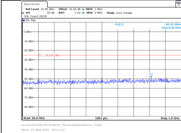
30.0MHz-1000.0MHz Band 41 15MHz/2503.8/Low 256QAM 1@74 Band 41 20MHz/2520.9/Low 256QAM 1@0
