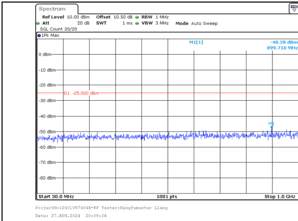
30.0MHz-1000.0MHz Band 41 15MHz/2503.8/Low 64QAM 75@0 Band 41 20MHz/2520.9/Low 64QAM 100@0
