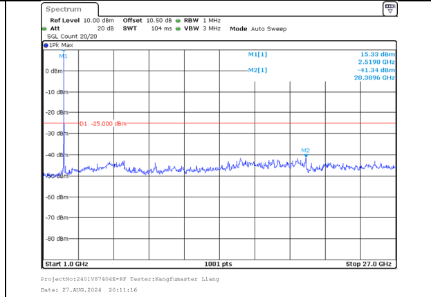
1000.0MHz-27000.0MHz Band 41 15MHz/2503.8/Low 256QAM 1@74 Band 41 20MHz/2520.9/Low 256QAM 1@0
