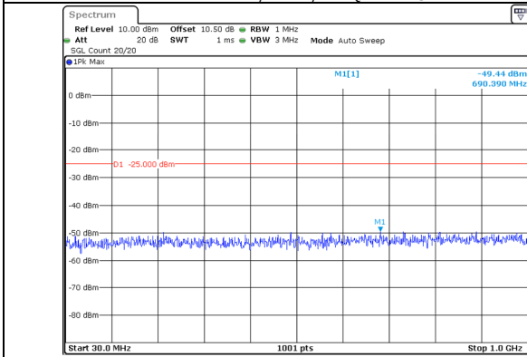
30.0MHz-1000.0MHz Band 41 20MHz/2506.0/Low QPSK 100@0 Band 41 10MHz/2520.4/Low QPSK 100@0
