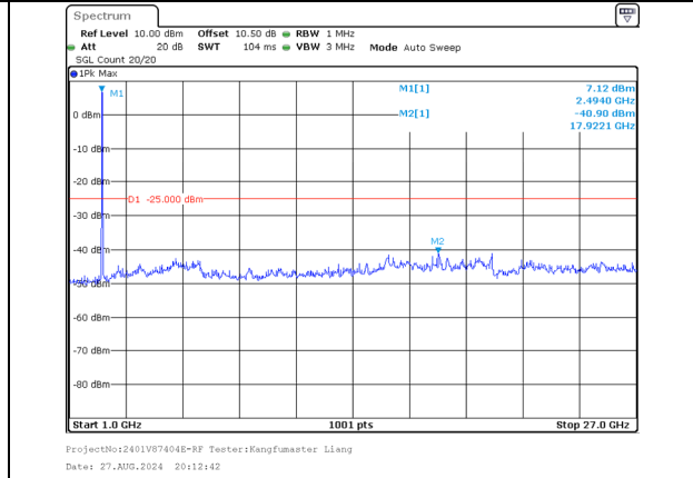
1000.0MHz-27000.0MHz Band 41 15MHz/2503.8/Low 256QAM 75@0 Band 41 20MHz/2520.9/Low 256QAM 100@0
