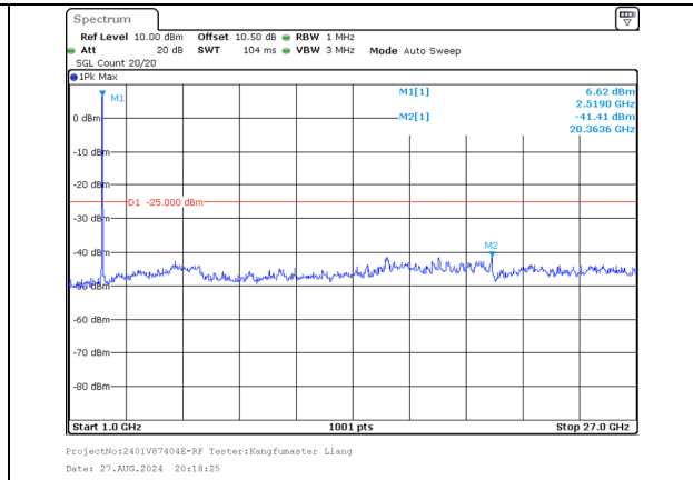
1000.0MHz-27000.0MHz Band 41 20MHz/2506.0/Low 16QAM 100@0 Band 41 15MHz/2523.1/Low 16QAM 100@0
