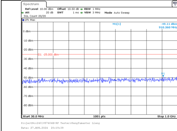
30.0MHz-1000.0MHz Band 41 20MHz/2506.0/Low 64QAM 1@99 Band 41 15MHz/2523.1/Low 64QAM 1@0
