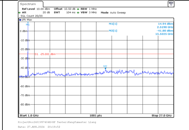
1000.0MHz-27000.0MHz Band 41 20MHz/2506.0/Low 64QAM 1@99 Band 41 15MHz/2523.1/Low 64QAM 1@0
