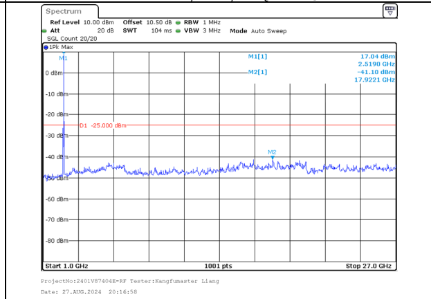
1000.0MHz-27000.0MHz Band 41 20MHz/2506.0/Low 16QAM 1@99 Band 41 15MHz/2523.1/Low 16QAM 1@0
