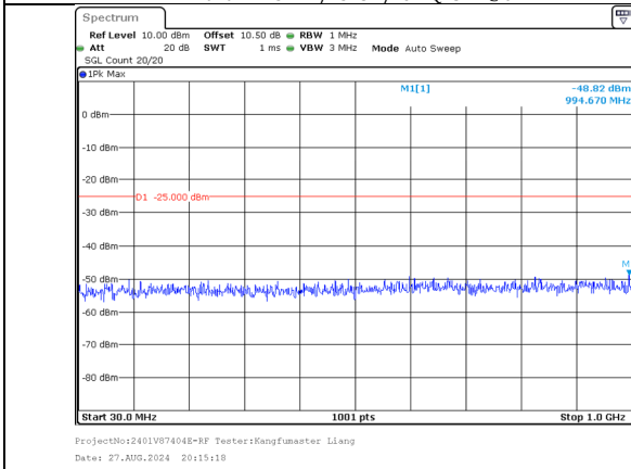
30.0MHz-1000.0MHz Band 41 20MHz/2506.0/Low QPSK 100@0 Band 41 15MHz/2523.1/Low QPSK 100@0
