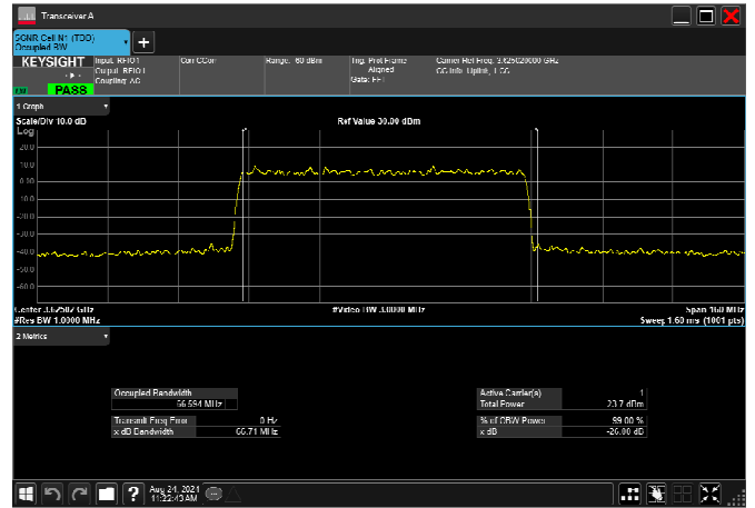
n78_2_70MHz_30kHz_3625MHz_DFT-s-OFDM 64 QAM_RB180@0 66.375MHz
