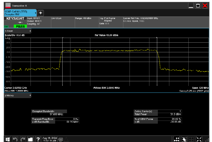
n78_2_60MHz_30kHz_3625MHz_DFT-s-OFDM 16 QAM_RB162@0 57.480MHz
