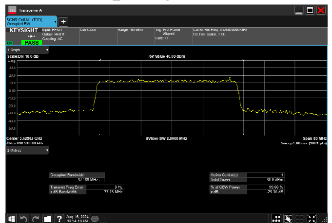
n78_2_40MHz_30kHz_3625MHz_DFT-s-OFDM 16 QAM_RB100@0 37.186MHz
