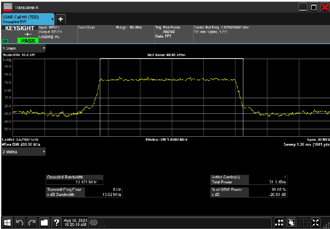
n78_2_15MHz_30kHz_3625MHz_DFT-s-OFDM 16 QAM_RB36@0 13.467MHz
