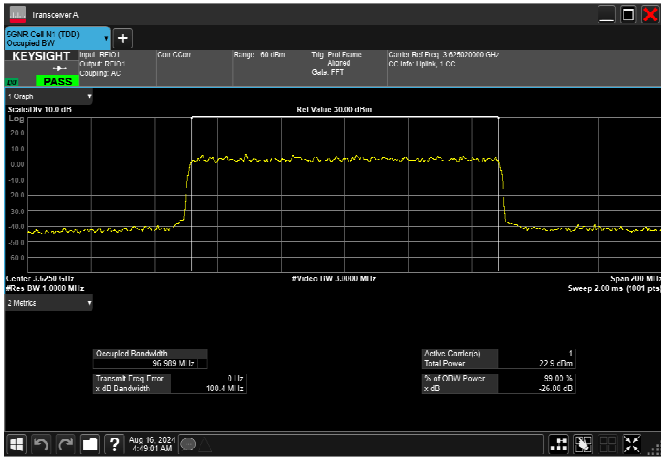
n77_2_100MHz_30kHz_3625MHz_CP-OFDM 16 QAM_RB273@0 96.989MHz
