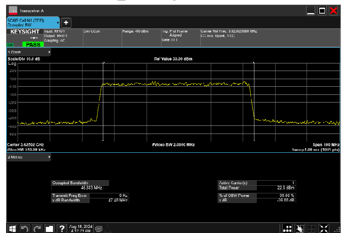
n77_2_50MHz_30kHz_3625MHz_DFT-s-OFDM 16 QAM_RB128@0 46.883MHz
