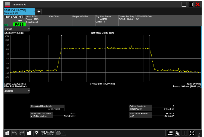
n77_2_30MHz_30kHz_3625MHz_CP-OFDM 256 QAM_RB78@0 27.760MHz
