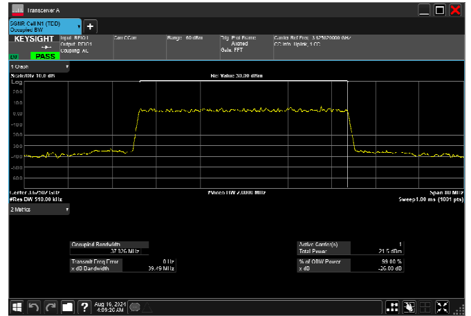
n77_2_50MHz_30kHz_3625MHz_DFT-s-OFDM \pi/2 BPSK_RB128@0 46.854MHz
