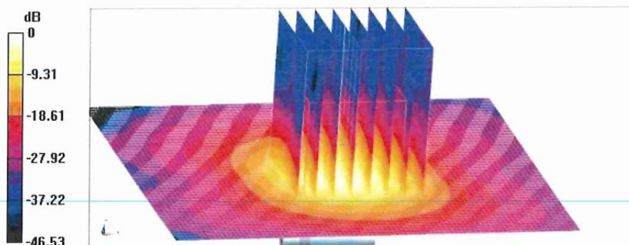
0 dB = 19.8 W/kg = 12.97 dBW/kg
