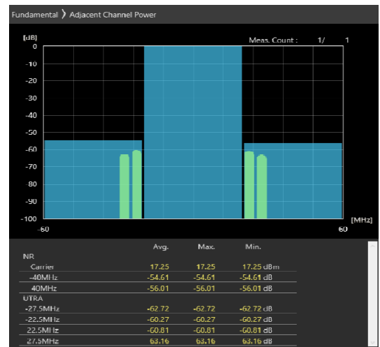
40MHz_30kHz_3680MHz-OFDM QPSK_RB50@25 -54.61,-56.01dB
